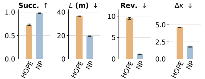
Fig. 3. NeuralParker improves success rate and trajectory quality over the adapted HOPE planner on the Factorial Parking Benchmark. Success uses all 1080 episodes per seed; trajectory metrics use the pairwise common-success cohort ( n = 773/748/790 ). Bars and error bars show the three-seed mean \pm sample SD. NP denotes NeuralParker.
