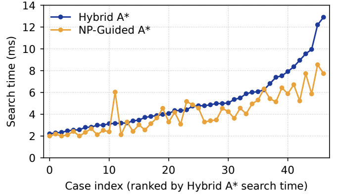
Fig. 8. Learned guidance reduces Hybrid A* search time mostly on the harder real-vehicle clips. The 47 held-out clips are ordered by Hybrid A* search time, which serves as a difficulty proxy, and both planners' times are shown in that order.
