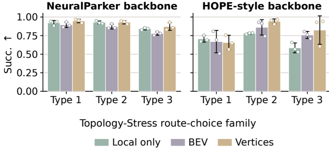
Fig. 5. Absolute family-level success rates show that representation effects depend on route-choice family and policy backbone on the Topology-Stress Benchmark. Each family contains 240 episodes per seed. Every group compares local-only, BEV, and vertices; bars and error bars show the three-seed mean \pm sample SD, and open circles show individual seeds.
