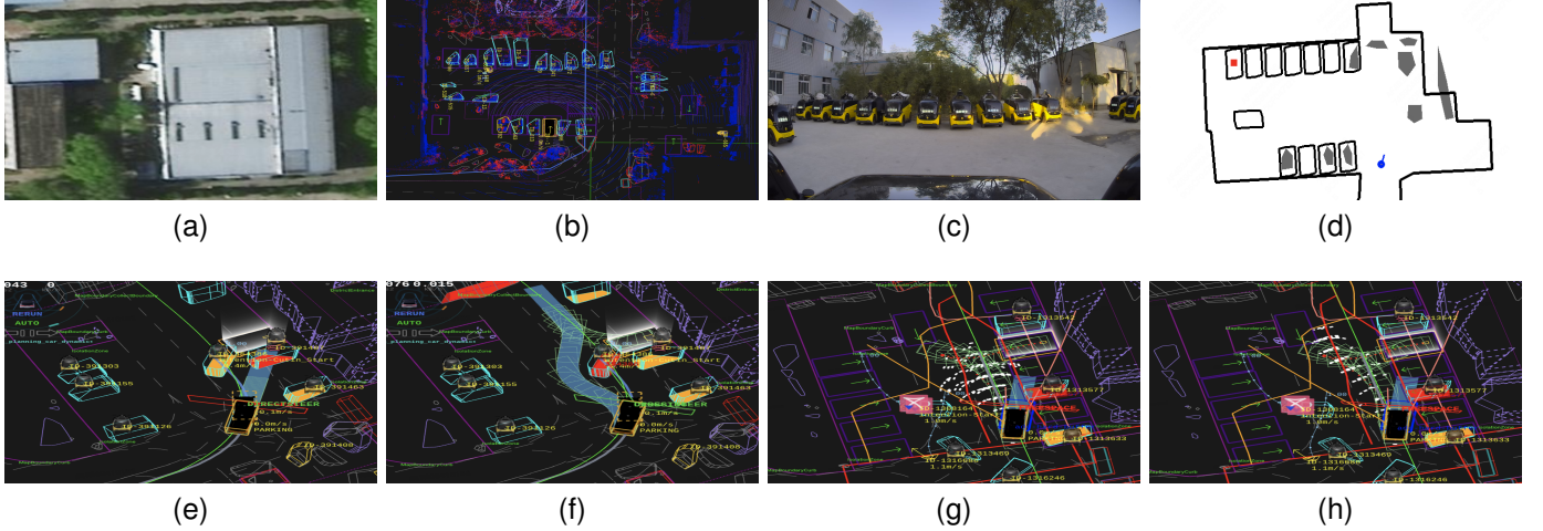
Fig. 7. Real-vehicle experiments with a simpler NeuralParker configuration. (a)–(d) operating site, perception visualization, camera view, and site-specific simulation reconstruction; (e)–(h) two simulation-validated cases comparing Hybrid A* with NeuralParker-Guided A*.
