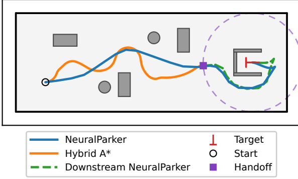
Fig. 4. Unified planning keeps one approach decision where a staged handoff splits it. Each planner is drawn as one line, so the staged arm’s arcs and terminal connector share the dashed green line. One checkpoint drives both learned arms on this pinned pocket case; the dashed circle is the 10 m handoff boundary.
