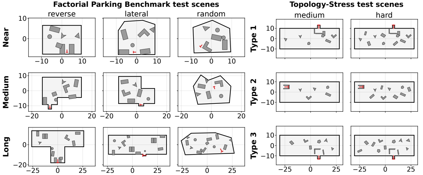
Fig. 2. Representative held-out scenes from the Factorial Parking Benchmark (left) and the Topology-Stress Benchmark (right). The Factorial block arranges start-separation regimes by row and target-pose types by column; the Topology-Stress block arranges route-choice families by row and difficulty by column. All panels preserve equal x - y metric scaling. Red T markers denote target poses and headings, and axes are in meters.
