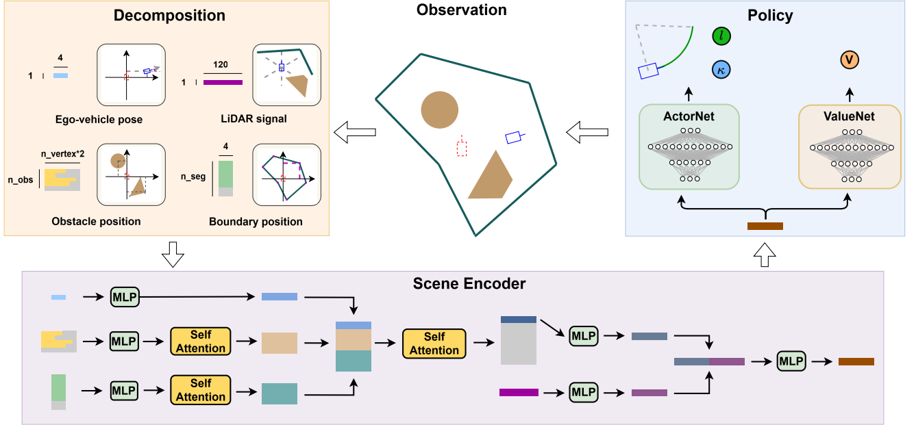
Fig. 1. Overview of the NeuralParker architecture. The observation is decomposed into the ego pose, obstacle vertices, boundary segments, and local LiDAR signals. The scene encoder embeds the four streams, uses self-attention to aggregate the obstacle and boundary tokens, and fuses the resulting global geometry with the ego and LiDAR features. The shared representation is passed to the actor and critic networks, which output the curvature-length arc ( \kappa, l ) and the state-value estimate, respectively.
