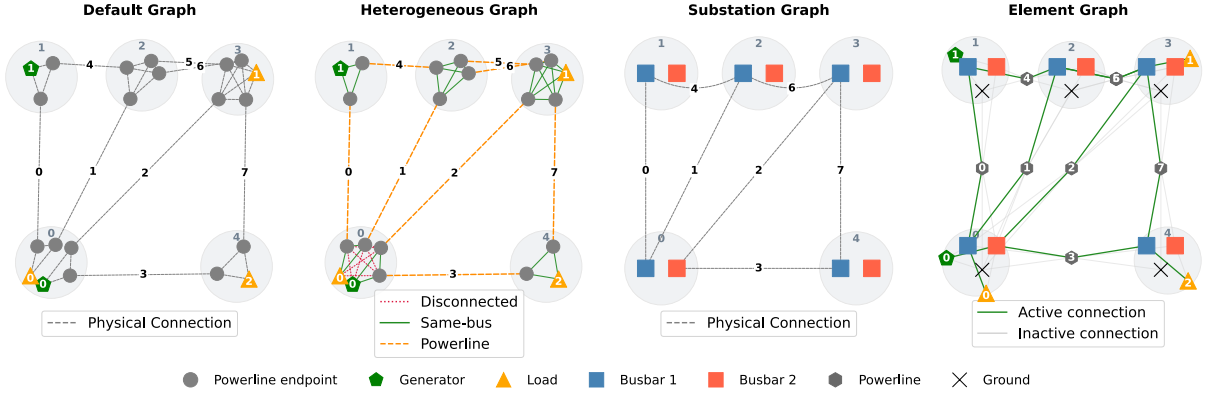
Fig. 1: Topology based representations of the rte_case5_example environment with 5 substations (0-4). Each panel depicts the same grid configuration. All elements are assigned to Busbar 1 except at substation 0 (bottom left), where several elements are assigned to Busbar 2.
