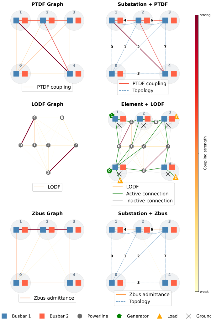
Fig. 2: Power-Flow-Based (left) and Hybrid (right) representations of the rte_case5_example environment.
