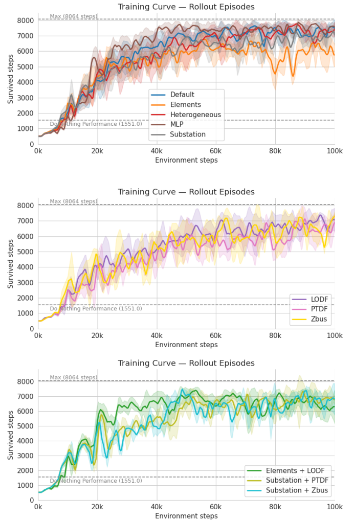
Fig. 3: Rollout survival during training for the topology-based graph and the MLP baseline (top), powerflow-based graphs (middle), and hybrid graphs (bottom).
