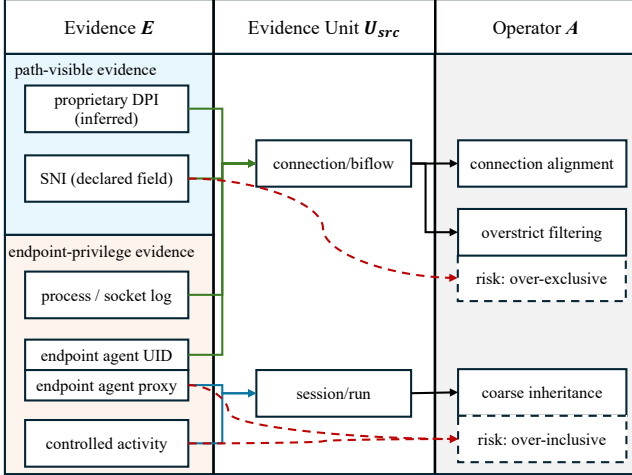
Figure 2: How label evidence reaches published flows in the 14 audited entries. Evidence (left, grouped by layer \Lambda ) holds at an evidence unit U_{\text{source}} (middle) and reaches published samples through an assignment operator A (right). Connection alignment is the non-failing counterpart; coarse inheritance risks over-inclusion; overstrict filtering risks over-exclusion by keying on a flow’s own path-visible identifier, bypassing the unit constraint.
