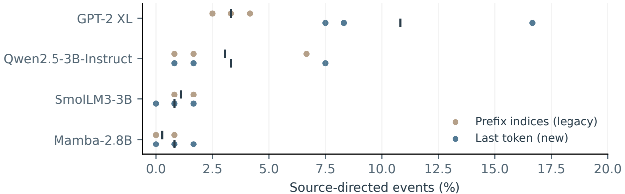
Figure 11: Token-position protocol changes the measured intervention effect. FARS source-directed event rates for the legacy prefix and last-token protocols. Dots represent seeds; horizontal marks represent seed means. Shared concept pairs make these repeated observations. A position change is not a test of semantic correctness.
