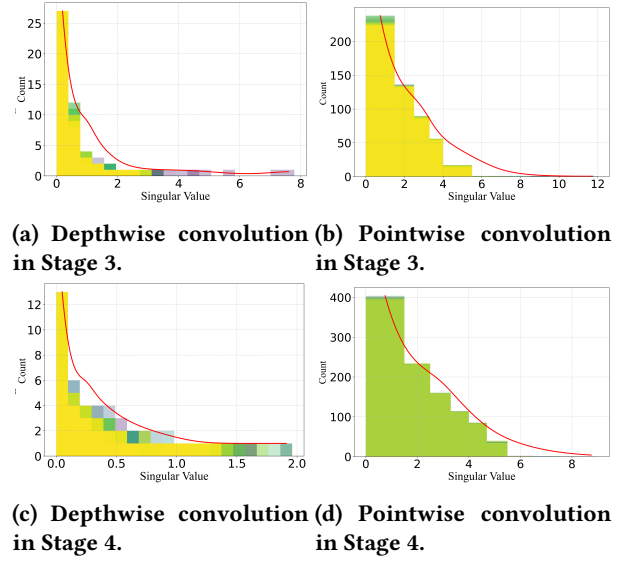
Figure 6: Singular value distributions of pointwise and depthwise convolutional kernels in pre-trained RepLKNet-31B (Stages 3-4) after channel grouping. Each subfigure aggregates the kernel matrices grouped by stage and convolution type, with individual matrices color-coded. X-axis: Singular values; Y-axis: Count of singular values within defined bounds.
