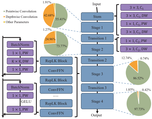
Figure 2: Parameter distribution across stages in pre-trained RepLkNet-31B: pie charts quantify the proportion of parameters from pointwise convolutions, depthwise convolutions, and other components within each stage.
