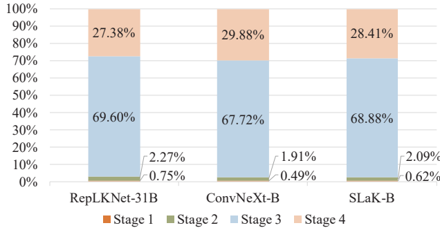
Figure 3: Stage-wise parameter distribution across Stages 1–4 in pre-trained RepLkNet-31B, ConvNeXt-B, and SLaK-B models: each bar quantifies the proportion of parameters from individual stages relative to the total model parameters.
