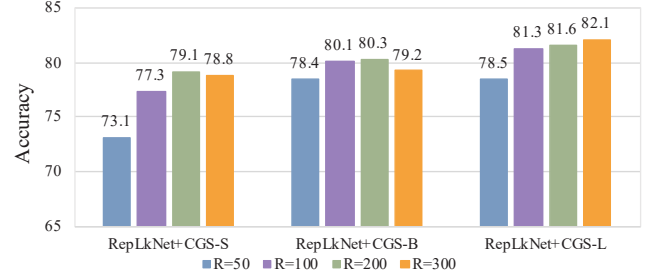
Figure 8: Systematic evaluation of dimensionality scaling effects in down/up-projection matrices on CGS performance for CIFAR-100 datasets. Detailed results are presented in Appendix B.
