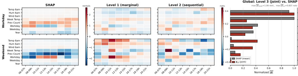
Figure D.3: Local SHAP vs. Entropy-Shapley attributions for the workday and weekend test instances (left, centre) and global aggregation over the full test set (right). SHAP attributes the predicted mean \hat{\mu}_t(\mathbf{x}) in rentals, while Level 1 ( \phi_H^{(t)} ) and Level 2 ( \phi_H^{(t|<t)} ) attribute the marginal and sequentially conditional predictive entropy in nats, respectively. The right panel compares the mean of |\phi_H^{\text{joint}}| across the test set with the corresponding mean absolute SHAP values, each min-max normalized within its method. This highlights how feature effects on the mean and uncertainty are naturally decoupled: for instance, Workday strongly drives point prediction but not the joint (daily) uncertainty, whereas the opposite is true for Hum. 6am and Temp. 6am.
