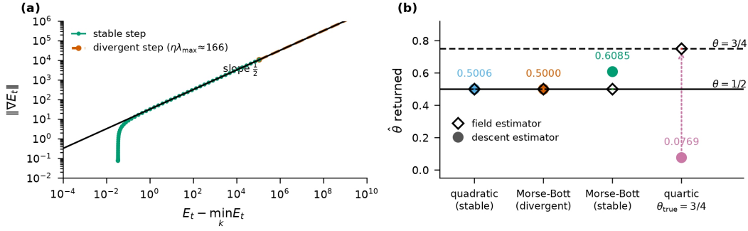
Figure 3: The descent-based Łojasiewicz estimator is uninformative by construction (Remark 11). (a) For a quadratic energy the log-log locus is the line of slope \frac{1}{2} over ten decades whether the iteration converges or diverges; the two traces coincide with the theorem line. (b) What the estimator returns on analytic energies of known exponent: \frac{1}{2} on quadratic and Morse-Bott energies including under a divergent step, a different value under a stable step on the same energy, and 0.077 on a quartic energy whose true exponent is \frac{3}{4} (dotted arrow to the truth). Open diamonds: the field estimator of (13) on the same energies, which returns the true exponent in all four cases.
