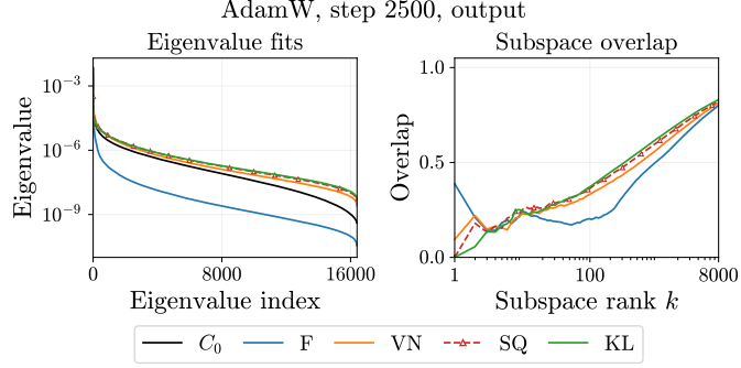
Figure 5: Large-sample Kronecker fits. Left: empirical and fitted eigenvalues. Right: overlap of the leading subspaces. The fitted spectra and eigenspaces follow the divergence-dependent preferences predicted in Section 3.2.
