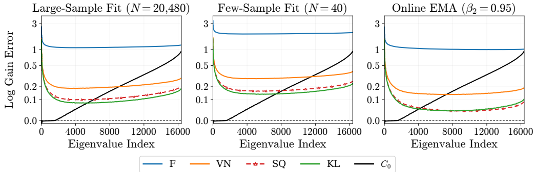
Figure 6: Smoothed log held-out gain error for the output projection at AdamW step 2,500. Closer to zero is better; with asinh vertical scale. Left: large-sample fit; middle: 40-sample fits (4 repeats); right: EMA (16 repeats). Black solid: large-sample C_0^{-1/2} in all panels; dashed: the held-out target.
