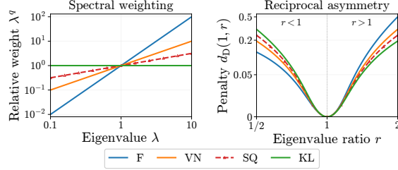
Figure 3: Left: Normalized penalties \frac{d_D(\lambda, r\lambda)}{d_D(1, r)} = \lambda^{q_D} for r \neq 1 . Smaller q places less emphasis on large eigenvalues; KL is scale-independent. Right: d_D(1, r) versus r , with a log horizontal scale and an asinh vertical scale. F and VN favor underestimation over reciprocal overestimation, KL shows the opposite preference, and SQ is symmetric.
