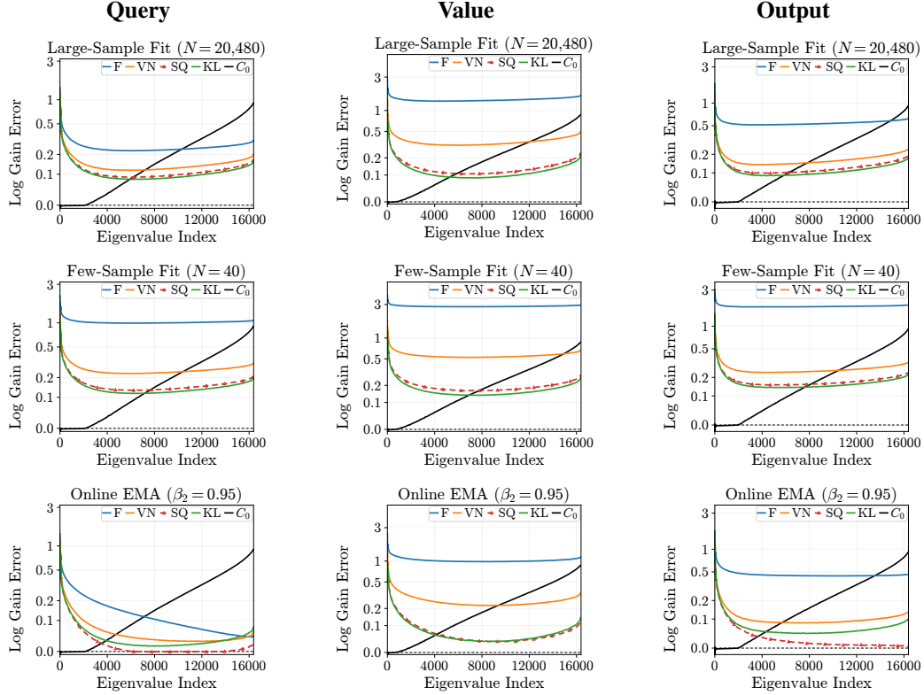
Figure 12: Held-out gain error on AdamW checkpoints at step 4500. Rows: large-sample fit, 40-sample fit, EMA with eigendecomposition every five steps.
