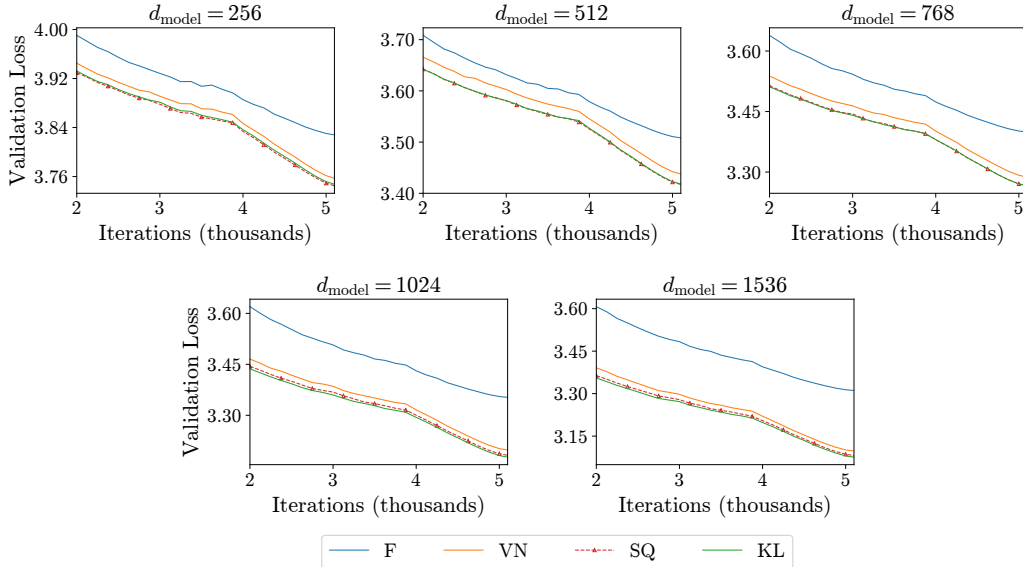
Figure 16: Validation loss from step 2,000 at all five widths.
