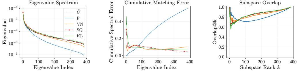
Figure 7: Smooth synthetic setting. From left to right: empirical and fitted spectra, cumulative spectral error, and leading-subspace overlap. Finite-sample stability is shown in Figure 4 (right).
