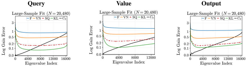
Figure 10: Held-out gain error on AdamW checkpoints at step 100. Rows: large-sample fit, 40-sample fit, EMA with eigendecomposition every five steps.
