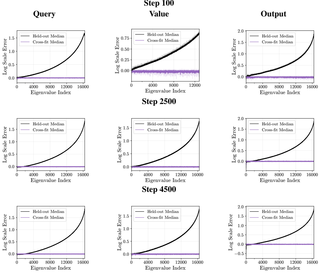
Figure 9: Held-out scale error. Rows: steps 100, 2500, 4500. Bands show split-comparison IQRs.
