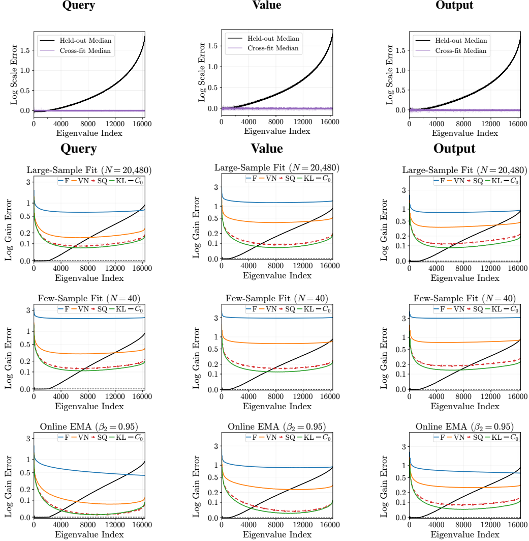
Figure 15: Distributed Shampoo diagnostics at step 2500. Top: held-out scale error and cross-fit controls. Remaining rows: held-out gain error for large-sample fits, 40-sample fits (four repeats), and EMA (512 gradients, 16 repeats, eigendecomposition every five steps).
