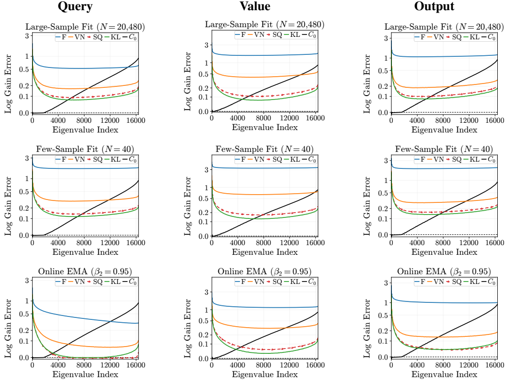
Figure 11: Held-out gain error on AdamW checkpoints at step 2500. Rows: large-sample fit, 40-sample fit, EMA with eigendecomposition every five steps.
