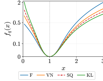
Figure 2: The family of scalar generators f_q(x) inducing trace-power Bregman divergences we study through one unifying lens. Shown with an asinh vertical scale.
