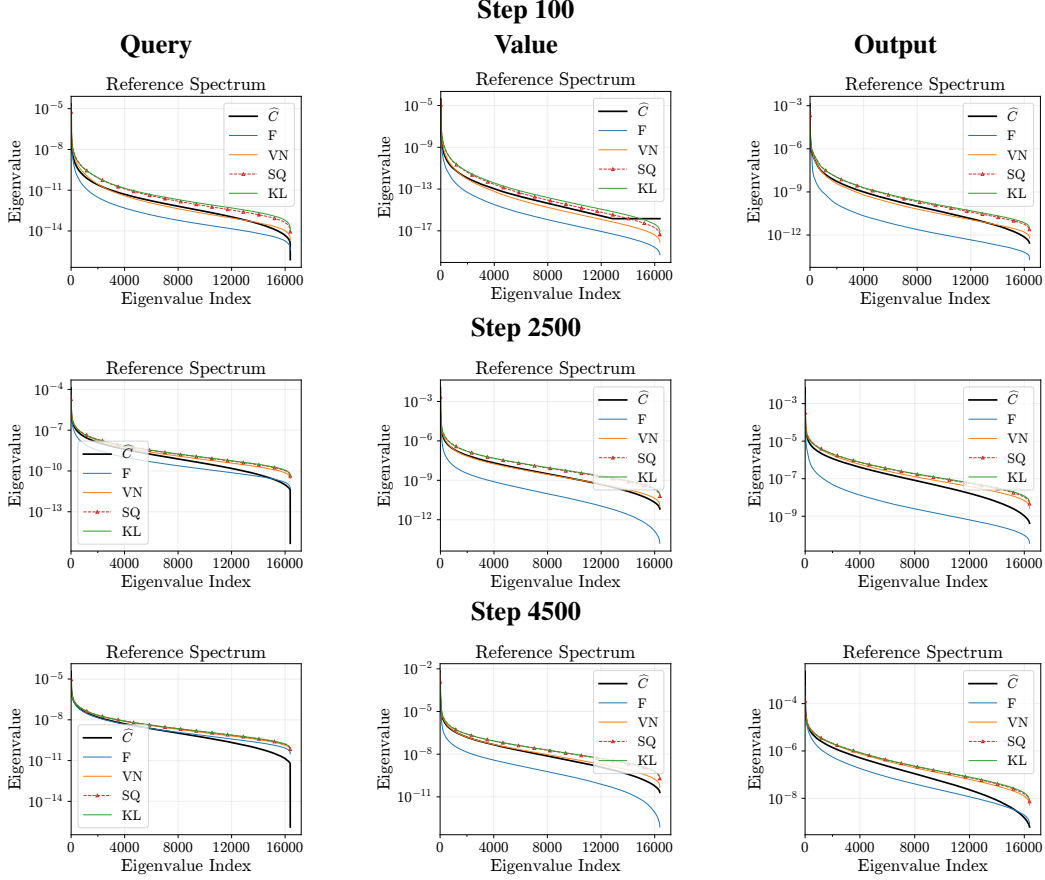
Figure 13: Large-sample spectra. Rows: steps 100, 2500, 4500.
