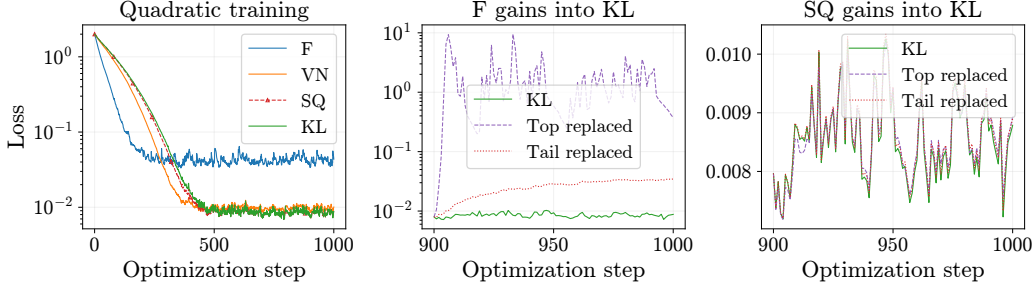
Figure 8: Quadratic training loss averaged over 3 seeds. Left: four methods. Middle and right: replacing KL gains from step 900. F gains raise loss in either region; SQ gains leave it close to KL.
