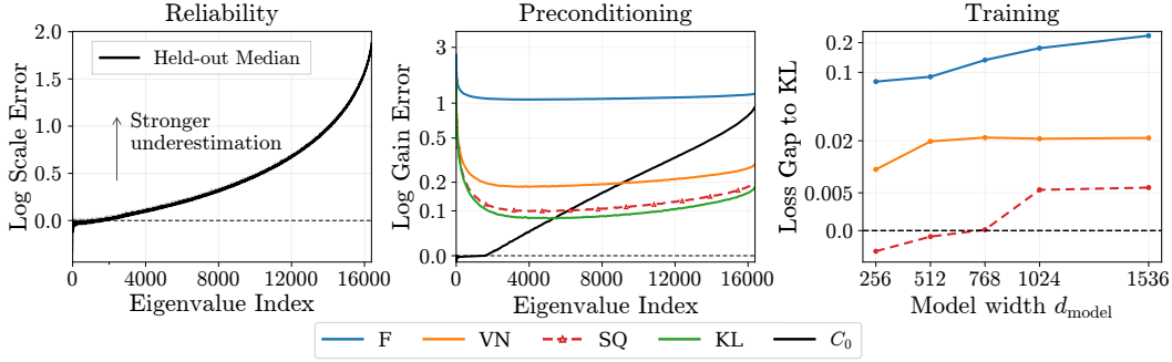
Figure 1: Divergences shape preconditioning and training. Left and middle: A GPT-2 checkpoint (output_proj) at step 2,500, ordered by decreasing eigenvalue. Left: Empirical second-moment ( C_0 ) eigenvalues become less reliable toward the tail, increasingly underestimating held-out scales (Section 4.1). Middle (smoothed curves, asinh y-axis for better resolution near zero): KL stays closest to the held-out target (dashed zero line), followed by SQ, compensating C_0 ’s scale errors (Section 5). Right: GPT-2 validation loss relative to KL with asinh y-axis; lower is better (Section 6).
