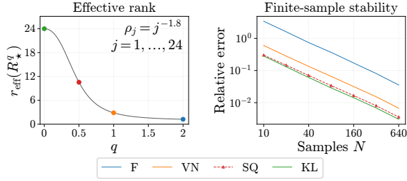
Figure 4: Left: Effective rank r_{\text{eff}}(R_*^q) for eigenvalues \rho_j = j^{-1.8} . Right: Mean squared relative Frobenius error of the jointly fitted S = L \otimes R (Equation (19)) on non-Kronecker gradients over 20 repeats, relative to each method’s 4096-sample fit. Both results favor smaller q_D , consistent with the theoretical prediction in Proposition 4.
