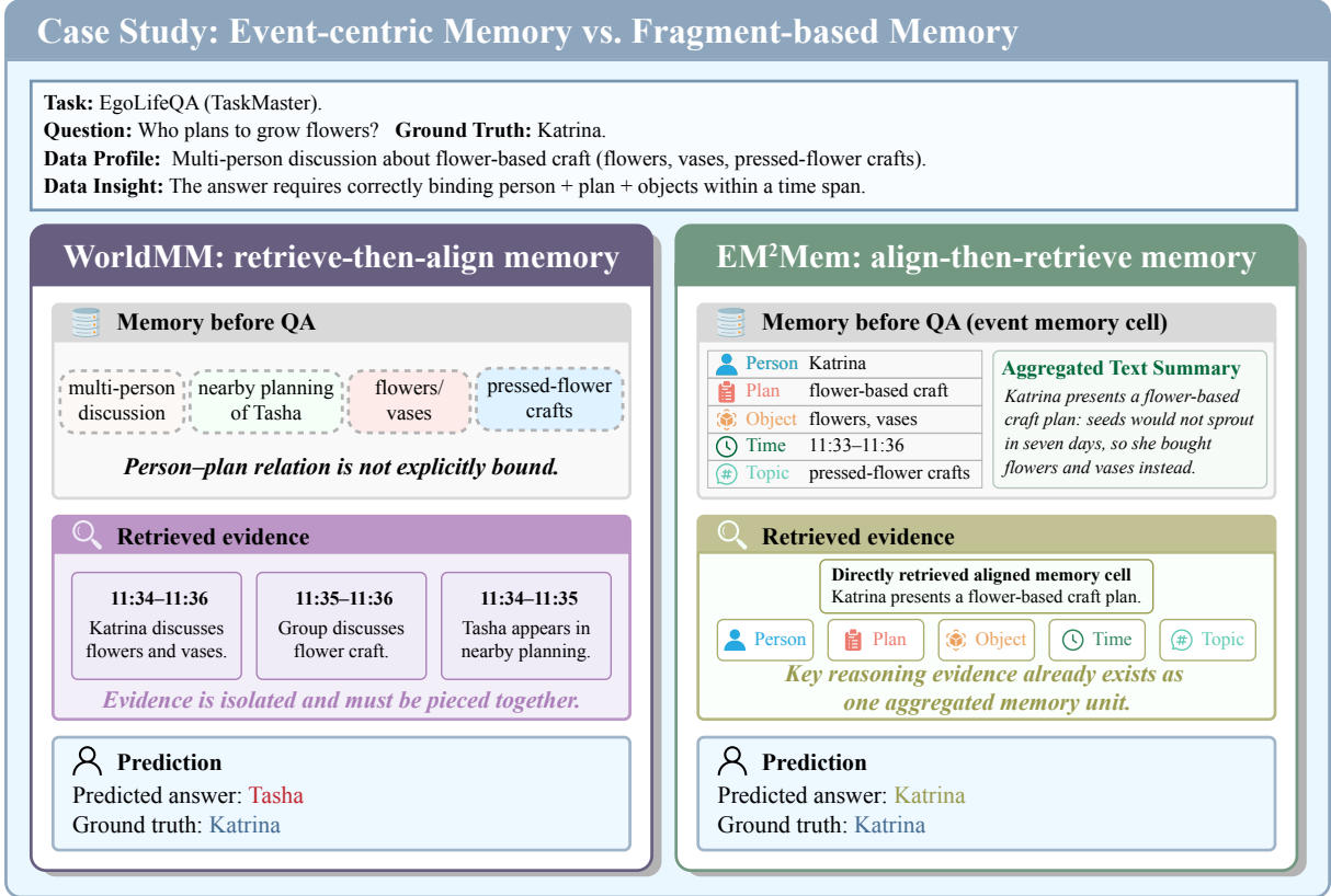
Figure 5: Case study of TaskMaster in EgoLifeQA.
