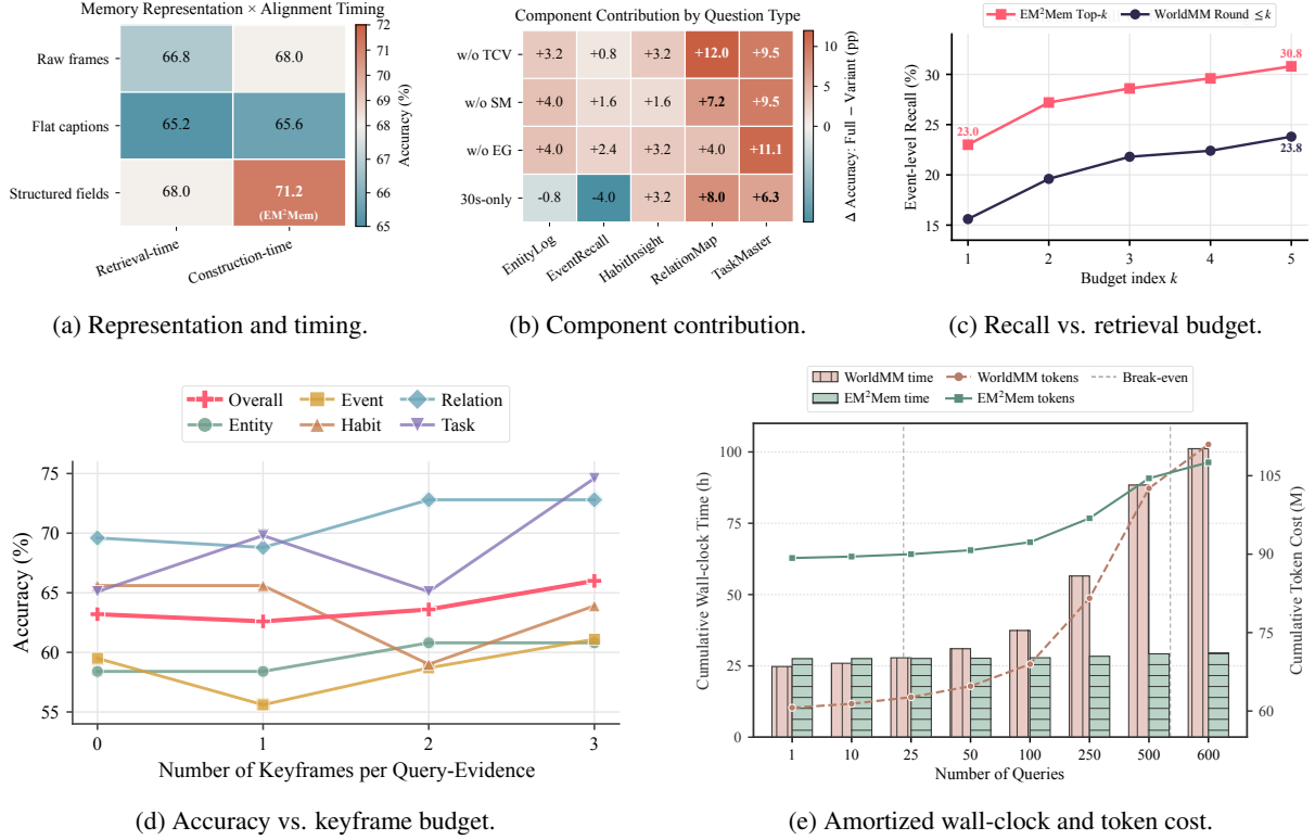
Figure 3: Analysis of EM²Mem design choices and efficiency. (a) Structured event fields with construction-time unification achieve the best accuracy. (b) Component-wise ablations show different contributions across question types. (c) EM²Mem improves event-level recall as retrieval budget increases. (d) Visual keyframes improve overall accuracy, especially with three keyframes. (e) EM²Mem amortizes its wall-clock overhead as the number of queries increases; dashed lines indicate wall-clock and token break-even points.
