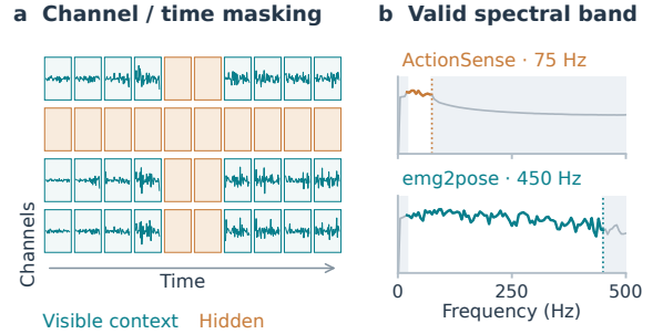
Fig. 2. Supported-band target construction. (a) Real emg2pose training signals with an illustrative whole-channel/time mask; hidden patches are orange. (b) Log-amplitude spectra from ActionSense and emg2pose training patches on the same 1 kHz grid. Gray regions are excluded from the spectral reconstruction loss. Cutoffs reflect these recordings.
