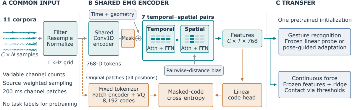
Fig. 1. EMGBlend’s heterogeneity-aware architecture. Shared Conv1D patch embeddings feed seven temporal–spatial attention pairs with sensor geometry. The frozen tokenizer supplies code targets (orange); encoder features support downstream decoding (blue). Attention grids indicate axes, not measured weights.
