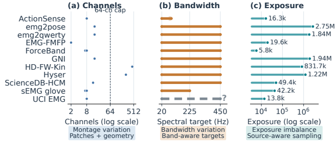
Fig. 3. Heterogeneity of the 11-source pretraining pool. (a) Released channel counts and the 64-channel sampling cap. (b) Recording-supported frequency ranges used by the spectral target; UCI’s effective upper cutoff is uncertain. (c) Naive available-window \times capped-channel exposure before source-aware acceptance. The three panels motivate the montage, target, and sampling mechanisms.
