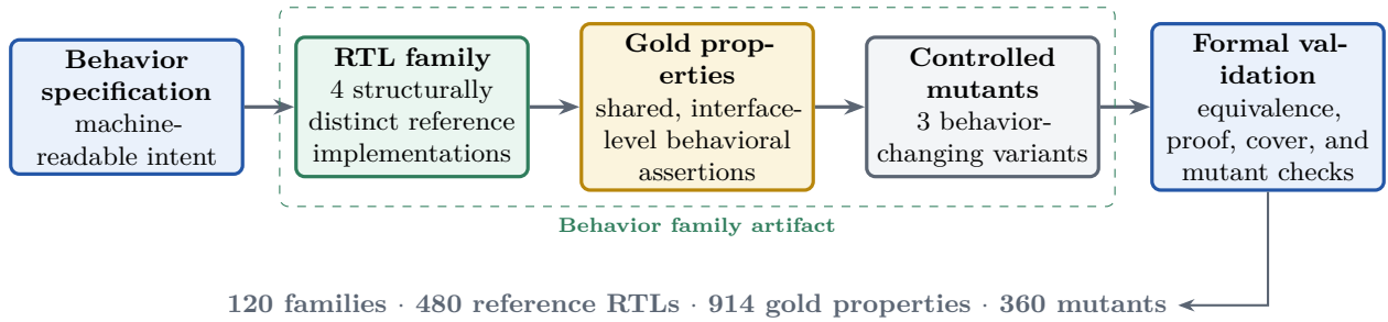
Figure 1: EQUIV SVA construction and validation pipeline. The family abstraction keeps intended behavior fixed while exposing multiple implementation structures and controlled behavior-changing mutants.
