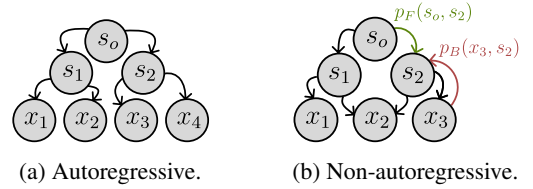
Figure 1: The state graph \mathcal{G} is a tree in an autoregressive setting (a). When many trajectories lead to the same state, such as s_o \rightarrow (s_1, s_2) \rightarrow x_2 in (b), \mathcal{G} is a non-tree DAG.
