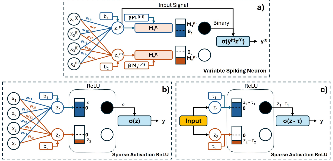
Figure 1: Sparse-Activation-ReLU Model (a) Visual demonstration of the Variable Spiking Neuron [17] operating after a linear fully-connected layer. Synaptic weights and unique bias terms accumulate the input for each neuron at spike time step t which is aggregated into the neuron’s leaky memory, mirroring LIF dynamics. VSN replaces the binary spike output with an activation function operating on the neuron input. (b) Sparse-Activation-ReLU for a fully-connected linear layer. We apply a ReLU activation function to the linear layer output which only allows positive signals subsequently operated on by a chosen activation function. Such forward pass communication allows for surrogate-free ANN-to-neuromorphic conversion that allows for variable signals (unlike traditional binary spike rate to activation matching), included in the original VSN framework. (c) Sparse-Activation-ReLU for a generic input (spectral/spatial convolution or norm). We apply a ReLU activation function to the input subtracted by an optional threshold utilized for better spiking control. Similar to the linear layers, the ReLU only allows positive signals subsequently operated on by a chosen activation function.
