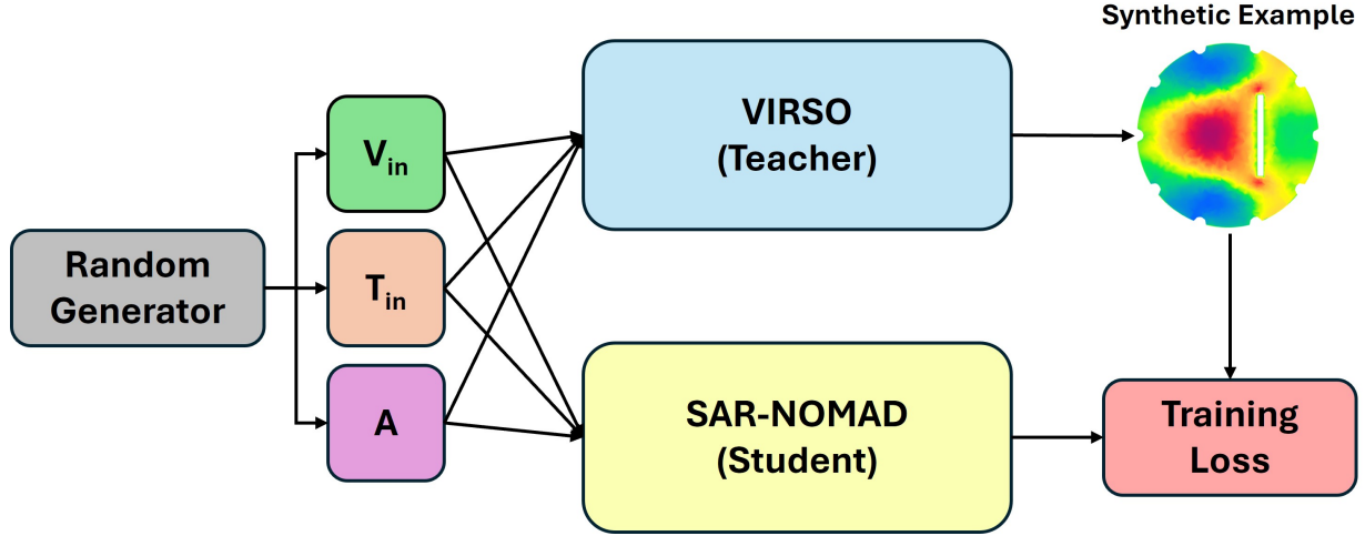
Figure 4: Synthetic Distillation We show the synthetic distillation framework utilized for neuromorphic virtual sensing. A graph-based VIRSO model, not native for neuromorphic hardware due to high connectivity and difficult integration, generates synthetic Heat Exchanger examples by randomly sampling input parameters for the Heat Exchanger dataset. These synthetic examples are compared against SAR-NOMAD’s predictions, a more neuromorphic friendly model, allowing for improved L_2 error performance in SAR-NOMAD, ideally keeping efficiency the same.
