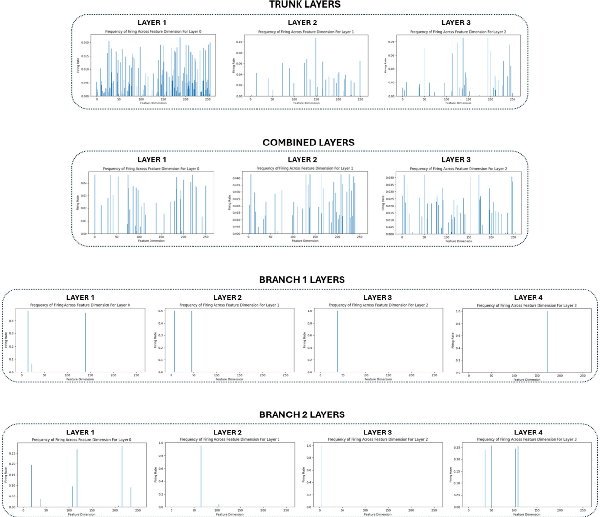
Figure 6: Spiking Activity Results We depict the probability/frequency of different feature dimensions spiking for the SAR-NOMAD model with the Hoyer loss and \gamma = 0.005 . For the branch layers, the sparsity regularization forces only a small subset, as a low as one dimension, to fire and communicate information, indicating that the model is forced to collapse its feature dimensions in order to provide low spiking. The trunk and combined subnetworks have a lot more activity across the entire dimension.
