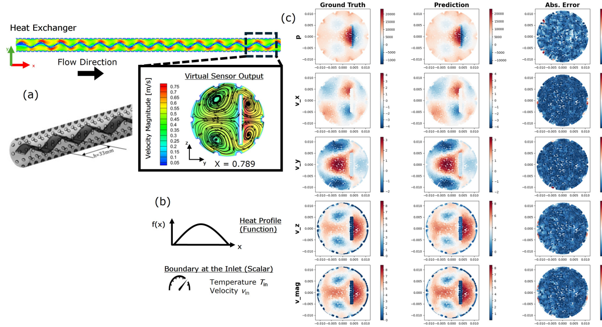
Figure 5: 2D Heat Exchanger (a) We define the 2D Heat Exchanger geometry which is a cross-sectional slice of a 3D grid at axial position x = 0.789 with a dimpled wall surface and tape insert utilized for better heat transfer, creating large vortex flow behavior and an irregular geometry with reduced symmetry (b) The boundary input utilized for our 2D Heat Exchanger. It includes a wall heat profile defined along the axial direction of the original 3D geometry and two inlet quantities: temperature and axial velocity/speed. (c) The 50th percentile test example for the SAR-NOMAD model with the Hoyer loss term and \gamma = 0.005 . We see that the main physics and vortex behavior is closely captured with mostly stochastic absolute error behavior and only small absolute error hotspots located around the wall surface.
