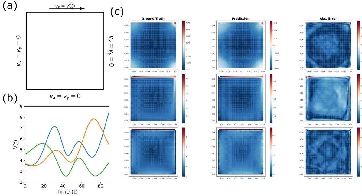
Figure 7: 2D Lid-Driven Cavity (a) We define the boundary conditions for the Lid-Driven Cavity geometry which shows zero velocity on all faces except for a temporal signal at the top surface. (b) We display example time-varying velocity profiles for the top surface which is defined for 90 time steps. (c) The 50th percentile test example for the SAR-NOMAD model with the Hoyer loss term and \gamma = 0.05 . We see that the main vortex and boundary behavior is closely captured as well as the corner eddies with mostly stochastic absolute error behavior. We do see small hotspots of absolute error located at the top surface and corners indicating some difficulty in capturing surface physics with a regular discretized grid.
