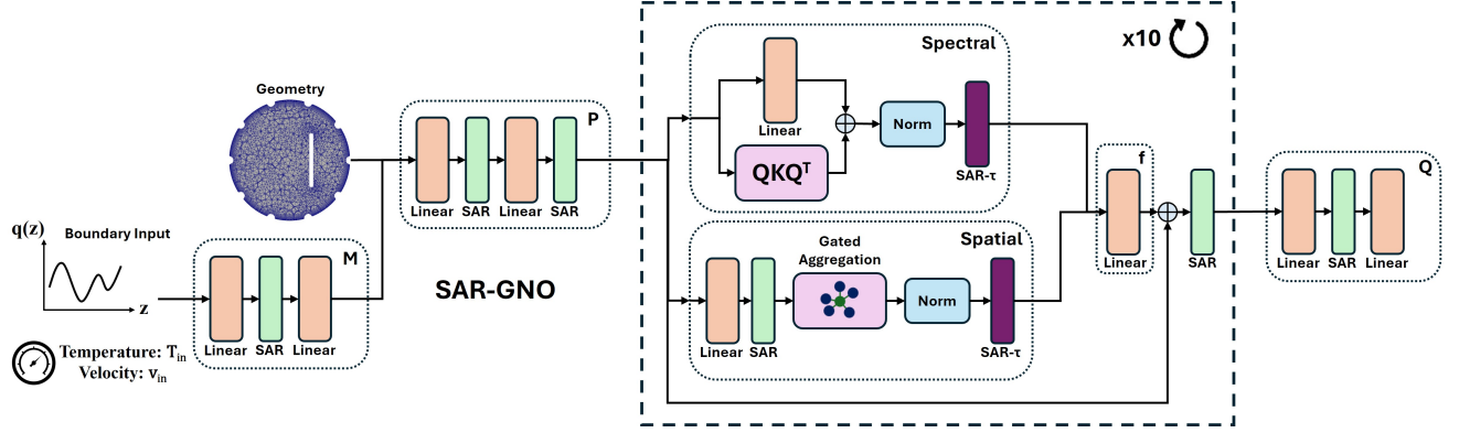
Figure 3: Sparse-Activation-ReLU Graph Neural Operator Architecture of SAR-GNO for the 2D Heat Exchanger. In green, exists every SAR layer included in the neural operator which does not utilize the optional threshold parameter. The green SAR layers replace either identity mappings or ReLU layers. Components in dark purple represent SAR with the optional threshold parameters \tau included for improved spiking control since they follow a normalization layer and non-linear computational layers. These threshold layers replace an identity mapping (spatial) and GeLU (spectral). SAR-GNO takes in boundary input with the input embedding mapping M and combines it with the geometry coordinates to produce an input for the latent projection mapping P . Subsequent spectral-spatial blocks (10 layers total) provide global and local analysis that is combined through a collaboration layer f . Final a downlift layer Q provides the final full-field reconstructed multi-physics output.
