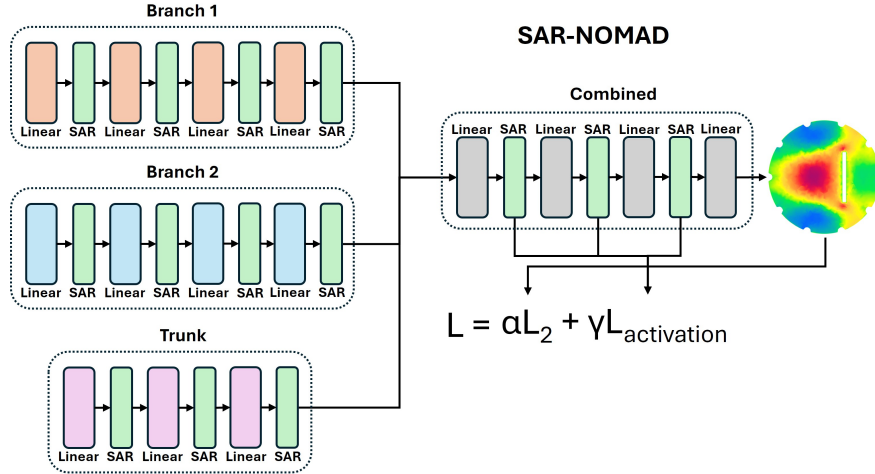
Figure 2: Sparse-Activation-ReLU Nonlinear Manifold Decoder for Operator Learning Architecture of SAR-NOMAD specifically for the 2D Heat Exchanger. In green, exists every SAR layer which naturally replaces the ReLU layers. Since every computation before SAR is a simple linear layer, we do not include a threshold parameter which is redundant in the presence of the bias term. As shown, the full-field output provides the L_2 error for the total objective function while the individual sparse activation outputs of the ReLU (from all SAR layers in the branch, trunk and combined networks not fully depicted in the figure) with the Hoyer/ L_1 loss term provide the control on energy efficiency.
