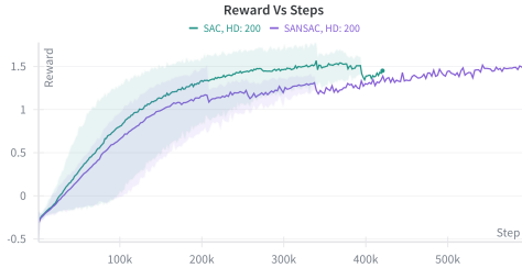
(c) Hidden dimension 200
