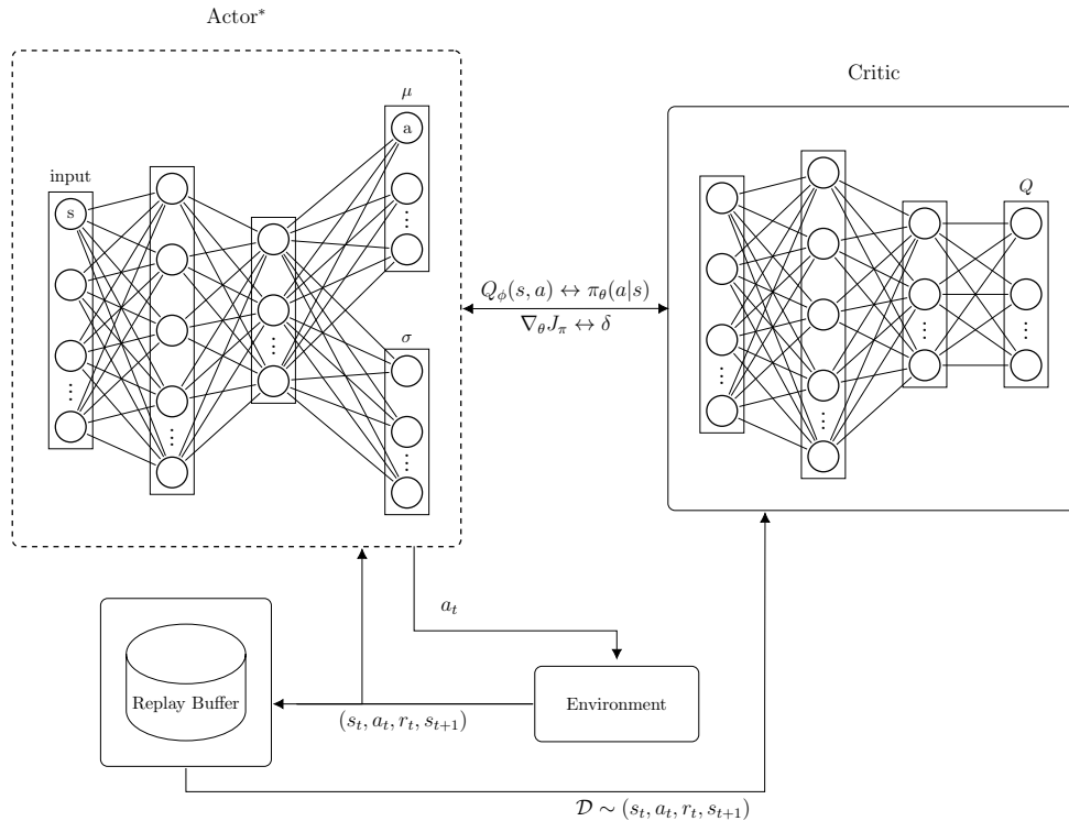
Figure 1: SANSAC/SAC Algorithm Diagram. Dashed border indicates spiking actor in SANSAC. All other components are identical between both algorithms. Critic outputs a state-action value Q(s, a) . Actor outputs a policy \pi(a|s) .
