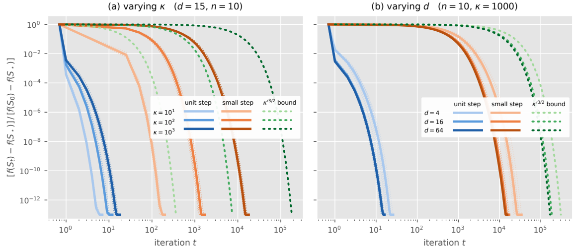
Figure 2: Unit-step (blue) against small-step (orange) RGD on pinned ensembles (every R_i of condition number exactly \kappa ), 12 instances per band (translucent) with opaque medians; darker shades for larger parameter values, gaps normalized by their initial value. (a) Varying \kappa at d = 15 : median iterations to the numerical floor range over 6 to 16 for the unit step, against 175 to 16288 for the small step. (b) Varying d at \kappa = 10^3 : the unit-step counts are essentially flat over a sixteenfold increase in d , as Theorem 10 asserts; the small-step counts track the conditioning \kappa' , not the dimension (see text). Dotted curves show the a priori guarantee of Corollary 17 at each setting’s median \kappa' ; the clip never activates, so the projected and unprojected unit steps coincide. Note the logarithmic iteration axis.
