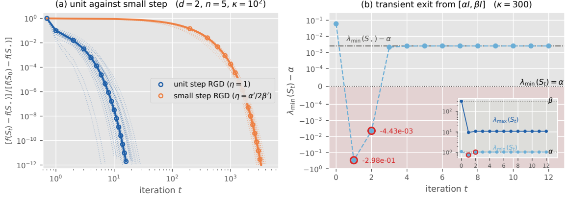
Figure 1: (a) Unit-step against small-step RGD on 30 instances of the pinned family at d = 2 , n = 5 , \kappa = 100 (every member with spectrum \{\alpha, \beta\} in a Haar-random eigenbasis), from the initialization S_0 = \frac{\alpha + \beta}{2}I : the relative optimality gap per iteration, translucent per instance with the medians opaque. At the median, the unit step converges to machine precision in 16 iterations, the small step \eta = \alpha'/(2\beta') of [ACGS21] (marked every 200th iterate) in about 3300. (b) The transient exit of Example 13 ( \kappa = 300 ): the signed deviation \lambda_{\min}(S_t) - \alpha of the unprojected unit-step iterates, on a symmetric log scale. The iterates at t = 1, 2 (circled) fall below the floor \alpha (dotted), by 2.98 \times 10^{-1} and 4.43 \times 10^{-3} , before re-entering at t = 3 and converging to the strictly interior limit \lambda_{\min}(S_*) - \alpha \approx 2.52 \times 10^{-3} (dash-dotted). The inset shows the full trajectory of both eigenvalues against the well-conditioned band [\alpha I, \beta I] := \{S : \alpha I \leq S \leq \beta I\} .
