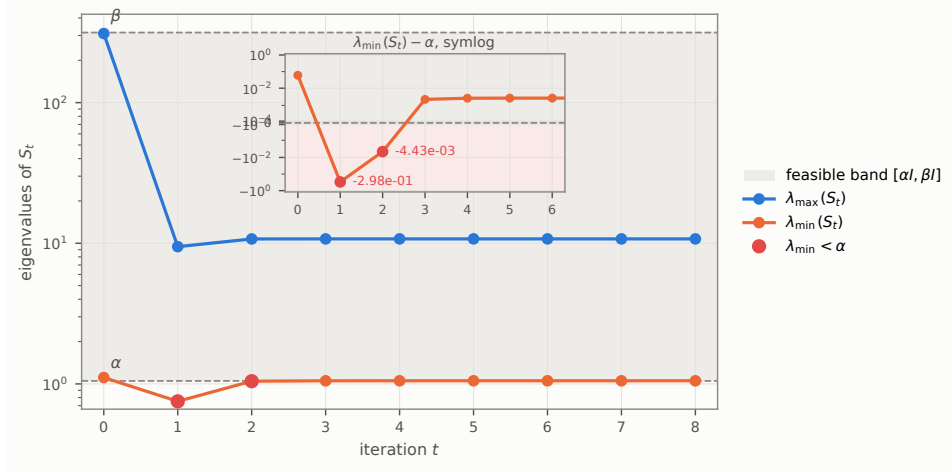
Figure 3: The trajectory of Example 13 . Main panel: both eigenvalues of the unprojected unit-step RGD iterates (log scale), with the feasible band [\alpha I, \beta I] shaded and the infeasible iterates marked. Inset: the signed deviation \lambda_{\min}(S_t) - \alpha on a symmetric-log scale, resolving the two undershoots ( -2.98 \times 10^{-1} and -4.43 \times 10^{-3} ) against the limit \lambda_{\min}(S_*) - \alpha \approx +2.52 \times 10^{-3} : the iterate exits [\alpha I, \beta I] at t = 1 , is still outside at t = 2 , and re-enters at t = 3 .
