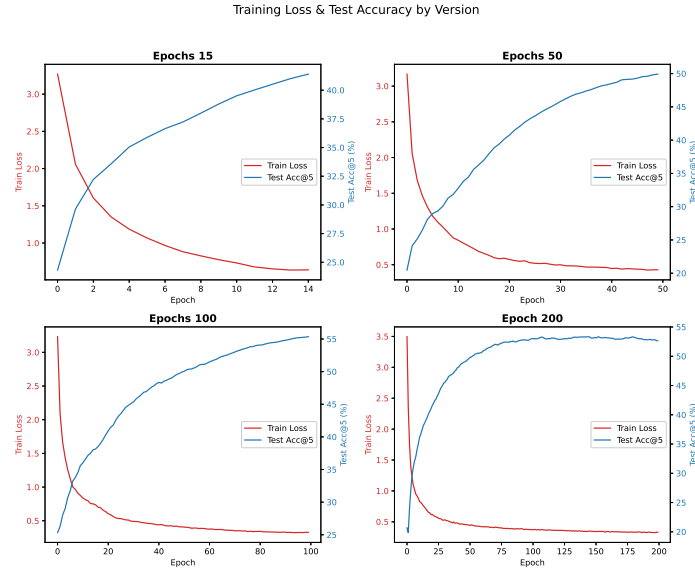
Fig. 5. Hybrid Quantum-Classical accuracy versus loss for SimCLR models with one QuFex layer injected at different epoch sizes.
