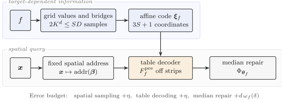
Figure 7: Proof architecture for the constructive upper bound. The target determines only the sampled values and latent vector. The spatial address network, decoder architecture, and affine loading rule are fixed, while the generated decoder parameters vary affinely with the latent vector. The capacity condition 2K^d \leq SD couples the number S of code blocks with the decoder length D .
