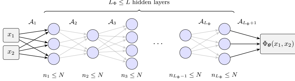
Figure 3: An architecture \Phi \in \text{Arch}(N, L) . The widths of hidden layers may be smaller than N , and all dense weight and bias entries are counted in P_\Phi .
