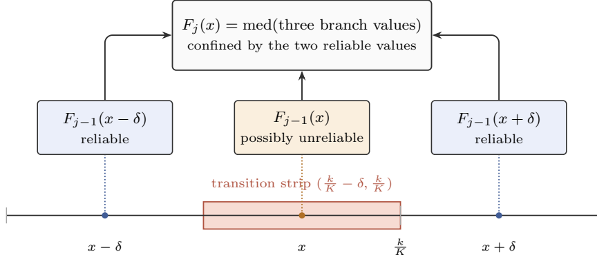
Figure 5: A representative one-dimensional transition. If x lies in a transition strip, the shifts x - \delta and x + \delta lie on its two sides. More generally, among the three translated branches at least two are reliable, so the median remains between the two reliable values, regardless of the remaining branch.
