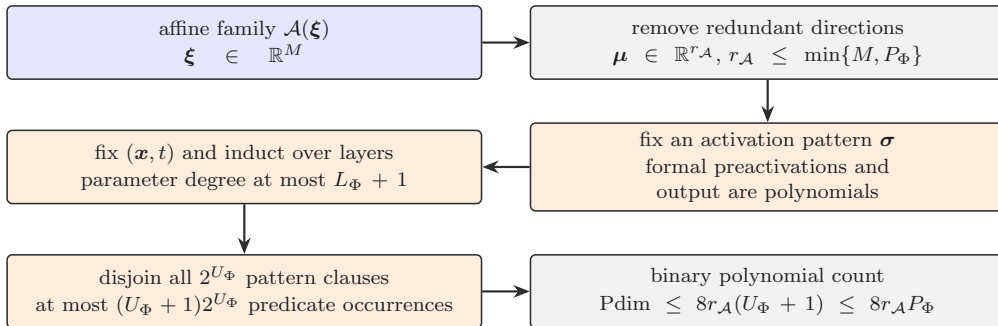
Figure 9: From affine parameter tying to the pseudo-dimension bound. Redundant latent-coordinate directions are removed before the network is represented, pattern by pattern, by polynomial predicates in only r_A effective variables. The exponential number of activation patterns appears inside a logarithm in Proposition 5.5.
