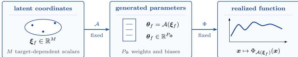
Figure 1: An affine latent parameterization. Only the M -dimensional latent vector \xi_f changes with the target. The shared affine map \mathcal{A} generates all P_\Phi network parameters, and the shared architecture \Phi realizes the approximation.
