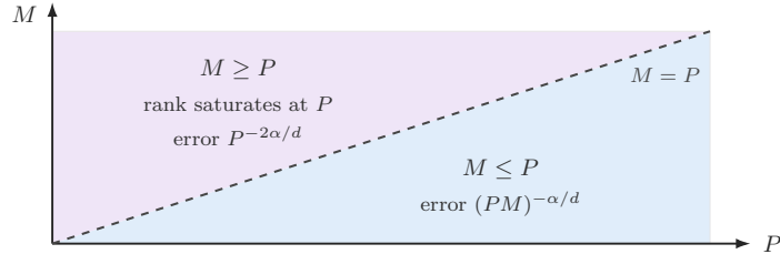
Figure 2: The sharp joint law in P and M in the nondegenerate regime of Theorem 3.1. For M \leq P , the effective scale is PM ; in particular, each fixed M \geq 4 yields the rate P^{-\alpha/d} . For M \geq P , the affine image is limited by the ambient parameter dimension, and the rate saturates at P^{-2\alpha/d} .
