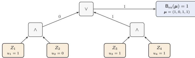
Figure 8: Evaluation of the fixed formula in (45). The orange boxes supply the changing input bits. The two \wedge gates, the \vee gate, and every edge of the tree are fixed before the bits are known.
