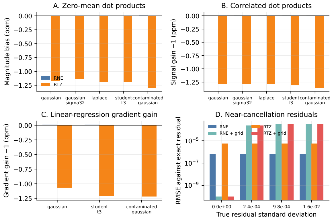
Figure 12: Statistical effect of the probe-matched emulator. RTZ produces a small toward-zero gain contraction across Gaussian and heavy-tailed dot products and regression gradients. Optional product-lattice canonicalization can eliminate exact-cancellation residue, but it also suppresses genuine residuals below its scale-dependent threshold.
