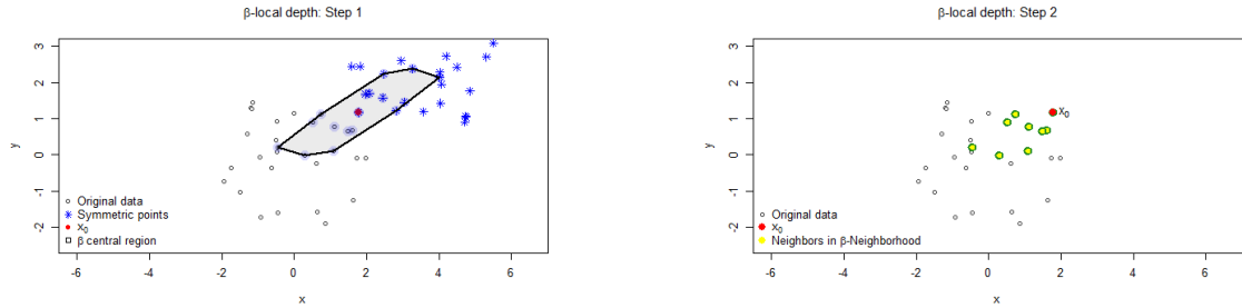
Figure 1. \beta -local halfspace depth construction for a sample of size n = 30 , with \beta = 0.3 . (a) Construction of the \beta -local depth region for \mathbf{x}_0 . (b) Depth-defined neighbors for \mathbf{x}_0 . The local depth of \mathbf{x}_0 is computed w.r.t. these neighbors.
