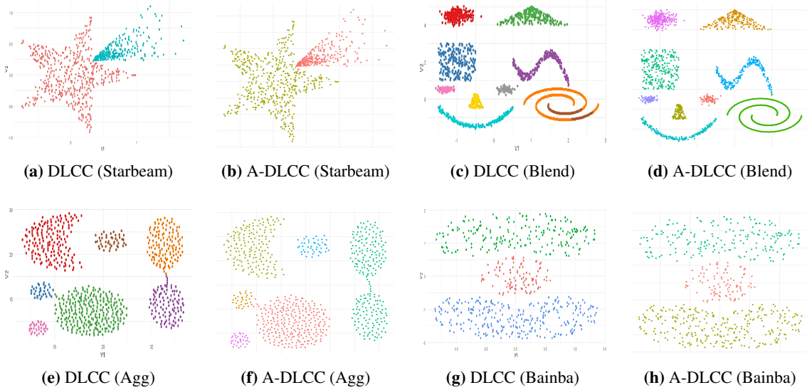
Figure 5. Comparison of clustering results by DLCC and A-DLCC on different synthetic datasets.
