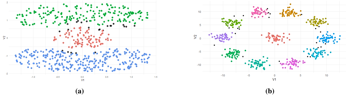
Figure 4. Temporary cluster results for two toy examples. (a) Bainba, where the groups are formed by bonding fragments of the interlocked shapes; (b) Normal, eleven normal components, where the groups are formed by absorption of the less representative local centers. Colors indicate retained points in each temporary cluster, while black points are unlabelled and left to be classified.
