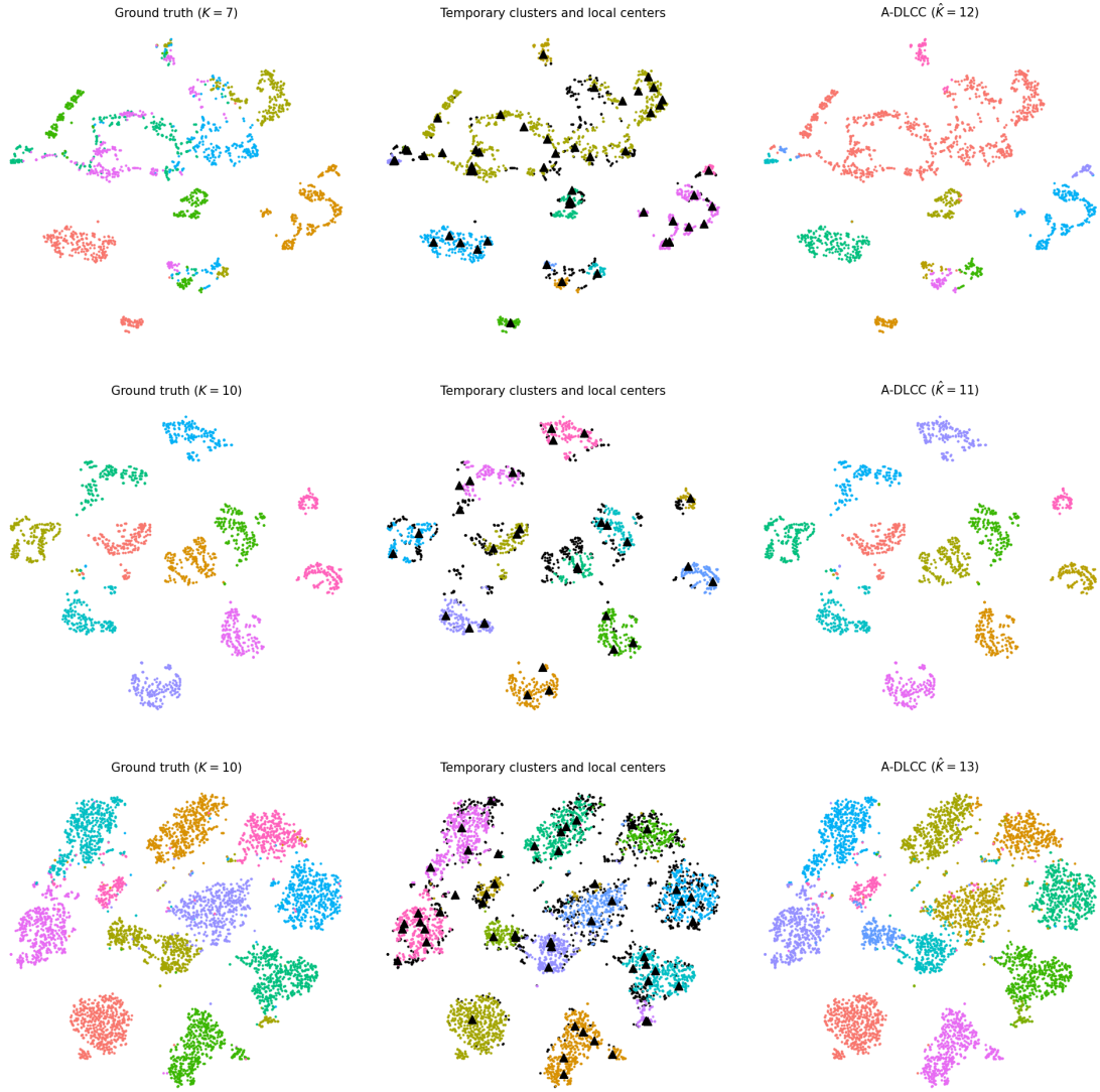
Figure 8. t-SNE visualizations for the Seg (top), Yale-B (middle), and Optidigits (bottom) datasets. Panel meanings are as in Figure 6.
