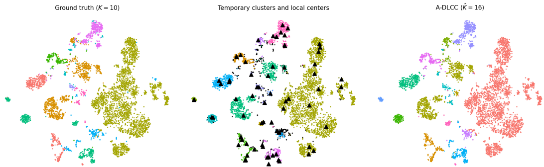
Figure 9. t-SNE visualization of Anuran Calls: ground truth, temporary clusters with local centers (triangles), and the A-DLCC result.
