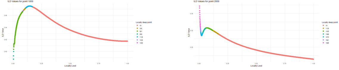
Figure 3. ILD values for two chosen points (Point 1000 and Point 2000) in the Yale-B dataset (Section 5.2) across varying locality levels. Colors indicate the locally deepest point in each neighborhood.
