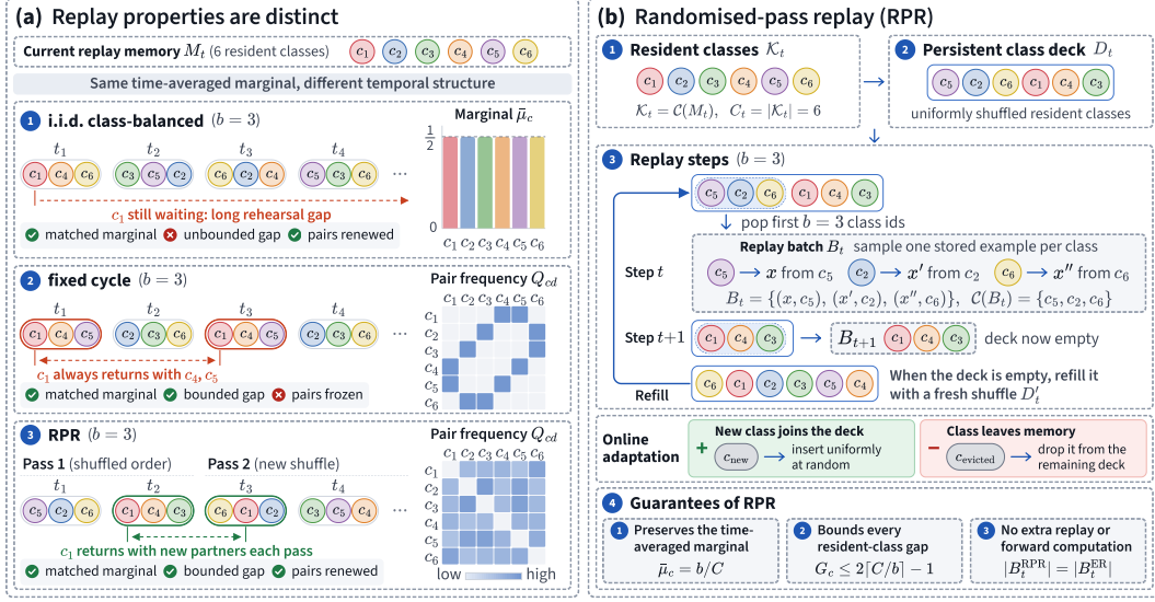
Figure 1: Replay properties and randomised-pass replay (RPR). (a) On a fixed resident set with replay batch b \leq C , independent balanced retrieval, fixed cycling, and RPR have the same time-averaged class marginal b/C but may differ in gap tails and class co-occurrence. (b) RPR keeps a persistent shuffled deck of resident classes, samples one stored example per selected class, and reshuffles when the deck empties. On a fixed resident set, it preserves \bar{\mu}_c = b/C and bounds G_c \leq 2\lceil C/b \rceil - 1 . It adds no replay examples or forward passes.
