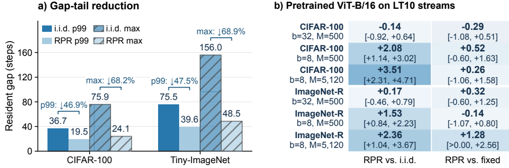
Figure 2: Temporal coverage and pretrained ViT evaluation. a , Linear-head ER-ACE resident-gap 99th percentiles and maxima on LT10 streams (ten-seed means); arrows show relative reductions. b , RPR minus indicated comparator (percentage points; 95% paired confidence intervals, ten seeds). Row labels give replay batch b and buffer capacity M ; colours are centred at zero. Table 3 gives baseline gaps.
