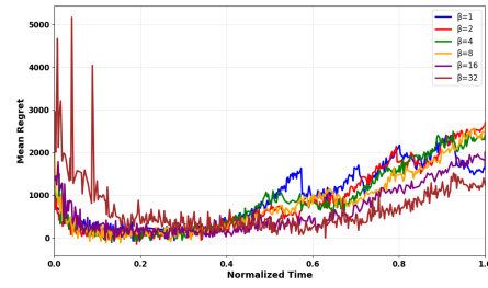
(b) Powell
