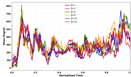
(c) Eggholder
