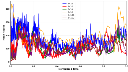
(c) Eggholder
