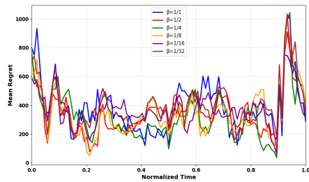
(c) Eggholder
