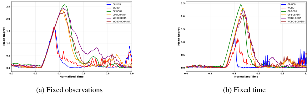
Figure 32: Both figures show how different models performed based on the metric mean regret over time on the Hartmann 3 function.
