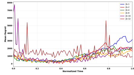
(b) Powell
