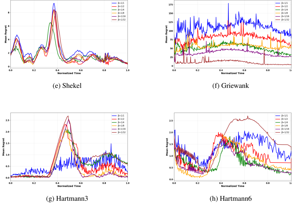
Figure 19: All eight figures show the mean regret with time for all eight simulations for the WDBO-BOBA (N) model with a fixed time horizon. All figures show how adapting the \beta value changes the models ability to minimize regret.
