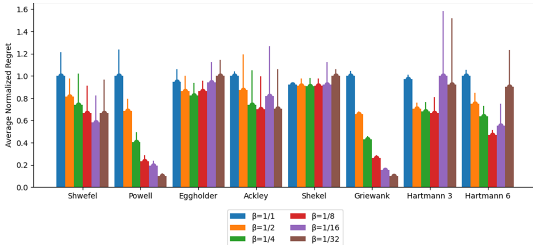
Figure 4: A grouped bar chart showing the variance \beta has on the GP-BOBA (N) model with fixed observation horizon for all simulations
