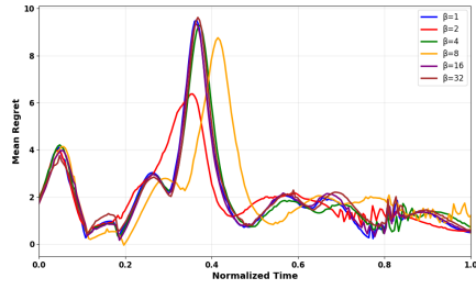
(e) Shekel
