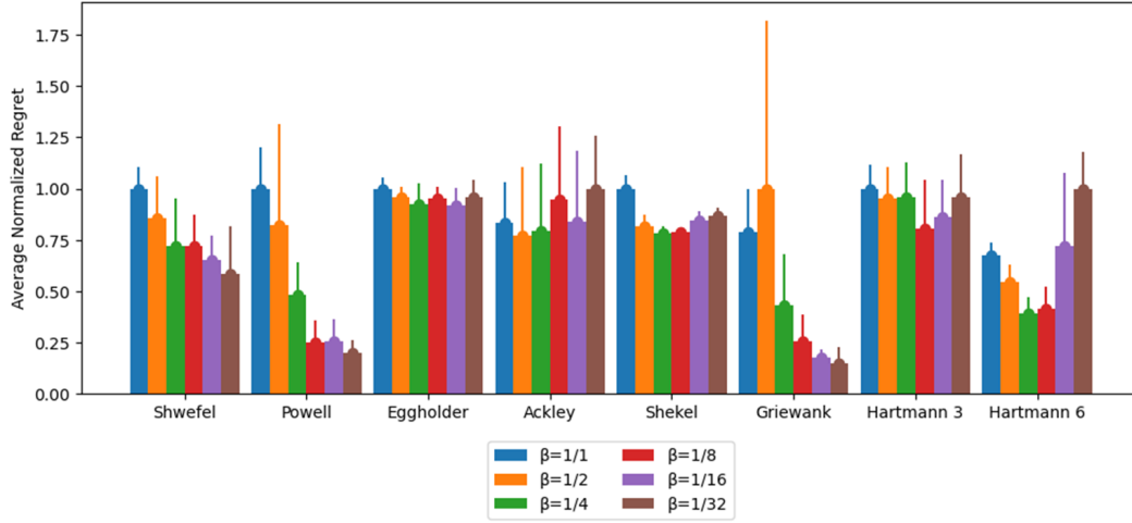
Figure 10: A grouped bar chart showing the variance \beta has on the WDBO-BOBA (N) model with fixed observation horizon for all simulations
