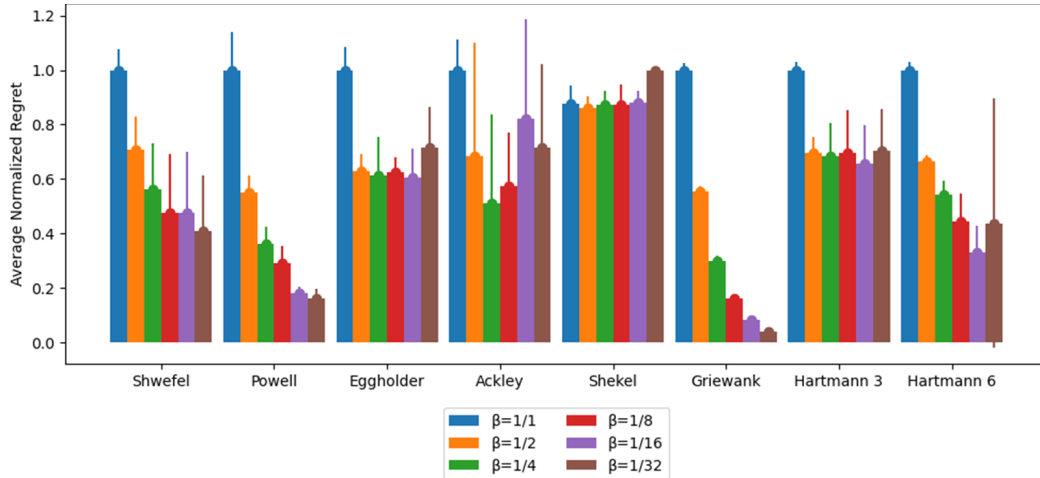
Figure 12: A grouped bar chart showing the variance \beta has on the GP-BOBA (N) model with fixed time horizon for all simulations
