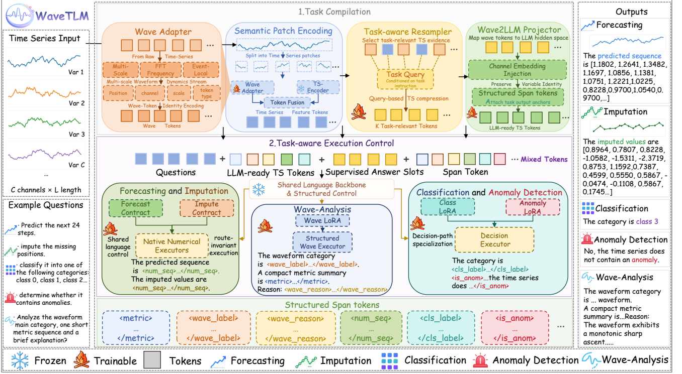
Figure 2: Compiler-executor architecture of WaveTLM. The task compiler binds a visible request to a typed contract and compiles semantic and waveform evidence into a task-conditioned state. Task-native executors then construct the corresponding numerical tensor, legal decision, or structured temporal record.
