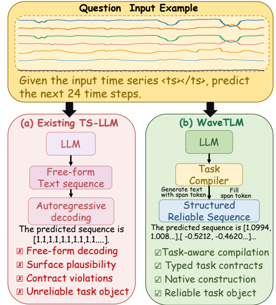
Figure 1: From plausible text to reliable time-series outputs. Existing TS-LLMs generate free-form text, whereas WaveTLM compiles task intent and temporal evidence into a typed state and constructs a contract-aligned output.
