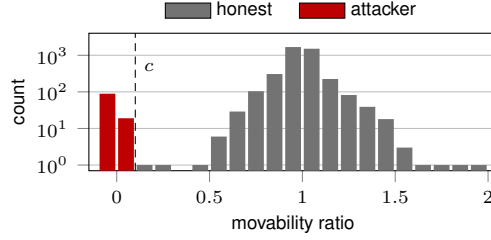
Figure 7: Movability ratio of every candidate tested in the 16-node runs with one, two and three attackers. The dashed line is c .
