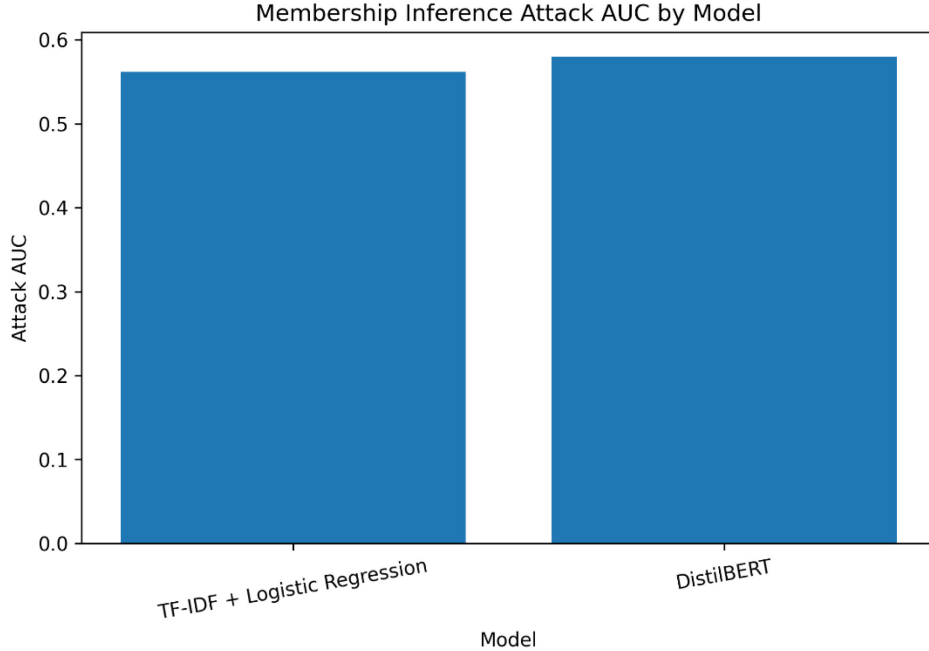
Figure 2: Attack AUC for the two baseline models.
