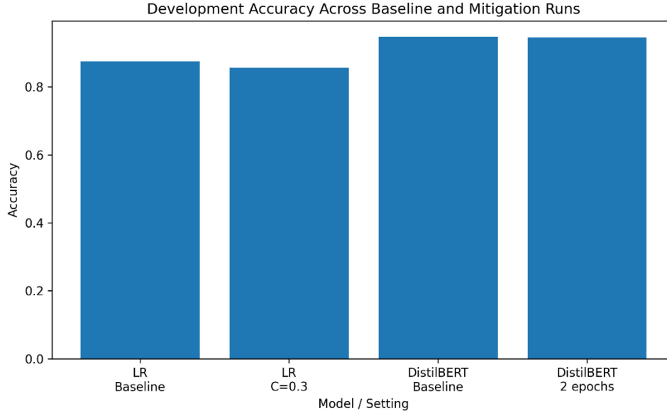
Figure 3: Development accuracy across baseline and mitigation runs.
