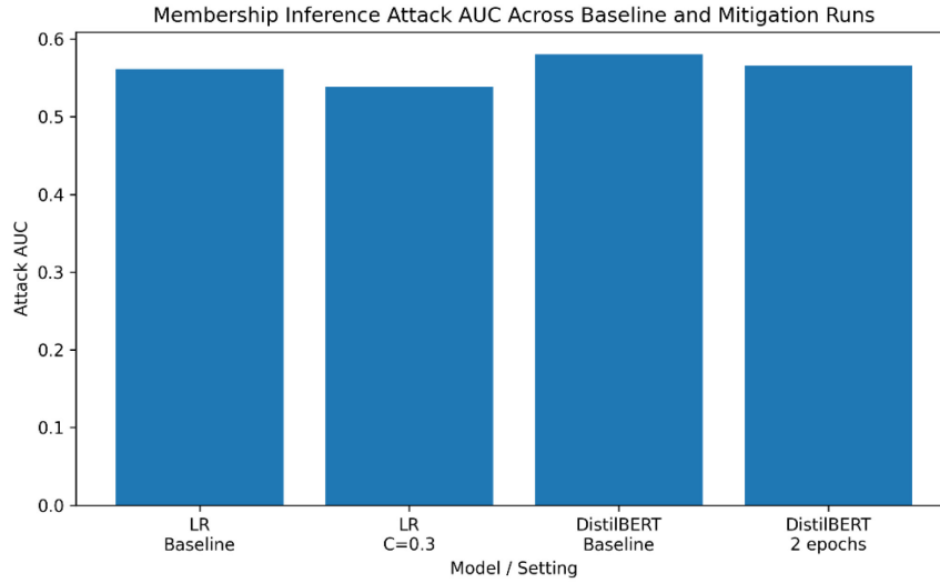
Figure 4: Attack AUC across baseline and mitigation runs.
