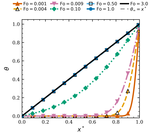
Figure 2: Analytical solution of the transient diffusion benchmark at representative Fourier numbers.
