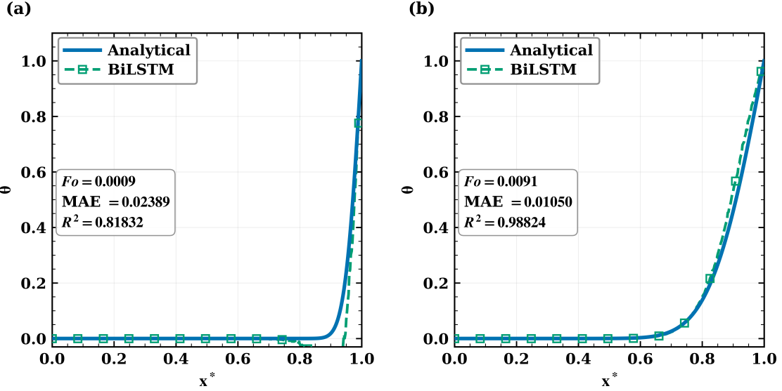
Figure 7: Extrapolation from the training range Fo \in [0.001, 0.009] using the Bi-LSTM to (a) Fo = 0.0009 and (b) Fo = 0.0091 , validated against the analytical solution.
