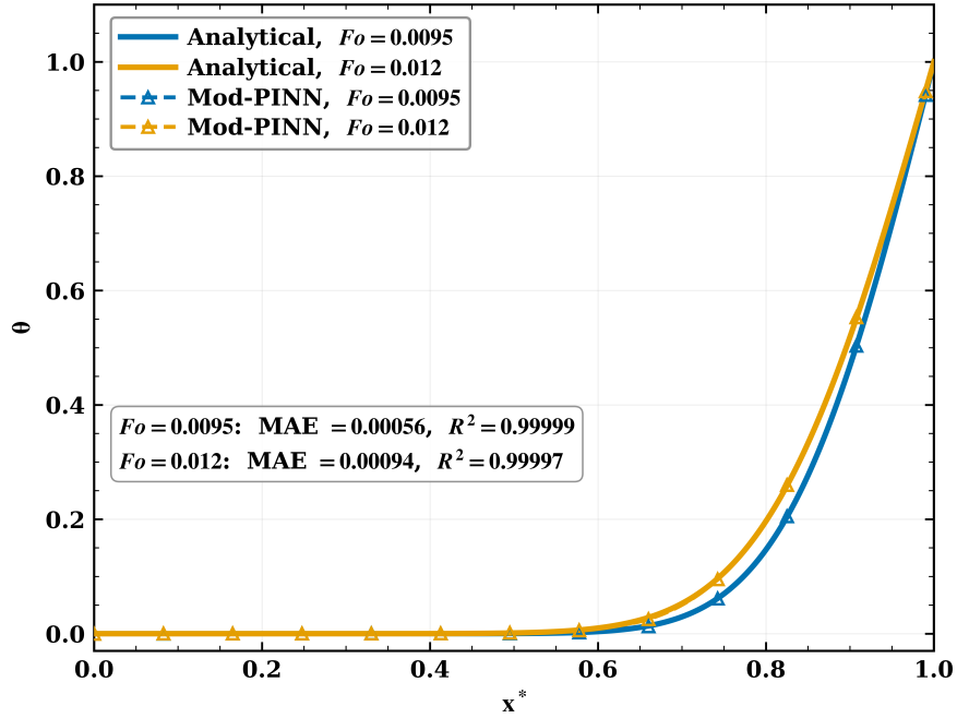
Figure 14: Forward extrapolation from the training range Fo \in [0.001, 0.009] using the Modified PINN across eight targets spanning Fo = 0.0091 – 0.0120 , validated against the analytical solution.
