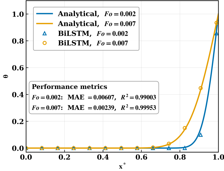
Figure 5: Interpolation within the training range Fo \in [0.001, 0.009] for the Physics-guided BiLSTM at (a) Fo = 0.002 and (b) Fo = 0.007 .
