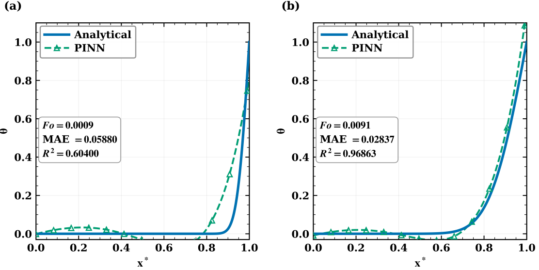
Figure 11: Extrapolation from the training range Fo \in [0.001, 0.009] using the PINN to (a) Fo = 0.0009 and (b) Fo = 0.0091 , validated against the analytical solution.
