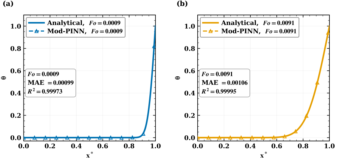
Figure 12: Extrapolation from the training range Fo \in [0.001, 0.009] using the Modified PINN to (a) Fo = 0.0009 and (b) Fo = 0.0091 , validated against the analytical solution.
