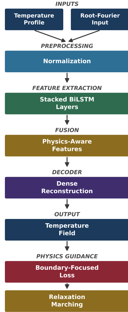
Figure 3: Physics-guided BiLSTM framework, the first of two independent demonstrations of the extrapolation-validation methodology: a Root-Fourier input ( s = \sqrt{Fo} ) realigns the network's time coordinate with the diffusion timescale, a boundary-weighted loss targets the highest-curvature region, and relaxation marching bounds error growth during sequential extrapolation.
