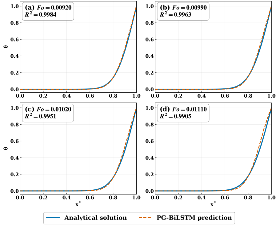
Figure 15: Physics-guided BiLSTM predictions at four increasingly distant forward targets, (a) Fo = 0.00920 , (b) Fo = 0.00990 , (c) Fo = 0.01020 , and (d) Fo = 0.01110 , each checked against the exact analytical solution.
