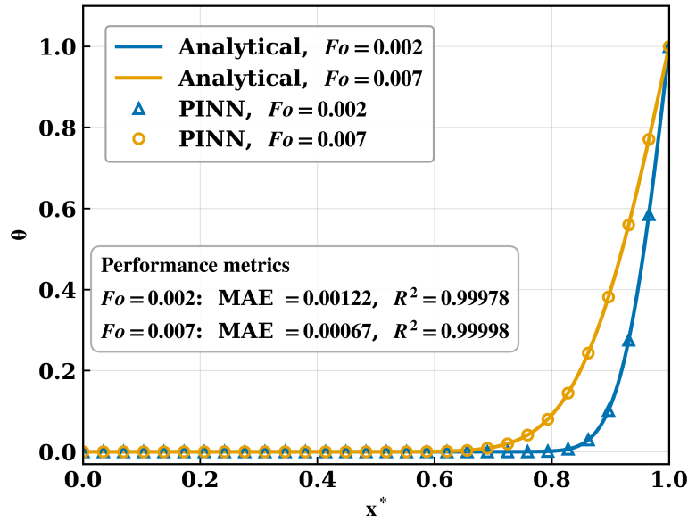
Figure 6: Interpolation within the training range Fo \in [0.001, 0.009] for the Modified PINN at (a) Fo = 0.002 and (b) Fo = 0.007 .
