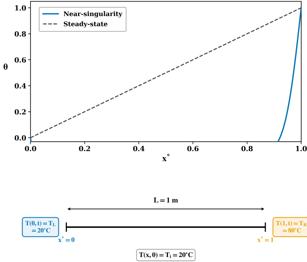
Figure 1: Physical configuration of the analytical benchmark: a step change in boundary temperature whose closed-form solution supplies exact, unlimited ground truth for certifying extrapolated predictions at every Fourier number.
