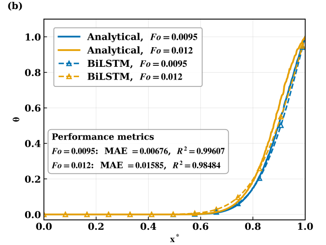
Figure 10: Forward extrapolation from the training range Fo \in [0.001, 0.009] using the Physics-guided BiLSTM to (a) Fo = 0.0095 and (b) Fo = 0.012 , validated against the analytical solution.
