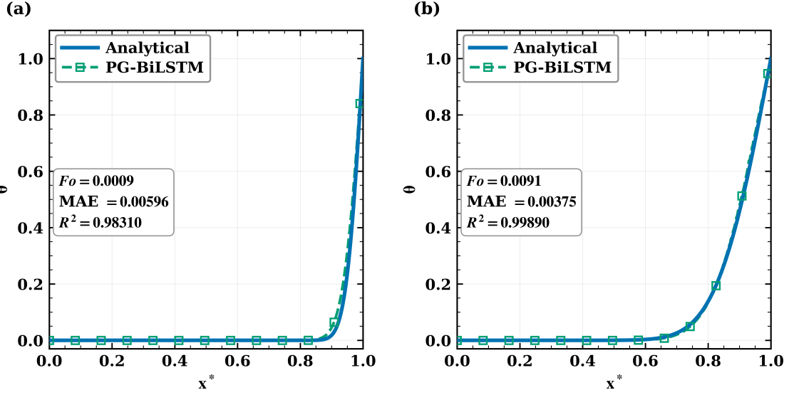
Figure 8: Extrapolation from the training range Fo \in [0.001, 0.009] using the Physics-guided BiLSTM to (a) Fo = 0.0009 and (b) Fo = 0.0091 , validated against the analytical solution.
