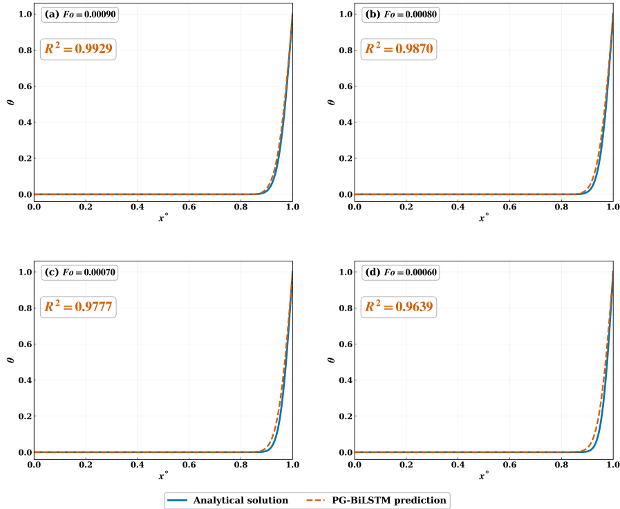
Figure 16: Physics-guided BiLSTM predictions at four increasingly distant backward targets, (a) Fo = 0.00090 , (b) Fo = 0.00080 , (c) Fo = 0.00070 , and (d) Fo = 0.00060 , each checked against the exact analytical solution.
