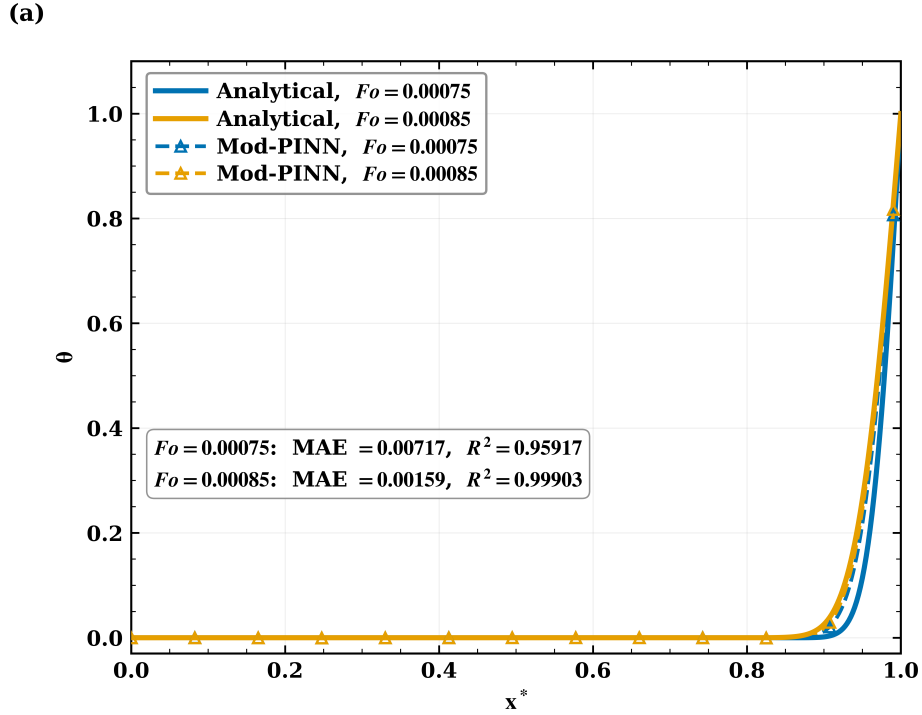
Figure 13: Backward extrapolation from the training range Fo \in [0.001, 0.009] using the Modified PINN to (a) Fo = 0.00075 and (b) Fo = 0.00085 , validated against the analytical solution.
