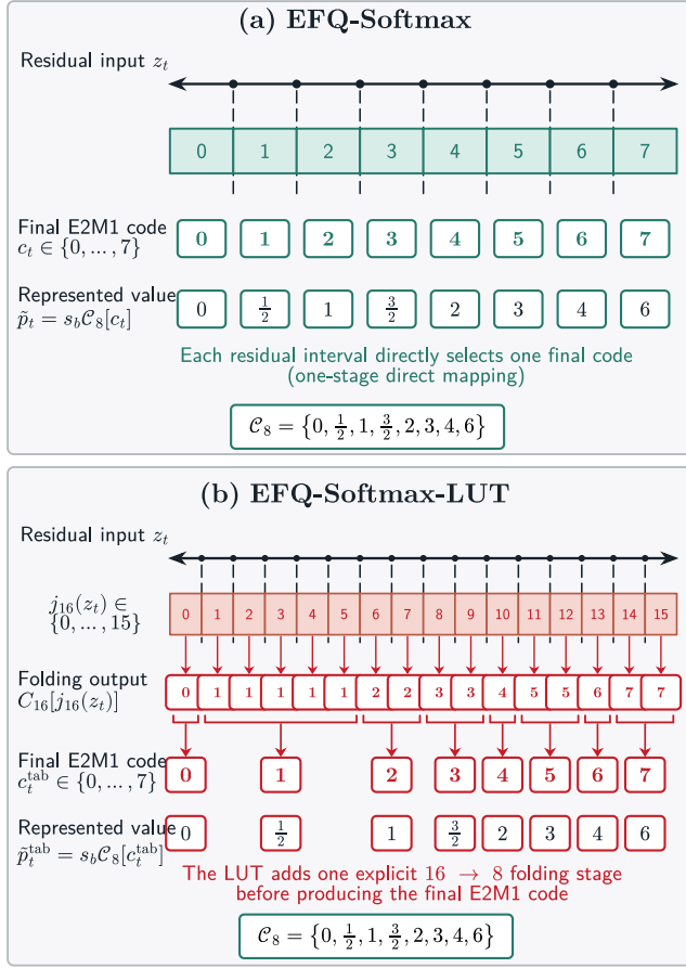
Fig. 4: Affine code mapping in EFQ-Softmax and two-stage mapping in EFQ-Softmax-LUT.
