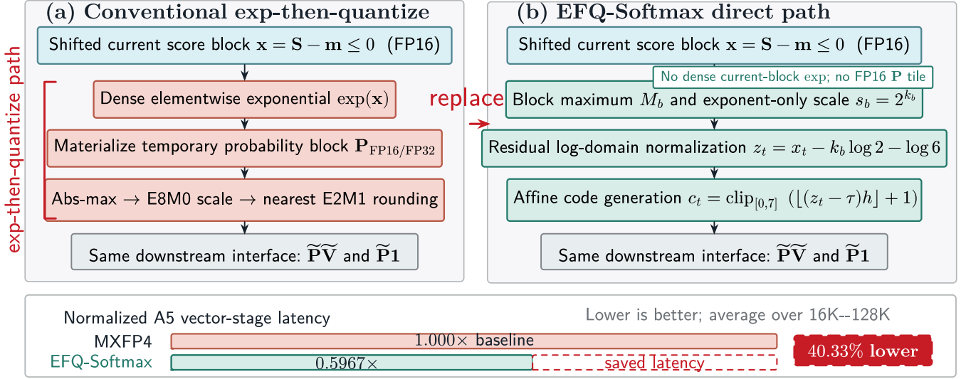
Fig. 2: Conventional exp-then-quantize versus EFQ-Softmax. EFQ-Softmax directly generates block-scaled E2M1 probabilities from shifted scores, reducing A5 vector-stage latency by 40.33%.
