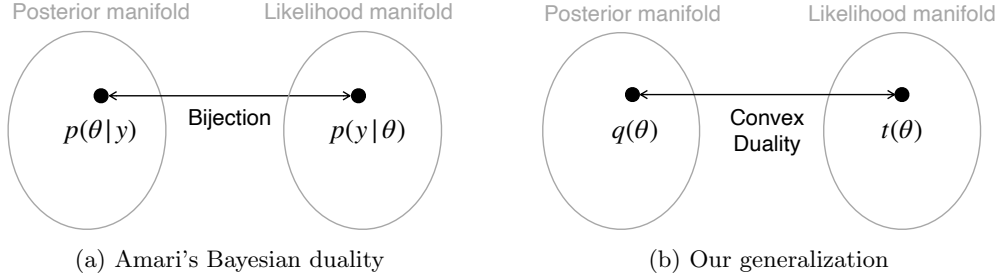
Fig. 1: Amari (1996) proposed a dual structure connecting the manifolds of posterior and likelihood (Panel a). In his case, a likelihood function p(\mathbf{y}|\boldsymbol{\theta}) over data vector \mathbf{y} given parameter vector \boldsymbol{\theta} is connected to a unique posterior p(\boldsymbol{\theta}|\mathbf{y}) and vice versa. His framework relied on a simple posterior form. We present a generalization by using convex duality which not only recovers Amari’s case but applies much more generally.
