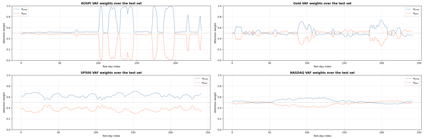
Fig. 7. Vertical Attention Fusion weights \alpha_{temp} and \alpha_{spec} across the 2023-06-01 to 2024-05-31 hold-out for KOSPI, Gold, S&P 500, and NASDAQ. The dashed line marks equal weighting. These four series span the range of gate behaviour observed on the evaluation panel, from episodic switching on KOSPI to near-static weighting on NASDAQ.
