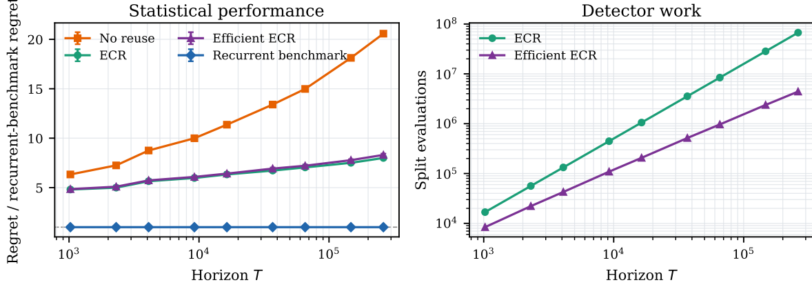
Figure 9. Geometric-grid ECR. (a) Regret relative to the recurrent benchmark’s Monte Carlo mean. (b) Total split evaluations. Results average 40 paired paths.
