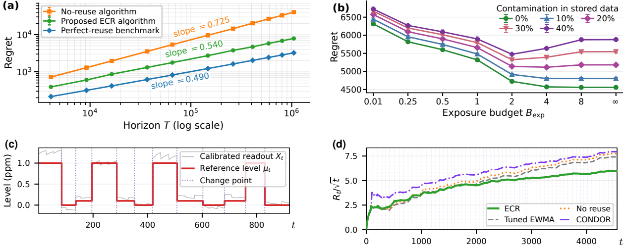
Figure 5. Numerical results. (a) Synthetic regret on log-log axes. (b) Exposure-budget tradeoff at different levels of source contamination. (c) Electronic-nose readouts and reference levels for the first 12 segments. (d) Regret over the full replay, normalized by \sqrt{t} . Error bars in (a) and (b) show 95% Monte Carlo intervals.
