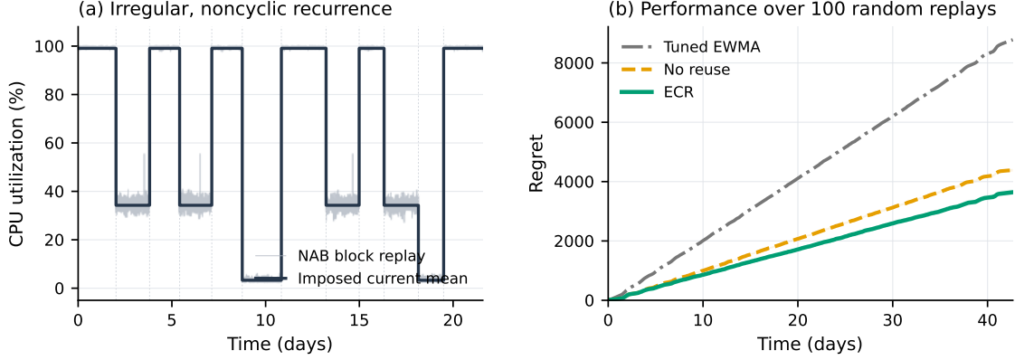
Figure 7. Trace-driven NAB replay. (a) The first 12 segments of one irregular, noncyclic replay. (b) Mean cumulative L_1 regret over 100 randomized replays.
