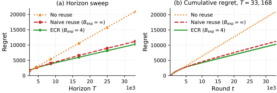
Figure 6. Exposure capping under persistent contamination. (a) Terminal cumulative L_1 regret as the subsequent recurrent sequence grows. (b) Cumulative regret at T = 33, 168 . Results average 100 paired paths.
