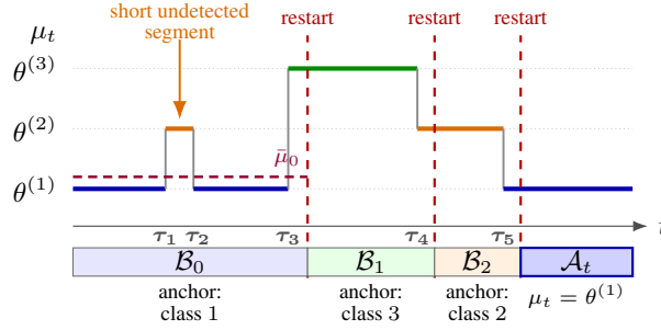
Figure 4. Schematic ECR segmentation. Red dashed lines delimit blocks created by detector alarms. Missed changes and detection delays introduce contamination, yet block \mathcal{B}_0 remains anchored at class 1.
