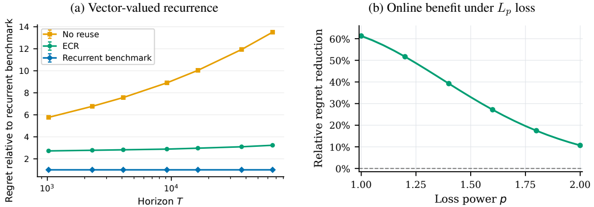
Figure 8. (a) Vector-valued recurrence. Euclidean regret relative to the recurrent benchmark for d = 5 , M = 4 , and S + 1 = \sqrt{T} , averaged over 40 paired paths. (b) Online benefit under L_p loss. Relative regret reduction of ECR over no reuse at T = 262, 144 , averaged over 30 paired paths.
