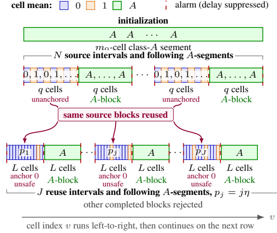
Figure 10. Environment illustration. Each cell represents two rounds. Each source interval is followed by a q -cell A -segment and produces an unanchored source block. Each reuse interval is followed by an L -cell A -segment and produces an unsafe block anchored at 0; the constant- A segments produce class- A blocks. During the latter half of each reuse interval, the same source blocks are accepted and reused, while all other completed blocks are rejected. The illustration is schematic and not to scale; alarm delays are suppressed.
