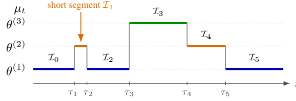
Figure 3. A recurrent environment. The mean undergoes S = 5 changes across M = 3 classes. Returns to previously visited classes create opportunities for data reuse. However, if the short segment \mathcal{I}_1 goes undetected, its observations can become mixed with those from the surrounding \theta^{(1)} segments. Reusing this mixed history when \theta^{(1)} returns can introduce bias.
