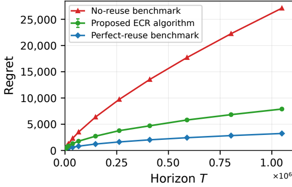
Figure 1. The value of recurrence. The setup is one where S \asymp \sqrt{T} and M = 4 . The widening regret gap between the no-reuse and perfect-reuse benchmarks illustrates the growing benefit (“value”) of ideal data reuse. Our proposed ECR algorithm is able to exploit this benefit without knowing the change points or class identities (Th. 4.1).
