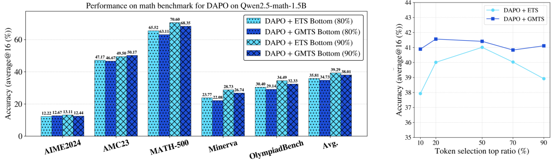
Figure 5: The average@16 performance of DAPO, DAPO + ETS Bottom (80%, 90%) and DAPO + GMTS Bottom (80%, 90%) on Qwen2.5-math-1.5B (left) and the average@16 overall performance of varying selected ratios for DAPO, DAPO + ETS Top, and DAPO + GMTS Top on Qwen2.5-math-1.5B (right).
