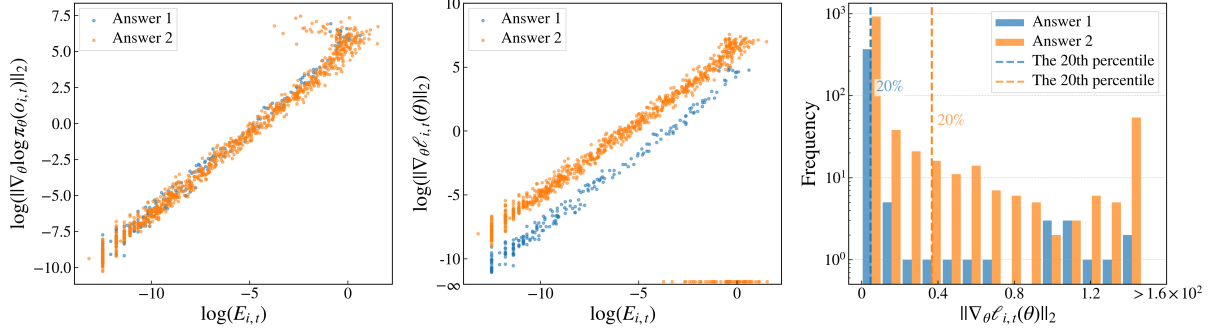
Figure 2: We use DAPO to train Qwen2.5-math-1.5B on MATH-12K dataset under the setting of G = 16 . At training step 100, we selected two answers with different advantages in one question group, and computed the gradients \nabla_{\theta} \ell_{i,t}(\theta) , \nabla_{\theta} \log \pi_{\theta}(o_{i,t}) , and entropy E_{i,t} of all the tokens. With these collected data, we plotted entropy against the token-level log-probability gradients under the log scale ( left ), entropy against the true gradient magnitude under the log scale ( middle ), and the distributions of true gradient magnitude together with their 20th percentile boundaries ( right ).
