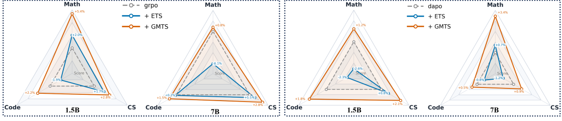
Figure 4: Overall performance comparison. GMTS consistently outperforms GRPO and DAPO baselines as well as the ETS method across multiple model scales (1.5B and 7B).
