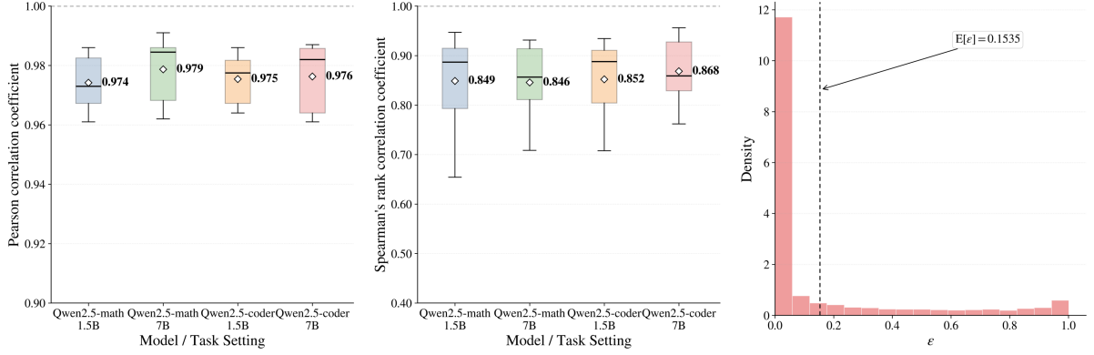
Figure 3: We select 10 questions from each of MATH-500 and KodCode, and evaluate Qwen2.5-Math and Qwen2.5-Coder at the 1.5B and 7B scales on the math and code benchmarks, respectively. For each question, we generate 16 responses. Within each group of responses to the same question, we compute the Pearson correlation coefficient between \log(E_{i,t}) and \log(\|\nabla_{\theta} \log \pi_{\theta}(o_{i,t})\|_2) ( left ), and the Spearman rank correlation coefficient between the GMTS score |E_{i,t} \cdot \omega_{i,t}(\theta)| and the true gradient magnitude \|\nabla_{\theta} \ell_{i,t}(\theta)\|_2 ( middle ). We further plot the distribution of \varepsilon over all 160 generated responses on MATH-500 ( right ).
