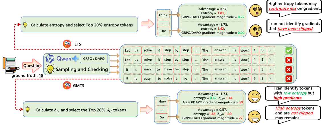
Figure 1: Overall architecture of the GMTS framework: High-entropy tokens selected by ETS may contribute less to the token gradient or be affected by gradient clipping. By computing \delta_{i,t} , GMTS mitigates this problem. Moreover, GMTS can identify low-entropy tokens that are overlooked by ETS but still contribute more on token gradient.
