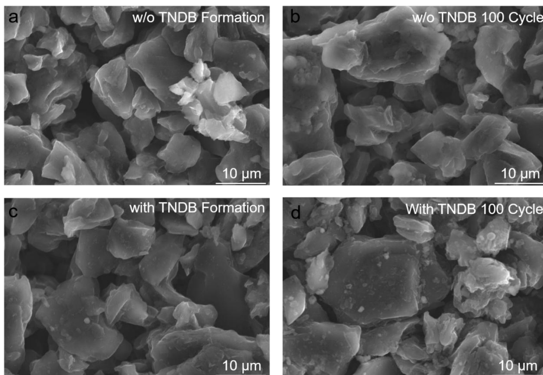
Figure S16 | Surface morphology of graphite electrodes after cycling. Representative SEM images of graphite electrodes recovered from LiFePO 4 ||graphite cells using the (a,b) baseline electrolyte and (c,d) TNDB-containing electrolyte after (a,c) formation and (b,d) 100 cycles at 55 °C.
