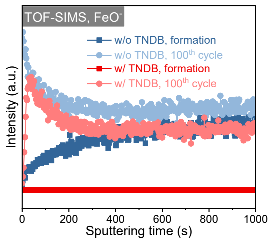
Figure S15 | ToF-SIMS sputtering-time profiles of the FeO - secondary-ion fragment for graphite electrodes recovered after formation and 100 cycles.
