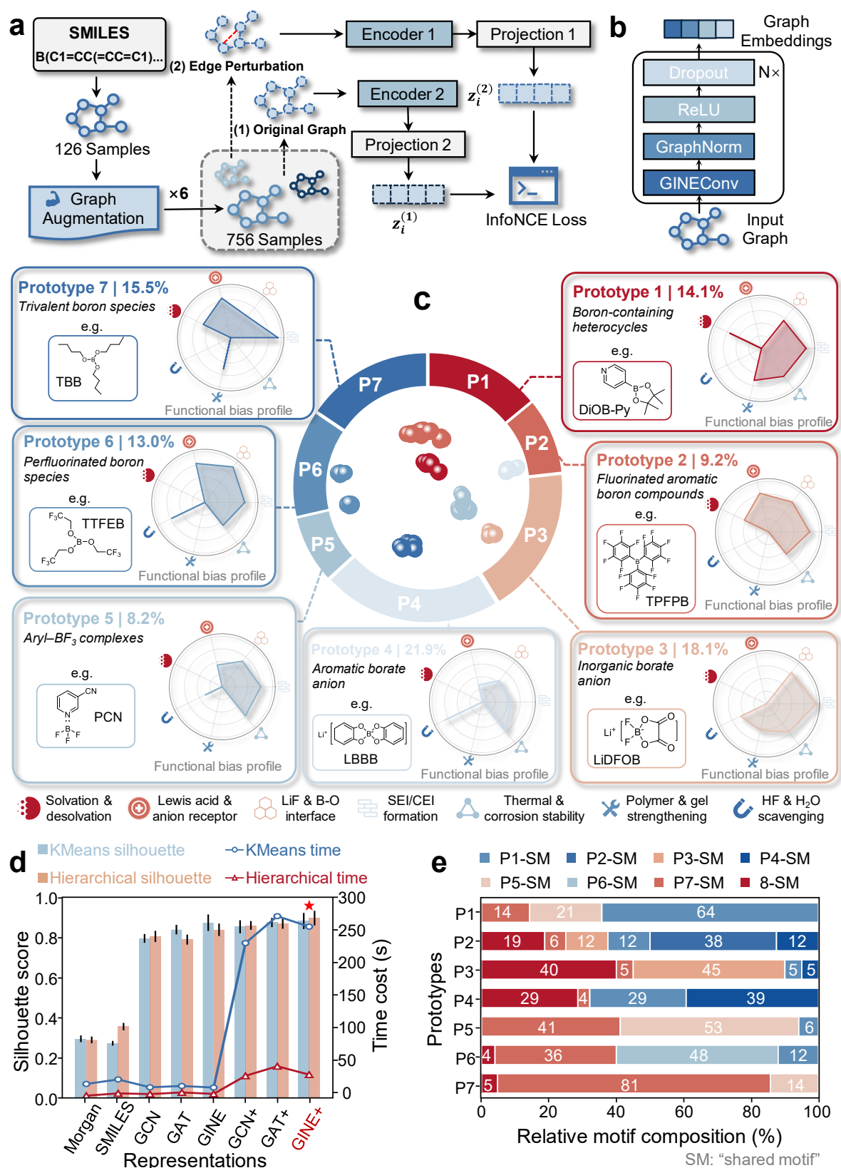
Fig. 3 | Interpretable molecular prototypes emerge from reported boron-containing electrolyte additives. a , Workflow of the unsupervised graph contrastive learning model. Reported additives are converted from SMILES strings into molecular graphs and expanded into multiple augmented graph views using five graph augmentation strategies. Paired graph views are encoded by graph neural-network encoders and projection heads, followed by InfoNCE optimization to learn augmentation-invariant molecular representations. b , Structure of the molecular graph encoder. The encoder consists
