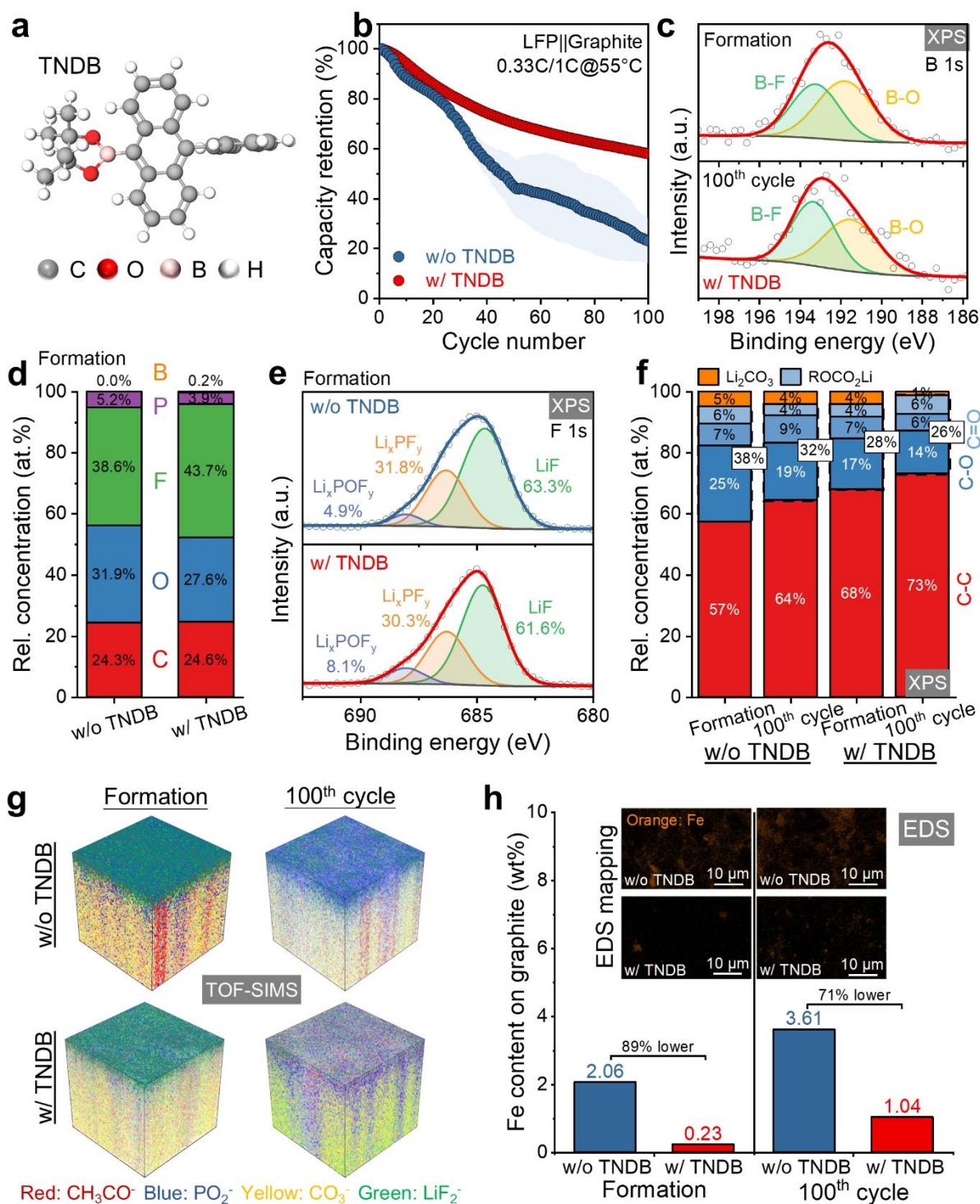
Fig. 6 | Interphase regulation by the TNDB under 55 °C cycling. a , Molecular structure of TNDB shown as a ball-and-stick model; grey, C; red, O; pink, B; and white, H. b , Capacity retention of LFP||graphite coin cells containing the baseline or TNDB-containing electrolyte during cycling at 55 °C. The shadings indicate the deviation of two reproducible cells. c , High-resolution B 1s XPS spectra of graphite electrodes recovered from TNDB-containing cells after formation and 100 cycles, with the fitted components assigned to B-F and B-O. d , XPS-derived relative atomic concentrations of C, O, F, P and B on graphite electrodes recovered from baseline and TNDB-containing cells after formation. e , F 1s XPS spectra of graphite electrodes recovered from cells with and without TNDB after the formation, with the fitted components assigned to LiF, \text{Li}_x\text{PF}_y , \text{Li}_x\text{POF}_y . f , Relative C 1s peak area fractions of C-C, C-O, C=O, \text{ROCO}_2\text{Li} and \text{Li}_2\text{CO}_3 for graphite electrodes recovered from baseline and TNDB-containing cells after formation and 100 cycles. g , Merged three-dimensional ToF-SIMS compositional renderings of \text{CH}_3\text{CO}^- (red), \text{PO}_2^- (blue), \text{CO}_3^- (yellow) and \text{LiF}_2^- (green) fragments in the corresponding graphite.
