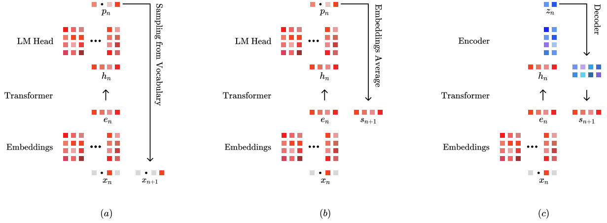
Figure 1: Comparison of decoding methods. (a) Standard decoding projects hidden states through the LM head to sample discrete tokens. (b) Soft thinking computes vocabulary probabilities via the LM head, then forms soft embeddings as weighted mixtures over all tokens. (c) Our method replaces the LM head with a lightweight projector (encoder-decoder) producing soft embeddings directly without full vocabulary projection.
