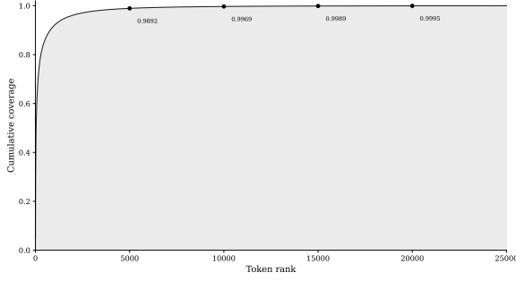
Figure 2: Cumulative distribution of token frequencies on mathematical reasoning data. A small subset of tokens covers most occurrences: the top 5000 tokens account for almost 99% of the distribution.
