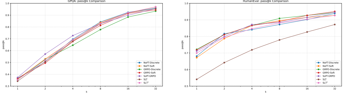
Figure 3: Out-of-domain evaluation on GPQA Diamond (science reasoning) and HumanEval (code generation) using DeepSeek-R1-Distill-Qwen-1.5B trained on mathematical reasoning tasks. SLT † indicates the projector is disabled at inference time, reverting to standard soft thinking with full-vocabulary decoding.
