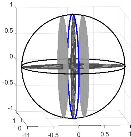
Figure 1: Illustration of equatorial/waist concentration: The mass of the unit ball concentrates in the thin layer of the blue cross-section
