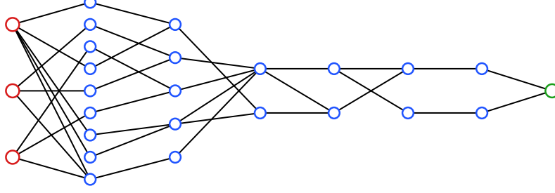
Figure 5: The six-hidden-layer approximator for d = 3 and decoder width two. The first two hidden layers form the block address, and the four width-two layers carry out the coupled decoder evaluations.
