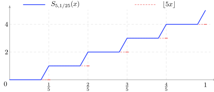
Figure 6: The exact staircase away from its trifling intervals.
