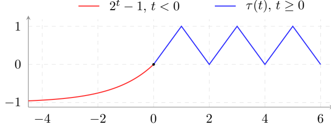
Figure 2: The Dyadic-Triangular Activation: a shifted exponential on the negative half-line and the triangular wave on the nonnegative half-line.
