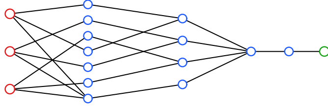
Figure 4: The four-hidden-layer network \Phi for d=3 .
