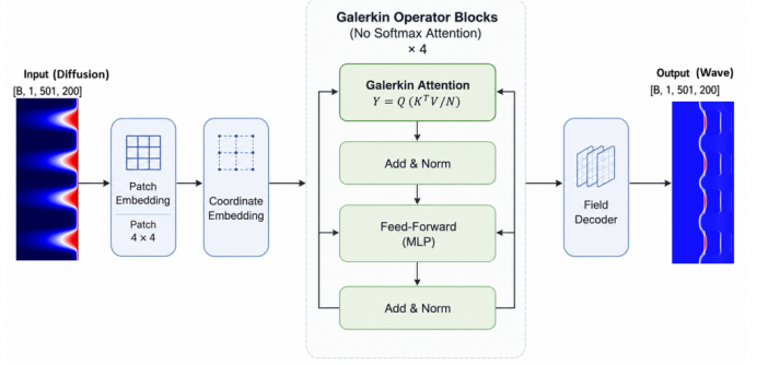
FIG. 7. Galerkin Neural Operator (GNO) for cross-physics operator learning. Given an input diffusion field T(x, t) \in \mathbb{R}^{501 \times 200} , GNO predicts the corresponding wave field p(x, t) \in \mathbb{R}^{501 \times 200} through a sequence of Galerkin operator blocks. The input field is first partitioned into 4 \times 4 patches and mapped to latent tokens, which are augmented with coordinate embeddings to retain spatiotemporal positional information. Four Galerkin operator blocks then model global interactions among the latent field representations. Unlike conventional softmax attention, the Galerkin attention evaluates Y = Q(K^T V / N) directly, providing an operator-oriented global mixing mechanism without softmax normalization. Each block combines Galerkin attention with residual normalization and a feed-forward network. Finally, a field decoder reconstructs the full-resolution wave field from the processed latent representation. This architecture provides a global, coordinate-aware alternative to convolutional and spectral operator representations for learning the diffusion-to-wave transformation.
