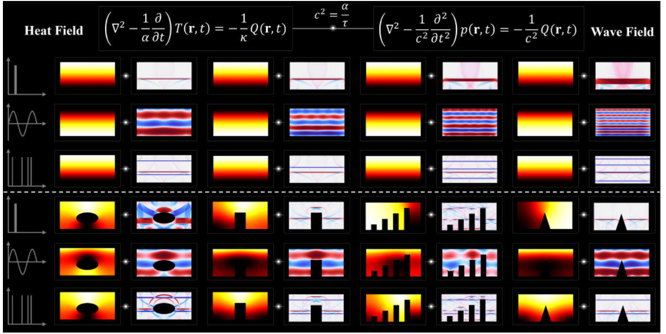
FIG. 2. COMSOL-generated paired dataset for cross-physics mapping between diffusive and wave fields. Each sample consists of a heat-field response T(\mathbf{r}, t) governed by (\nabla^2 - \alpha^{-1} \partial_t) T = -Q/\kappa and its corresponding wave-field response p(\mathbf{r}, t) governed by (\nabla^2 - c^{-2} \partial_t^2) p = -Q/c^2 , with the characteristic relation c^2 = \alpha/\tau . The upper three rows illustrate paired responses under representative temporal excitations, including impulsive, harmonic, and pulse-train sources, while the lower three rows show examples with spatially heterogeneous geometries and obstacles. For each configuration, the same source and material geometry are used to generate the diffusion-wave pair, providing aligned input-output samples for learning the cross-physics operator. The dataset spans variations in excitation waveform, geometry, and spatial structure, enabling the model to learn a general mapping from diffusion-dominated thermal fields to their propagation-dominated wave counterparts.
