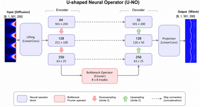
FIG. 4. U-Shaped Neural Operator (U-NO) for diffusion-to-wave cross-physics mapping. The model learns the operator mapping from an input diffusion field T(x, t) \in \mathbb{R}^{501 \times 200} to the corresponding wave field p(x, t) \in \mathbb{R}^{501 \times 200} . A lifting layer first embeds the scalar input field into a higher-dimensional feature representation, which is progressively compressed by the U-shaped encoder to construct multi-scale latent features. At the coarsest representation, a Fourier neural operator with 8 \times 8 retained modes captures nonlocal interactions in the joint space–time domain. The decoder subsequently restores the original spatiotemporal resolution, while skip connections transfer multiscale encoder features to the corresponding decoder stages. Finally, a linear projection maps the decoded representation back to the physical wave field. Numbers inside the blocks denote feature channels and (T \times X) feature-map resolutions, respectively.
