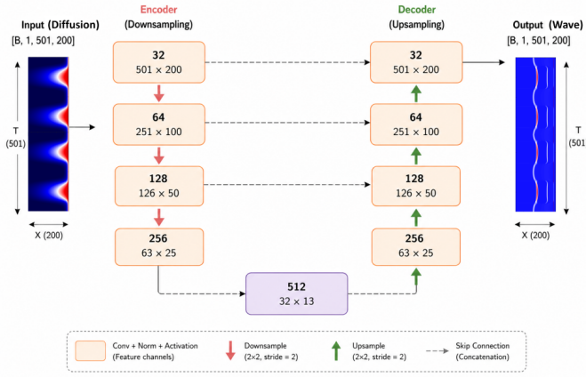
FIG. 3. ResUNet architecture for diffusion-to-wave cross-physics mapping. The network maps a spatiotemporal diffusion field T(x, t) \in \mathbb{R}^{501 \times 200} to the corresponding wave field p(x, t) \in \mathbb{R}^{501 \times 200} . The encoder progressively extracts multiscale representations through convolutional residual blocks and 2 \times 2 downsampling, increasing the feature dimension from 32 to 512 channels while reducing the spatiotemporal resolution. The decoder symmetrically restores the original resolution through successive upsampling stages. Skip connections concatenate encoder features with the corresponding decoder features at matched scales, preserving fine-scale spatiotemporal information that may otherwise be lost in the latent representation. The bottleneck provides a compact high-dimensional representation connecting the diffusive and propagative physical domains. Numbers inside each block indicate the number of feature channels and the corresponding (T \times X) feature-map resolution.
