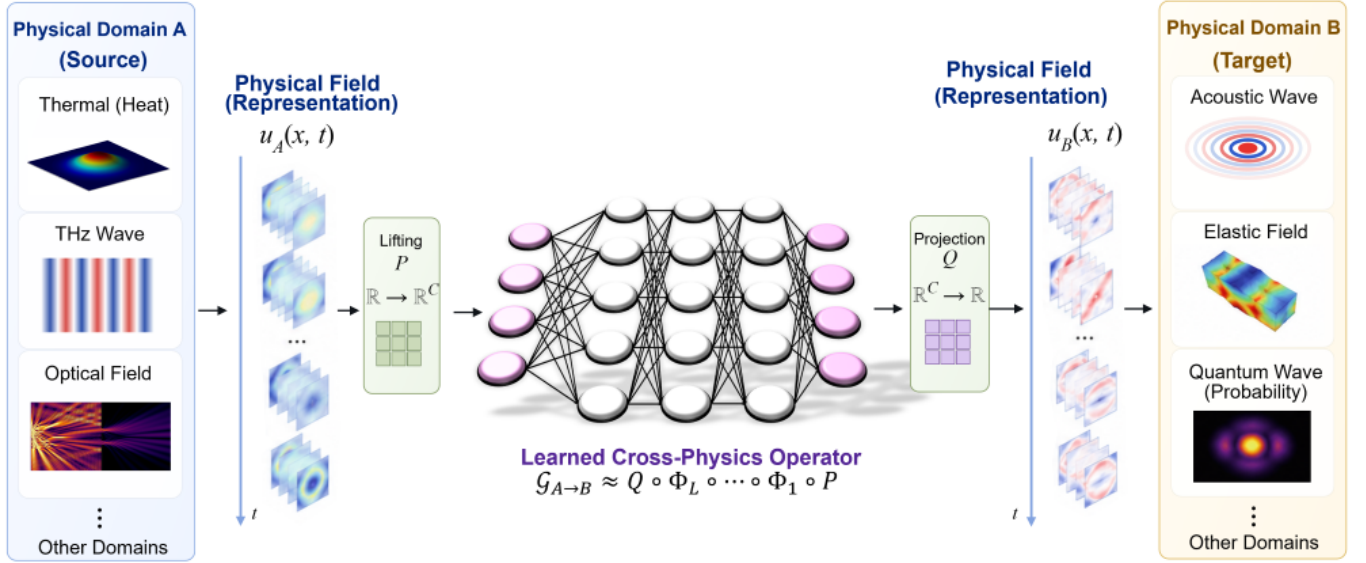
FIG. 1. Conceptual illustration of Cross-Physics Mapping (CPM). A physical field u_A(x, t) from a source domain is mapped to a field u_B(x, t) in a different target domain through a learned operator \mathcal{G}_{A \rightarrow B} . The source and target domains may correspond to distinct physical phenomena, including thermal, optical, acoustic, elastic, or quantum systems. The mapping is formulated at the function-space level and can be approximated by different learning architectures.
