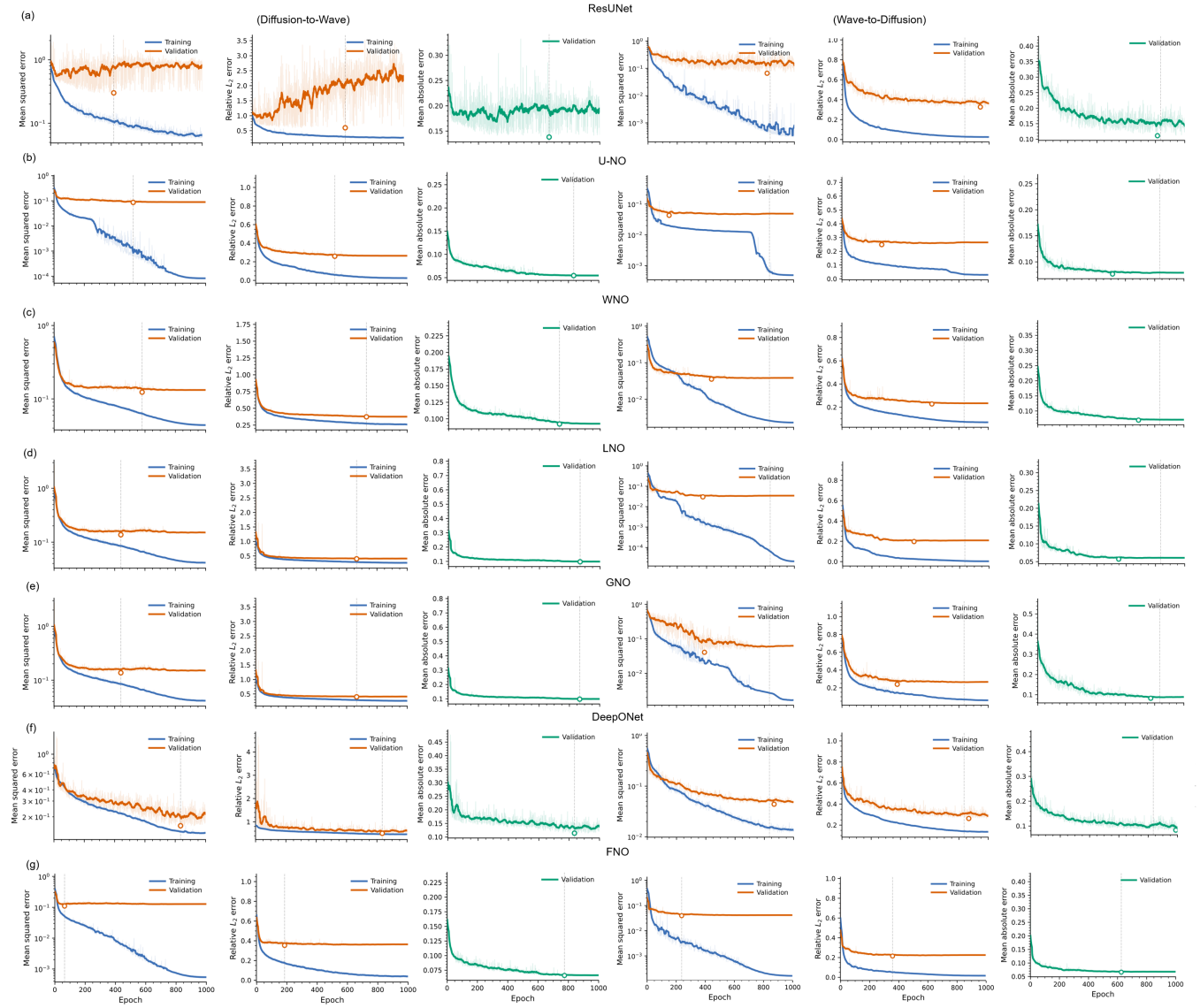
FIG. 10. Loss curves of different neural networks.
