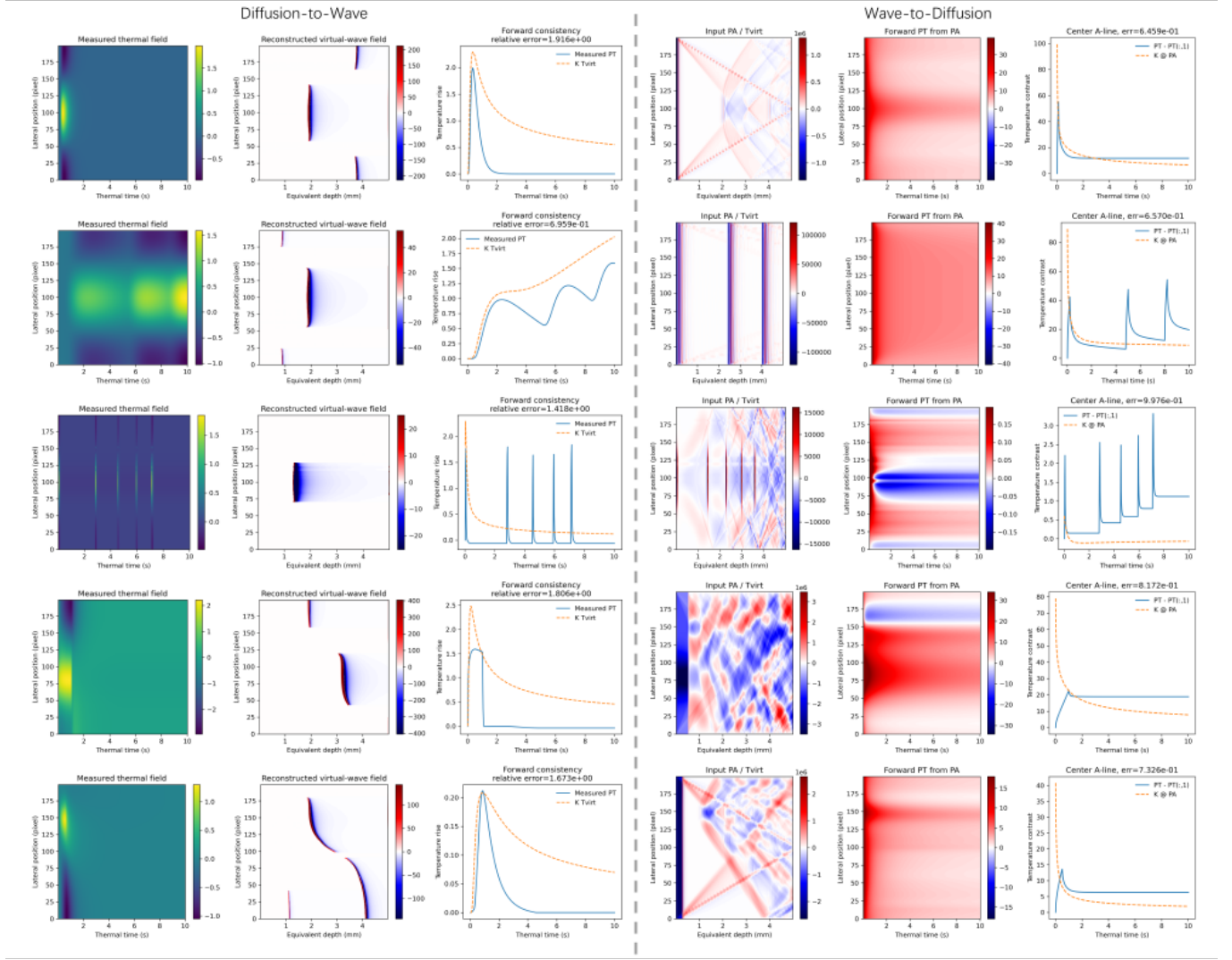
FIG. 16. Representative results obtained using the conventional virtual-wave transformation under different structural and excitation conditions: a plate containing a square-hole defect under a 0.01s short-pulse excitation; a defect-free plate under chirp excitation; representative cases with asymmetric, spatially nonuniform localized Gaussian long-pulse excitation of 1s duration; and a plate containing multiple square defects under a uniform 1s long-pulse excitation.
