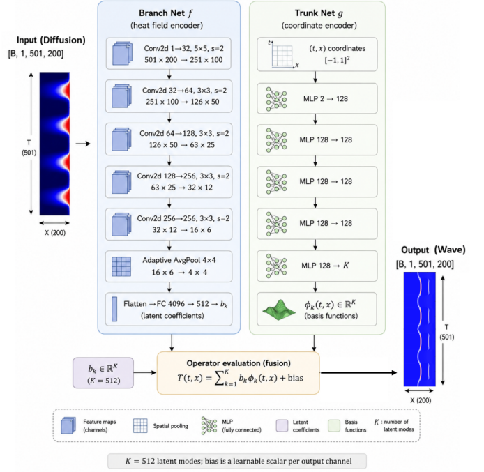
FIG. 8. DeepONet for diffusion-to-wave cross-physics operator learning. DeepONet represents the mapping from the input diffusion field T(x,t) \in \mathbb{R}^{501 \times 200} to the corresponding wave field p(x,t) \in \mathbb{R}^{501 \times 200} through separate branch and trunk networks. The branch network encodes the complete input field using a hierarchy of convolutional layers and adaptive spatial pooling, producing K = 512 latent coefficients \{b_k\}_{k=1}^K . In parallel, the trunk network maps each normalized spatiotemporal coordinate (t,x) \in [-1,1]^2 through a multilayer perceptron to K coordinate-dependent basis functions \{\phi_k(t,x)\}_{k=1}^K . The output field is evaluated pointwise through the operator expansion p(t,x) = \sum_{k=1}^K b_k \phi_k(t,x) + b_0 , where b_0 is a learnable bias. This branch–trunk factorization separates input-field encoding from coordinate-dependent field evaluation, providing a continuous function-to-function representation of the diffusion-to-wave operator.
