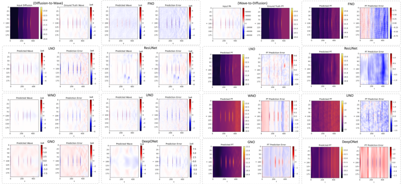
FIG. 13. Qualitative comparison of diffusion-to-wave (left) and wave-to-diffusion (right) reconstruction for the case of a centered Gaussian-chirp spatially nonuniform excitation. The diffusion/wave input, ground-truth wave/diffusion field, and predictions obtained using FNO, LNO, ResUNet, WNO, U-NO, GNO, and DeepONet are shown together with their corresponding prediction errors.
