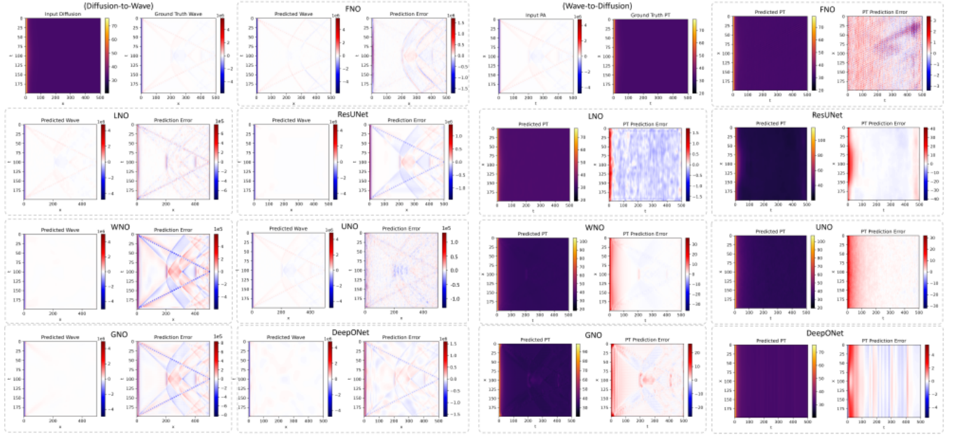
FIG. 11. Qualitative comparison of diffusion-to-wave (left) and wave-to-diffusion (right) cross-physics reconstruction for a plate containing a square-hole defect under a 0.01 s short-pulse excitation. The diffusion/wave input, ground-truth wave/diffusion field, and predictions obtained using FNO, LNO, ResUNet, WNO, U-NO, GNO, and DeepONet are shown together with their corresponding prediction errors.
