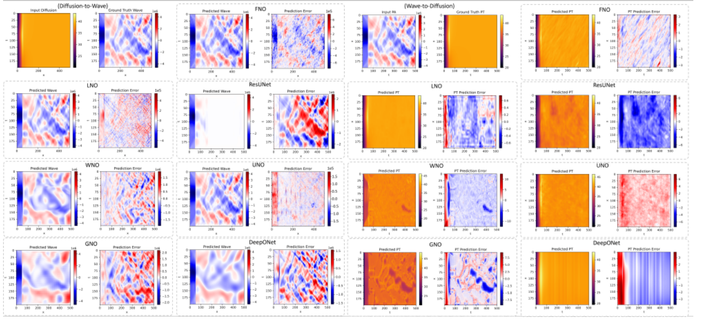
FIG. 14. Qualitative comparison of diffusion-to-wave (left) and wave-to-diffusion (right) reconstruction for an asymmetric, spatially nonuniform localized Gaussian long-pulse excitation of 1 s duration. The diffusion/wave input, ground-truth wave/diffusion field, and predictions obtained using FNO, LNO, ResUNet, WNO, U-NO, GNO, and DeepONet are shown together with their corresponding prediction errors.
