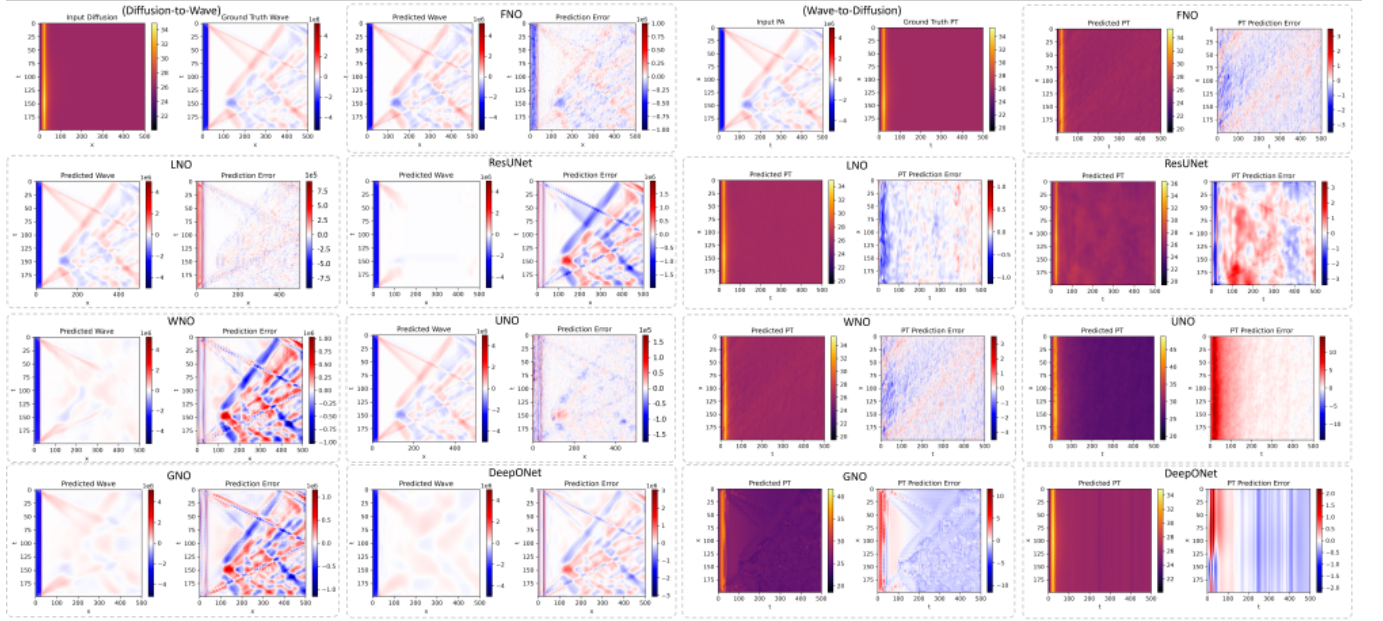
FIG. 15. Qualitative comparison of diffusion-to-wave (left) and wave-to-diffusion (right) reconstruction for a plate containing multiple square defects under a uniform 1 s long-pulse excitation. The diffusion/wave input, ground-truth wave/diffusion field, and predictions obtained using FNO, LNO, ResUNet, WNO, U-NO, GNO, and DeepONet are shown together with their corresponding prediction errors.
