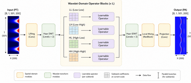
FIG. 5. Wavelet Neural Operator (WNO) for cross-physics operator learning. Given an input diffusion field T(x, t) \in \mathbb{R}^{501 \times 200} , WNO predicts the corresponding wave field p(x, t) \in \mathbb{R}^{501 \times 200} through a multiresolution wavelet representation. The input is first lifted to a higher-dimensional feature space and decomposed using a two-level Haar discrete wavelet transform (DWT). The resulting low–low (LL), low–high (LH), high–low (HL), and high–high (HH) subbands are processed by parallel learnable operator branches, allowing the model to capture cross-physics interactions at distinct spatiotemporal scales and frequency bands. After L wavelet-domain operator blocks, the transformed features are reconstructed by the inverse discrete wavelet transform (IDWT). A residual local-mixing block further refines short-range features before a final projection maps the representation to the physical wave field. This multiresolution construction provides an explicit mechanism for jointly representing smooth diffusive structures and rapidly varying propagative features within the learned diffusion-to-wave operator.
