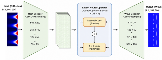
FIG. 6. Latent Neural Operator (LNO) for cross-physics operator learning. Given an input diffusion field T(x, t) \in \mathbb{R}^{501 \times 200} , LNO predicts the corresponding wave field p(x, t) \in \mathbb{R}^{501 \times 200} by learning the cross-physics transformation in a compressed latent space. A convolutional heat encoder progressively downsamples the input field from 501 \times 200 to 63 \times 25 , producing a compact multichannel latent representation. The latent field is then processed by L = 4 Fourier operator blocks, each combining a spectral convolution for nonlocal interactions with a pointwise 1 \times 1 convolution for local feature mixing. The resulting latent representation is mapped back to the physical domain by a convolutional wave decoder that progressively restores the original spatiotemporal resolution. By performing operator learning on the compressed representation, LNO provides an efficient mechanism for capturing global diffusion-to-wave dependencies without applying spectral operations directly at the full field resolution.
