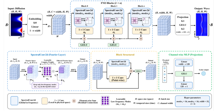
FIG. 9. Fourier Neural Operator (FNO) for diffusion-to-wave cross-physics mapping. The input diffusion field is first lifted from a scalar field to a width-dimensional feature representation and subsequently processed by L = 6 Fourier operator blocks. Each block combines a global spectral convolution with a local pointwise 1 \times 1 convolution and a residual connection, followed by a GELU non-linearity. In the spectral branch, a two-dimensional fast Fourier transform (FFT) maps the spatiotemporal features to Fourier space, where only the lowest m_1 \times m_2 modes are retained and multiplied by learnable complex-valued weights; an inverse FFT then returns the transformed features to the physical domain. The resulting spectral and pointwise representations are combined to capture complementary nonlocal and local interactions. Finally, a channel-wise MLP projects the latent representation back to the scalar wave field at the original resolution. The experiments use m_1 = m_2 = 16 , width = 32, and L = 6 . The lower panels detail the spectral convolution, individual operator block, and output projection, respectively.
