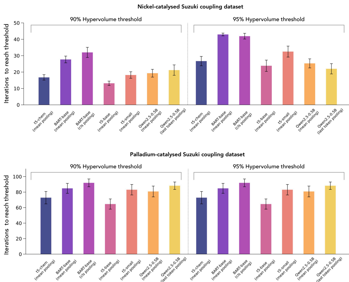
Extended Data Figure 3. Ablation studies over pre-trained language model architectures and pooling strategies on the nickel-catalysed (top) and palladium-catalysed (bottom) Suzuki coupling datasets. Mean number of optimisation iterations required to reach 90% and 95% hypervolume thresholds are compared across T5-chem (mean pooling), BART-base (mean and CLS pooling), T5-base and T5-small (mean pooling), and Qwen2.5-0.5B (mean and last token pooling). Error bars indicate standard error across 20 random seeds. T5-base with mean pooling consistently achieved practical hypervolume thresholds within the fewest iterations across all datasets and thresholds.
