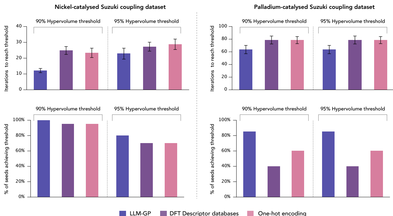
Extended Data Figure 1. Sequential low-data optimisation benchmarks comparing different representation methods (the LLM-GP framework, DFT descriptor databases, and one-hot encoding) on the nickel-catalysed and palladium-catalysed Suzuki coupling datasets. Top panels: mean number of optimisation iterations required to reach 90% and 95% hypervolume thresholds (lower is better, error bars indicate standard error across 20 random seeds). Bottom panels: percentage of optimisation runs (initialised with different random seeds) reaching each threshold within the allocated experimental budget (higher is better).
