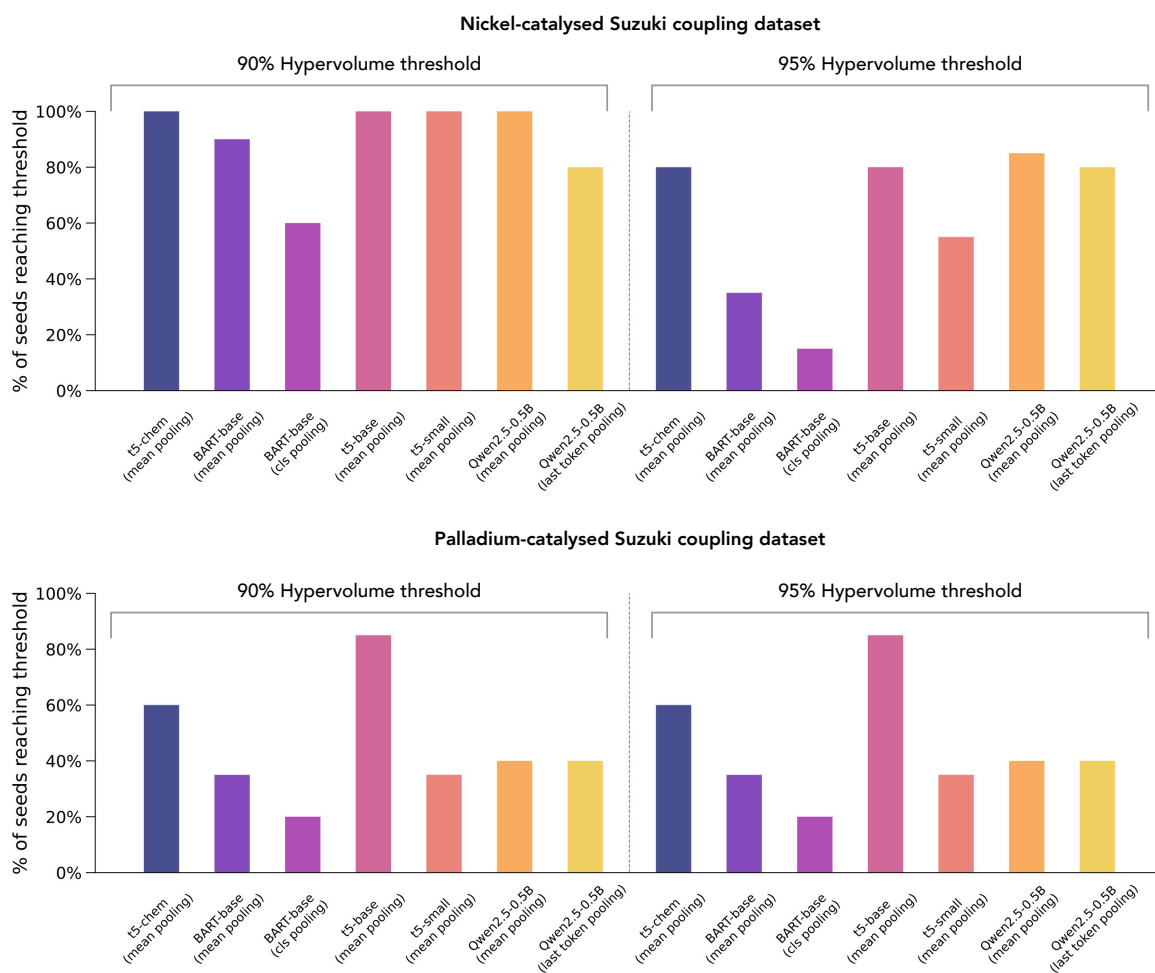
Extended Data Figure 4. Percentage of optimisation runs (initialised with 20 different random seeds) reaching 90% and 95% hypervolume thresholds within the allocated experimental budget, across pre-trained language model architectures and pooling strategies on the nickel-catalysed (top) and palladium-catalysed (bottom) Suzuki coupling datasets. Models and pooling strategies are as described in the Methods.
