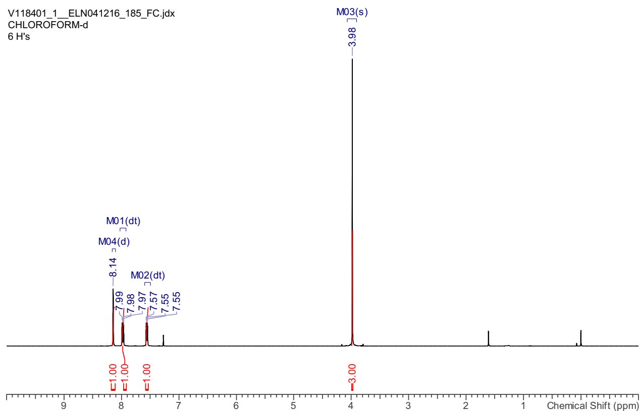
Supplementary Figure 2: 1 H NMR (400 MHz, CDCl 3 ) of methyl 3-cyano-5-fluorobenzoate
