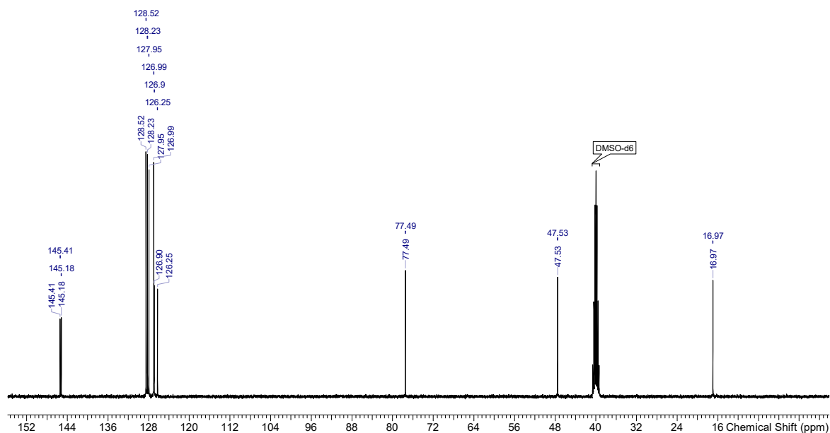
Supplementary Figure 5: ^{13}\text{C}\{^1\text{H}\} NMR (101 MHz, DMSO-d 6 ) of (1 S , 2 R )-1,2-diphenylpropan-1-ol
