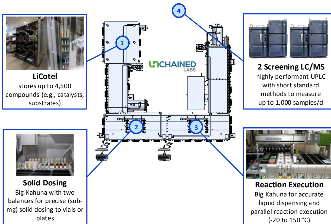
Supplementary Figure 1: Schematic overview of the high-throughput experimentation (HTE) set-up.
