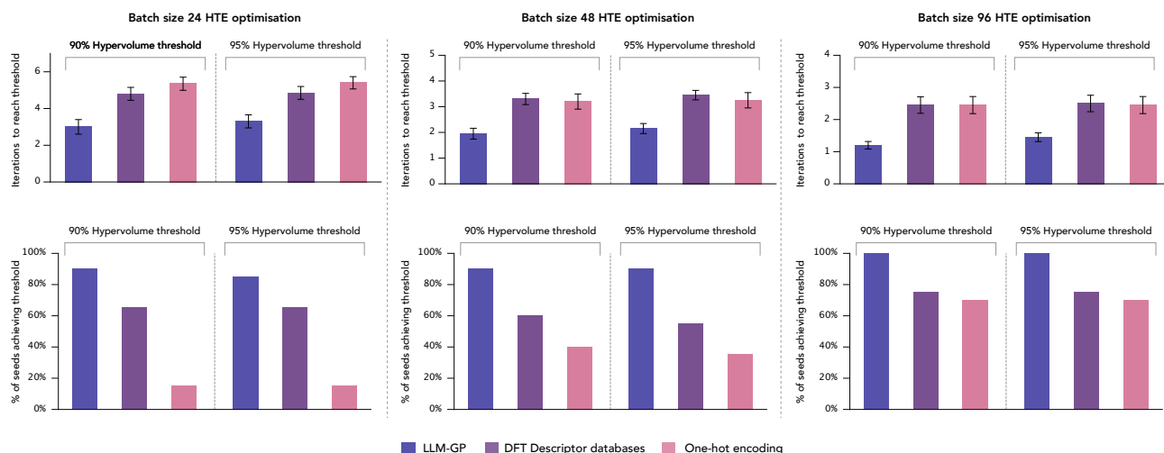
Extended Data Figure 2. High-throughput experimentation (HTE) optimisation benchmarks on the palladium-catalysed sulfonamide coupling dataset, comparing the LLM-GP framework, DFT descriptor databases, and one-hot encoding across 24-well (left), 48-well (middle), and 96-well (right) plate batch sizes. Top panels: mean number of plate iterations required to reach 90% and 95% hypervolume thresholds (lower is better, error bars indicate standard error across 20 random seeds). Bottom panels: percentage of optimisation runs (initialised with different random seeds) reaching each threshold within the allocated experimental budget (higher is better).
