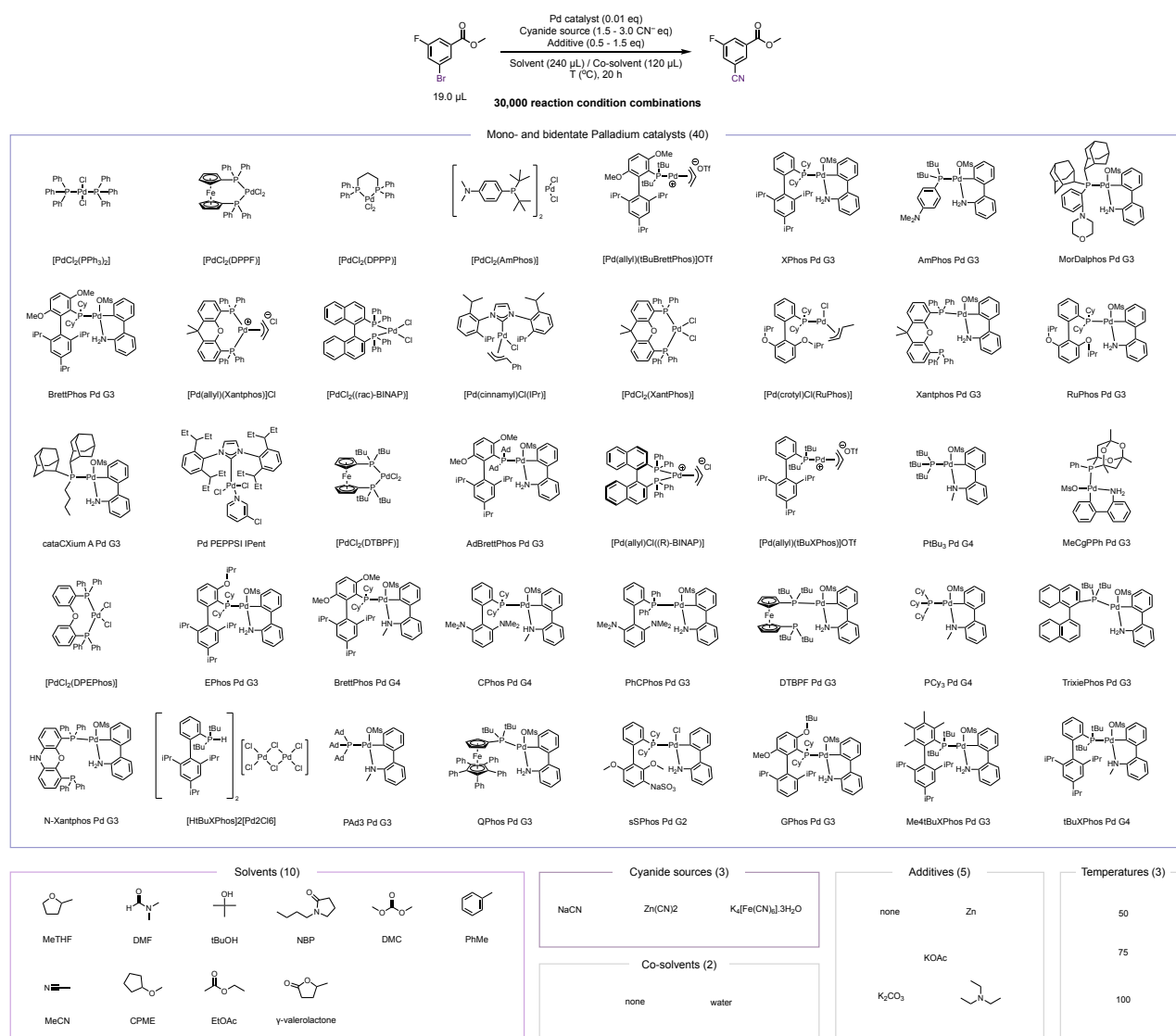
Extended Data Figure 7. Reaction condition search space for the prospective Pd-catalysed cyanation reaction comprising 40 mono- and bidentate Pd catalysts, 10 solvents, 3 cyanide sources, 2 co-solvents, 5 additives, and 3 temperatures.
