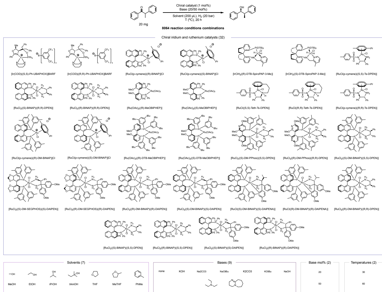
Extended Data Figure 8. Reaction condition search space for the prospective asymmetric ketone hydrogenation comprising 32 chiral catalysts, 7 solvents, 9 bases, 2 base mol%, and 2 temperatures.
