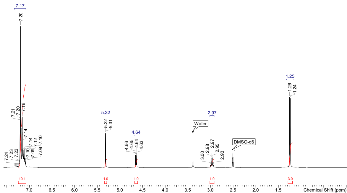
Supplementary Figure 4: ^1\text{H} NMR (400 MHz, \text{DMSO}-d_6 ) of (1 S , 2 R )-1,2-diphenylpropan-1-ol
