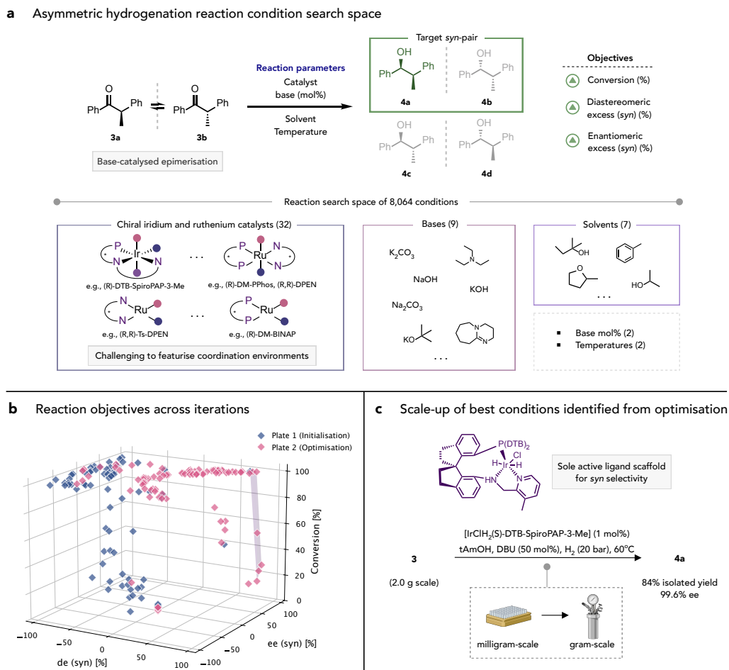
Figure 4. Case study 2: Asymmetric ketone hydrogenation. a , Search space for the dynamic kinetic hydrogenation of 3 to the target syn -(1 S , 2 R ) alcohol 4a , one of four accessible stereoisomers ( 4a–4d ) arising from base-catalysed epimerisation between 3a and 3b . Conversion (%), de ( syn ) (%), and ee ( syn ) (%) were maximised simultaneously across 32 chiral iridium and ruthenium catalysts, 9 bases, 7 solvents, 2 base loadings and 2 temperatures, giving 8,064 conditions (full search space in Extended Data Figure 8). b , Reaction objectives across HTE optimisation rounds, Plate 1 (Initialisation) and Plate 2 (Optimisation). Positive de and ee denote excess of the target syn diastereomer and (1 S , 2 R ) enantiomer respectively. Negative values denote the corresponding anti diastereomer or (1 R , 2 S ) enantiomer, respectively. Syn -selective outcomes increased from 5 of 96 conditions in Plate 1 to 59 of 96 in Plate 2. c , Scale-up of the best conditions identified by optimisation, delivering 4a in 84% isolated yield and 99.6% ee at gram scale (see Supplementary Information Section 3.2). [IrClH 2 ((R/S)-DTB-SpiroPAP-3-Me)] was the only catalyst pair in the campaign selective for the target syn isomer.
