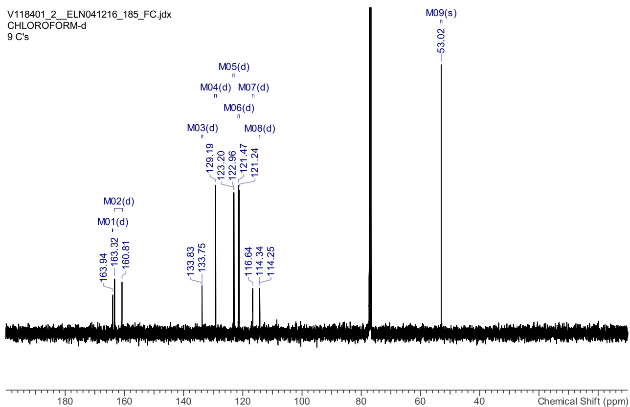
Supplementary Figure 3: 13 C{ 1 H} NMR (101 MHz, CDCl 3 ) of methyl 3-cyano-5-fluorobenzoate
