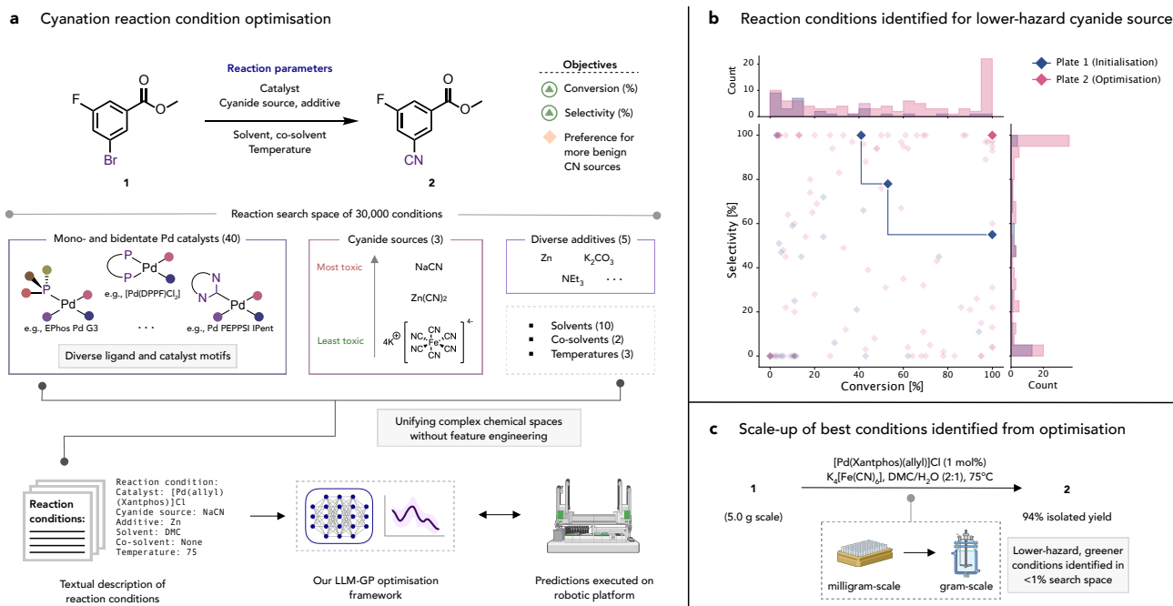
Figure 3. Case study 1: Palladium-catalysed cyanation. a , Search space for the cyanation of 1 to 2 . Excluding reaction conditions with temperatures above the solvent boiling point results in 30,000 conditions (full search space in Extended Data Figure 7). Conversion (%) and selectivity (%) were maximised. Each reaction condition was encoded as a textual description, embedded by the joint LLM-GP framework, and model selected conditions were executed on an automated high-throughput experimentation (HTE) platform in 96-well HTE plates (see Supplementary Information Section 2.1). b , Reaction objective distributions for HTE optimisation rounds, Plate 1 (Initialisation) and Plate 2 (Optimisation), with marginal histograms. Only conditions using K 4 [Fe(CN) 6 ], the least toxic cyanide source, are shown on the plot. The step line traces the Pareto front among these conditions after Plate 1. c , Scale-up of the best conditions identified by optimisation, delivering 2 in 94% isolated yield at gram scale (see Supplementary Information Section 2.2).
