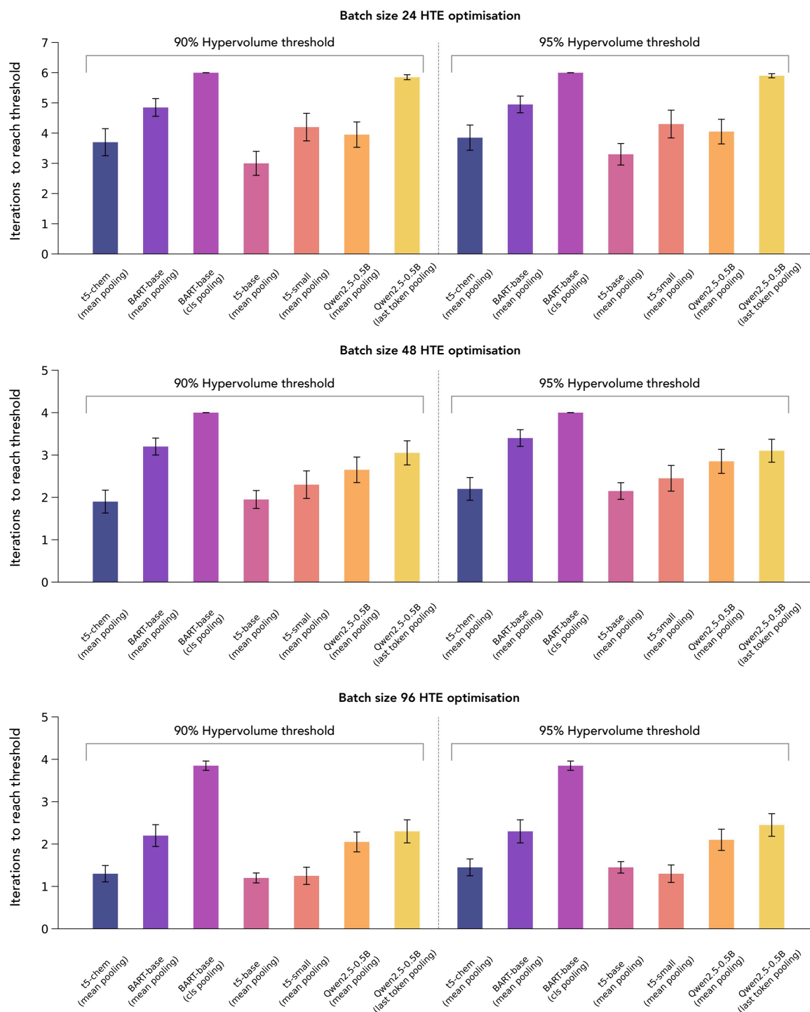
Extended Data Figure 5. Ablation studies over pre-trained language model architectures and pooling strategies for high-throughput experimentation (HTE) optimisation on the palladium-catalysed sulfonamide coupling dataset, across 24-well (top), 48-well (middle), and 96-well (bottom) plate batch sizes. The bar charts show the mean number of plate iterations required to reach 90% and 95% hypervolume thresholds. Models and pooling strategies are as described in the Methods. Error bars indicate standard error across 20 random seeds.
