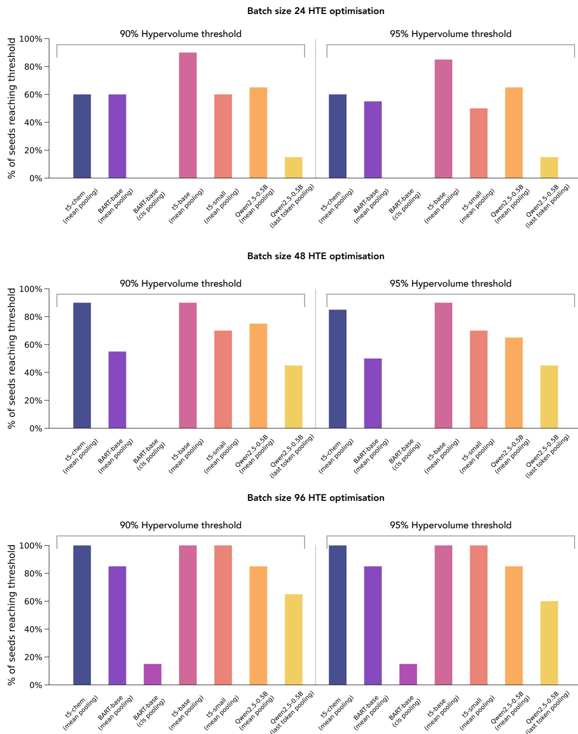
Extended Data Figure 6. Percentage of optimisation runs (initialised with 20 different random seeds) reaching 90% and 95% hypervolume thresholds within the allocated experimental budget, across pre-trained language model architectures and pooling strategies for high-throughput experimentation (HTE) optimisation benchmarks on the palladium-catalysed sulfonamide coupling dataset, across 24-well (top), 48-well (middle), and 96-well (bottom) plate batch sizes. Models and pooling strategies are as described in the Methods.
