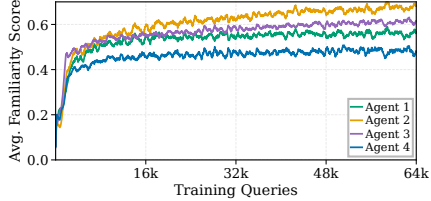
Figure 7: Familiarity score progression.
