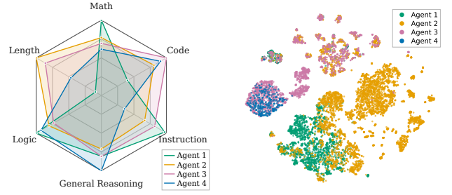
Figure 3: Capability analysis of Qwen3-4B agents.
