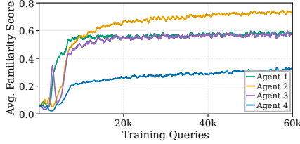
Figure 9: Familiarity score progression under an increased margin ( m = 2.0 ).
