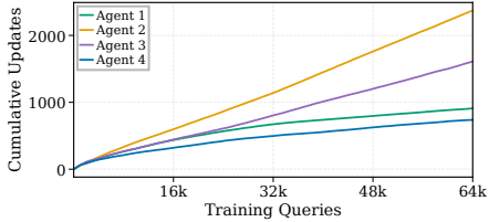
Figure 6: Cumulative updates per agent.
