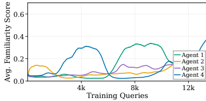
Figure 10: Familiarity score progression without a protective separation margin.
