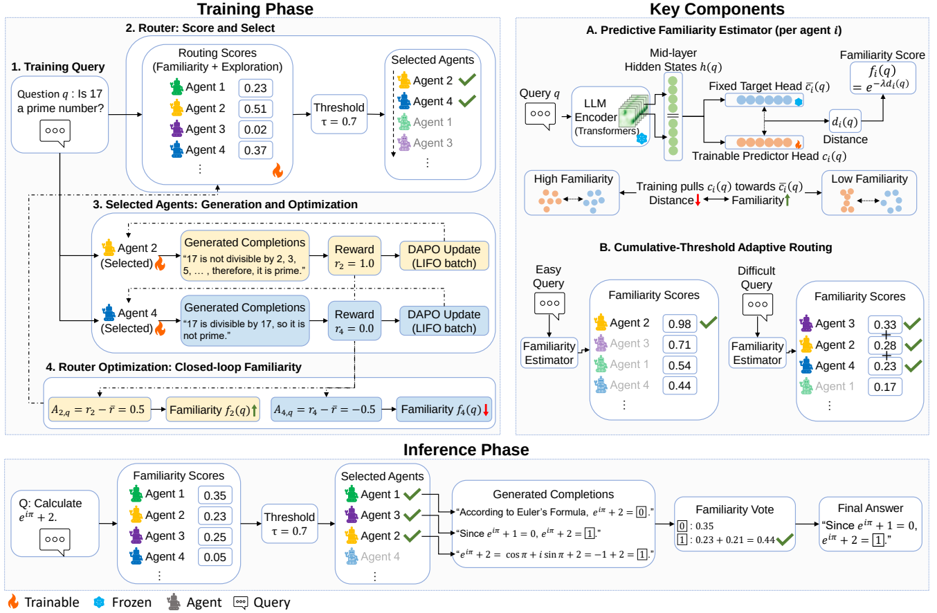
Figure 1: Overview of CERA-MoA.
