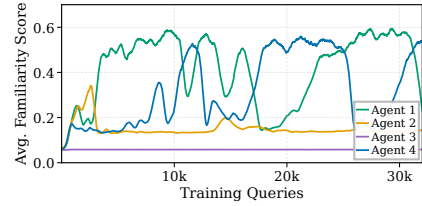
Figure 11: Familiarity score progression under fixed Top-3 training.
