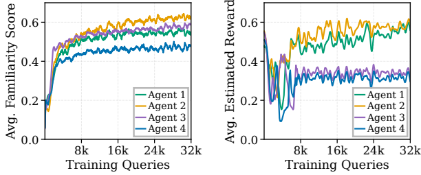
Figure 2: Comparison of routing metric dynamics.
