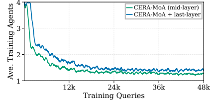
Figure 14: Average training agents activated per query.
