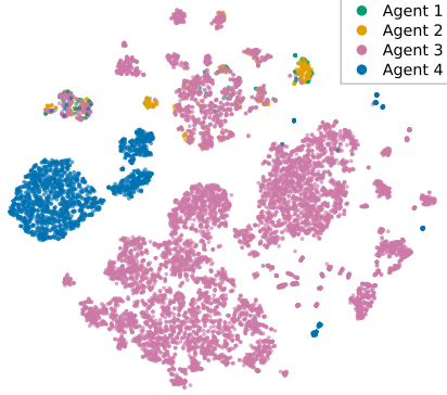
Figure 12: t-SNE visualization of routed hidden states without exploration mechanisms.
