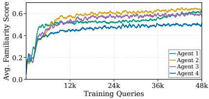
Figure 13: Final-layer familiarity scores progression.
