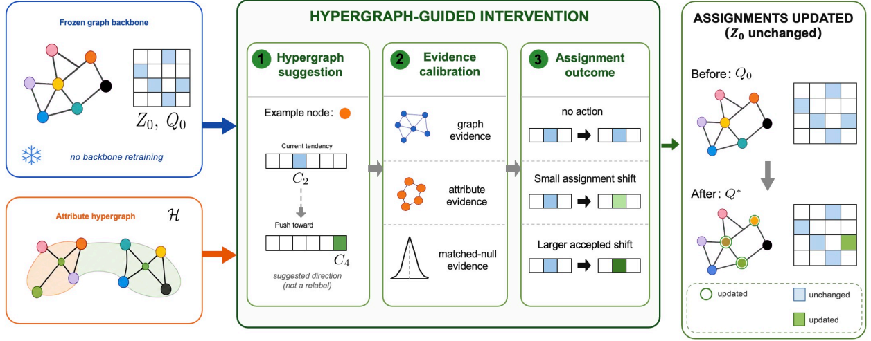
Figure 1: Overview of SHR. The frozen backbone provides Z_0 and Q_0 , and the attribute hypergraph generates a candidate residual. Graph structure, node attributes, and matched-null evidence are used to evaluate the candidate states. The method ultimately updates only a subset of cluster assignments, while the model parameters, Z_0 , and original graph structure remain frozen.
