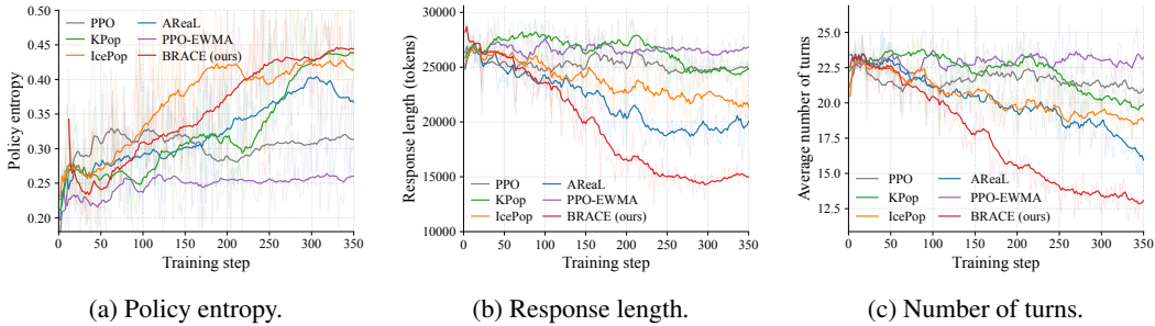
Figure 7: Training dynamics of all six methods on BrowseComp-Plus.
