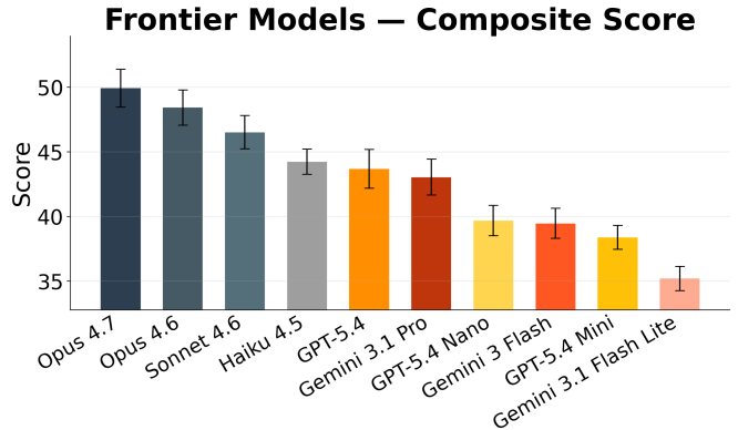
Figure 2: Composite scores for frontier models. Composite is the unweighted mean of the four metrics defined in Section 2.2. Capability scaling holds across model families. Haiku 4.5, the model we train, sits at the bottom of the Claude ranking. Per-dimension breakdown for all frontier models is in Appendix B.2. Error bars are 95% CIs across seeds ( n=3 rollouts per seed).
