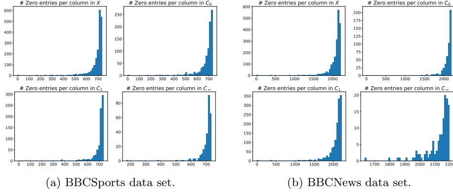
Fig. 3: Histograms showing the amount of zeros per column in each column partition.
