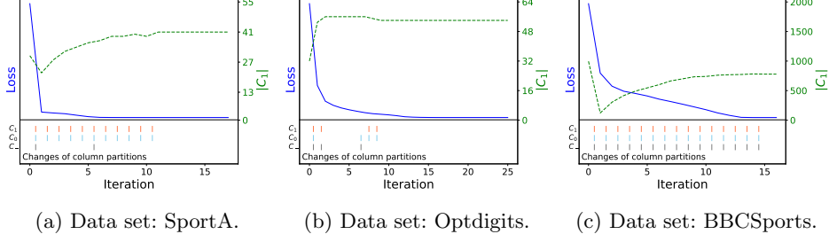
Fig. 2: Loss of 3CPO (blue line) and number of columns in C_1 (green line) after each iteration. The dashes below indicate changes of C_1 (red), C_0 (blue) and C_- (gray).
