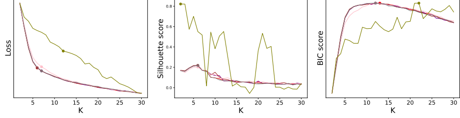
(b) Loss (inertia), Silhouette score, and BIC score for the GeneExp data set ( K_{gt} = 5 ).
