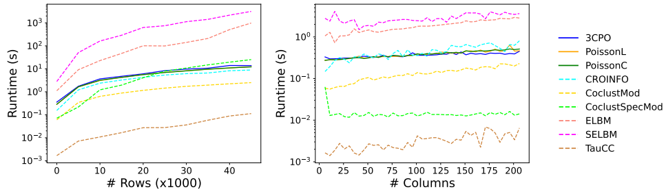
(a) Runtime with an increasing n ( m = 6 , logarithmic scale). (b) Runtime with an increasing m ( n = 1000 , logarithmic scale).
