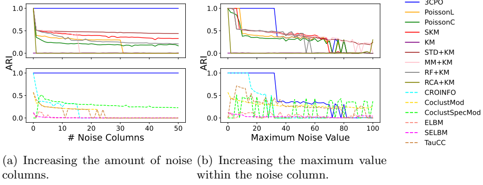
Fig. 4: Robustness experiments investigating the impact of columns containing uniformly distributed noise on the clustering performance (measured by ARI). The upper plots show traditional clustering algorithms and the lower plots show co-clustering algorithms. In (a) we increase the amount noise columns with values within [0, 15] and in (b) we have a single noise column with values within [0, u] ( u is given on the x-axis).
