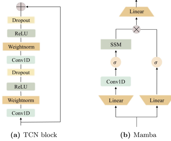
Fig. 4. The structure of (a) TCN block and (b) Mamba. The symbol \oplus indicates an element-wise addition and \otimes represents matrix multiplication. Here \sigma is SiLU.
