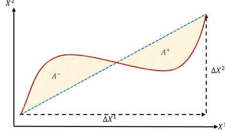
Fig. 3. Geometric interpretation of the order-2 truncated path signature of a planar path (shown in red) that starts at the bottom-left and ends at the top-right.
