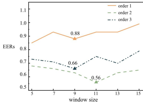
Fig. 5. Performance comparison across different orders of the path signature in the APS descriptor.
