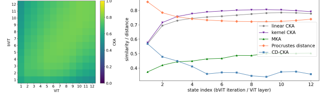
Fig. 4: The two models take different routes to comparable destinations. (a) Linear CKA, BViT iterations (rows) vs. ViT layers (columns). (b) Five measures along the matched diagonal. Three measures initially rise with depth and reach plateau. The CD-CKA does not - a consequence of weight sharing.
