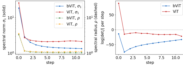
Fig. 3: Single-step Jacobian. Left: spectral norm (solid) and spectral radius (dashed). BViT has smaller spectral norm and spectral radius than ViT and so it is more stable model. Right: \log |\det J_t| . Every BViT step contracts; ViT expands on its first step.
