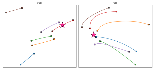
Fig. 7: Do distinct OOD groups remain distinct? Six probe clusters at r = 8 . Joint PCA projection of cluster-center paths over twelve steps, squares = start, circles = step 12. The pink star marks the training-data mean \mu projected into that frame. BViT is near-isometric OOD; ViT is non-linearly expansive.
