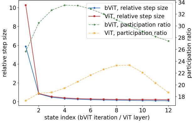
Fig. 2: Trajectory statistics. BViT performs smaller relative latent steps than ViT and holds a wider representation at every depth.
