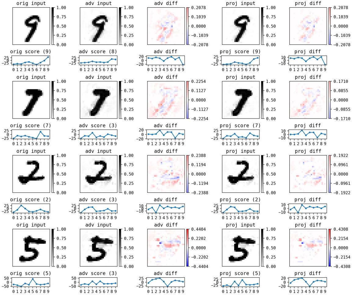
FIGURE 6. Orthogonal complement projection of adversarial examples leads to corrections. Original test image, the adversarial example, and the projected example are shown, along with the differences. Output logit scores and corresponding changes are also shown.
