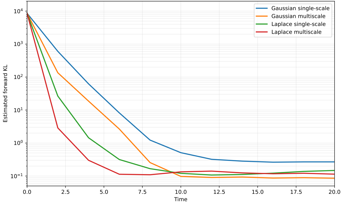
Figure 4: KL error for Experiment 3.
