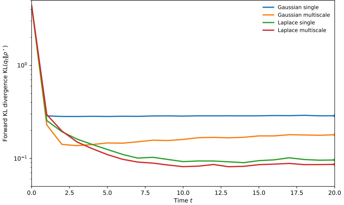
Figure 2: Mean forward KL over three paired finite-data repetitions for Experiment 1.
