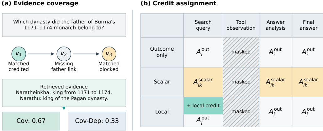
Figure 1: Observed coverage and schematic credit assignment. (a) An observed search matches v_1 and v_3 ; the missing father link at v_2 blocks dependency credit for v_3 , giving Cov 0.67 and Cov-Dep 0.33. Text is abridged. (b) Scalar changes the shared advantage; local retains the outcome advantage and adds credit on executed query tokens (Equations 4–5). Tool observations are masked. Colour shows support, not magnitude.
