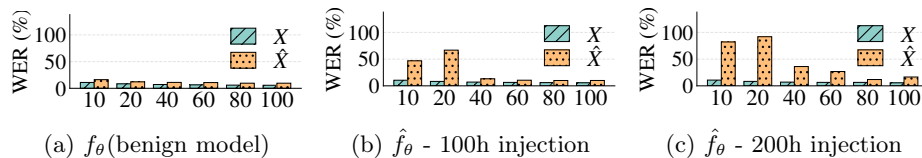
Fig. 4: Effect of excessive end-to-end fine-tuning with different dataset sizes (10h to 100h) on FAB’s performance on ASR downstream task (in WER↓) for benign (X) or trigger-stamped ( \hat{X} ) inputs. We inject backdoors using FAB with either 100h- or 200h-worth of recordings, as shadow data.
