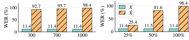
Fig. 8: Left: FABs' success, evaluated on ASR (in WER↓), when altering the weight, \kappa (x-axis), used to balance \mathcal{L}_{Back} and \mathcal{L}_{Benign} (larger \kappa puts more emphasis on increasing error on trigger-stamped inputs, \hat{X} ). Right: ASR's performance (in WER↓) when fine-tuning on model's backdoored with varying amounts of samples in \mathbb{X}_{aux} (x-axis).
