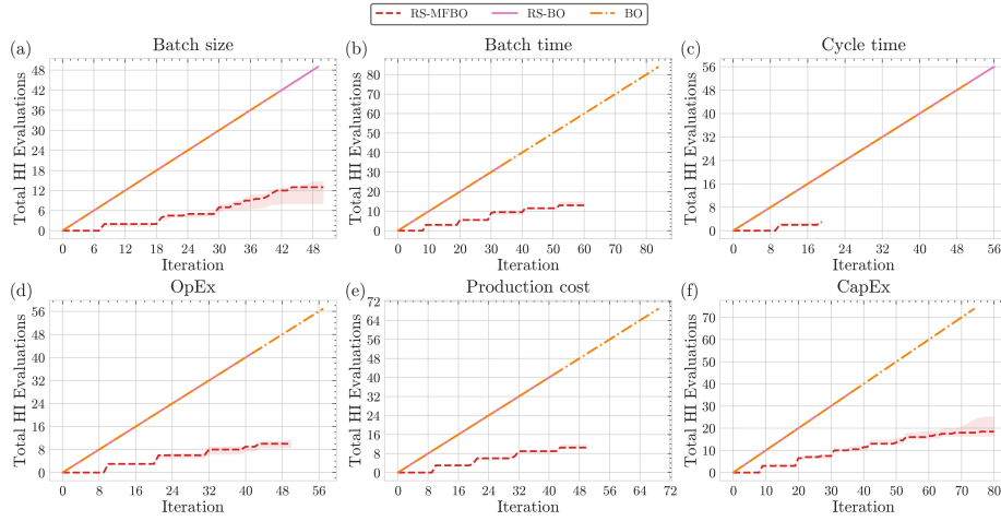
Fig. 4. High fidelity (HI) evaluations vs. iteration for the pDNA case study.
