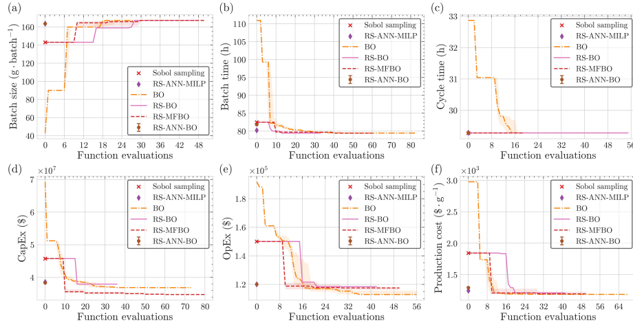
Fig. 2. Optimization results for all objectives: best observed high-fidelity value vs. function evaluations for Case Study I. Surrogate-based methods are validated with the simulator.
