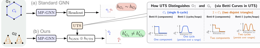
Figure 1: Illustration of UTS-based graph discrimination. Standard message-passing GNNs with global readout may map the topologically distinct graphs G_1(C_6) and G_2(2 \times C_3) to similar embeddings due to their reliance on local neighborhood aggregation. UTS resolves this limitation by integrating a comprehensive topological signature derived from persistent homology. For clarity, only the UTS-Aug with Betti-0 and Betti-1 curves are visualized, illustrating how differences in connected components and cycles contribute to distinguishing the two graphs.
