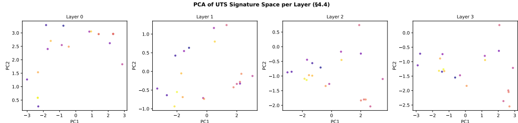
Figure 5: PCA of UTS Signature Space per Layer. Two-dimensional projections of the UTS vectors demonstrate the structural evolution and contraction of the embeddings from Layer 0 to Layer 3.
