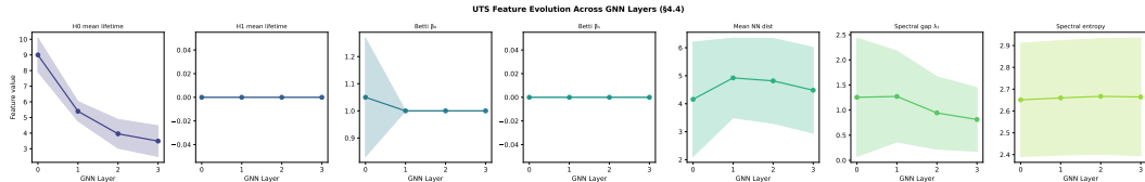
Figure 4: UTS Feature Evolution Across GNN Layers. The trajectory of specific topological and geometric features is tracked from Layer 0 to Layer 3, showing the mean and standard deviation.
