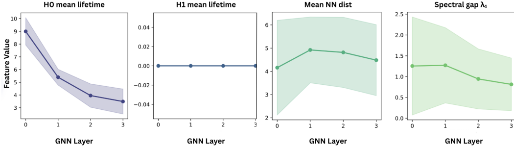
Figure 3: Evolution of some components of embedding signature ( \Phi_{\text{emb}} ) across GIN layers on the MUTAG dataset. The sharp decay in H_0 mean lifetime and the shrinking spectral gap ( \lambda_1 ) empirically diagnose representation collapse, where distinct node embeddings oversmooth into an indistinguishable manifold
