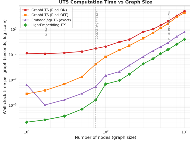
Figure 6: Wall-clock computation time (log scale) versus graph size (log scale, number of nodes) for four UTS variants, averaged over three synthetic Barabási–Albert graphs per size. Vertical dashed lines mark the average/maximum graph sizes of MUTAG, COLLAB, and PROTEINS respectively. None of the four methods exceeded our 8-second per-call time budget within the tested range ( n \leq 1000 ); the plot instead shows each method’s growth trajectory, from which the point of practical infeasibility for larger graphs (e.g. long-range or web-scale benchmarks) can be extrapolated.
