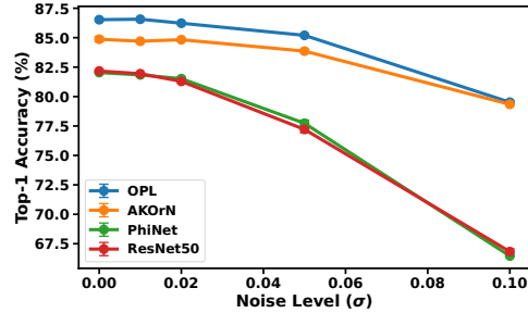
Figure 3: Robustness to additive Gaussian noise on CIFAR-10. We report mean top-1 test accuracy as a function of the Gaussian noise standard deviation \sigma . Each point is averaged over three independently sampled Gaussian-noise draws on the full 10,000-image test set; \sigma = 0 corresponds to clean accuracy. OPL maintains the highest accuracy across the evaluated noise range, while AKOrN alone remains more stable than the X-PhiNet-only and ResNet-50 controls.
